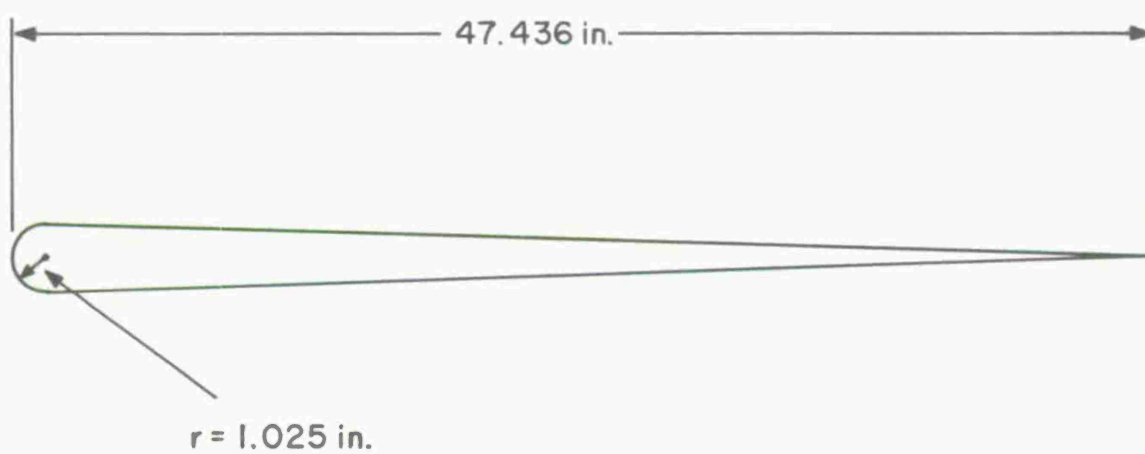
Fig. 1. Cone-Sphere.
