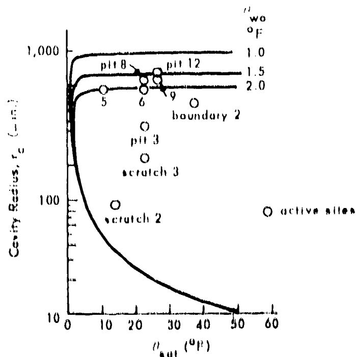
Figure 10. Size of effective cavities as function of surface-to-bulk-temperature difference, \theta_{sat} , for the boiling of ether. (From Y. Y. Hsu, 1962.)
