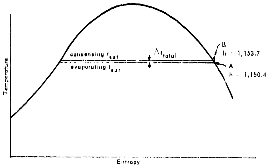
Figure 14. Possible temperature-entropy diagram and schematic of temperature drop for vapor-compression still with small temperature drop.
