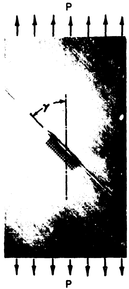
Fig. 2 SPECIMEN UNDER COMBINED TENSION AND SHEAR LOADING
