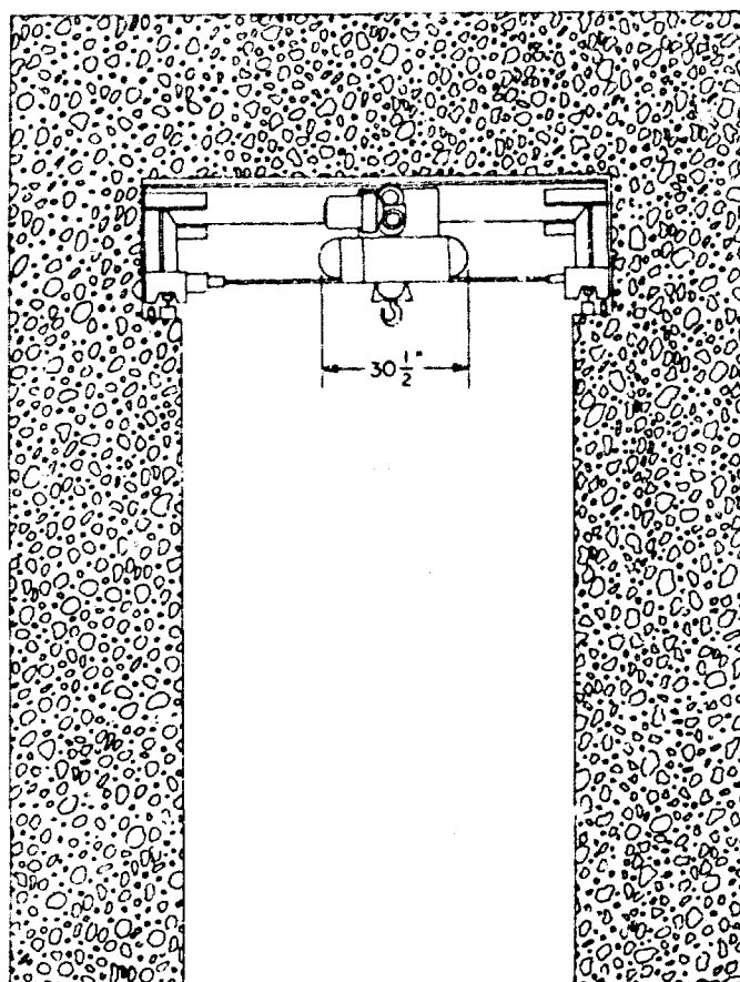
Fig. 60 - Schematic view of in-cell installation of crane hoist
