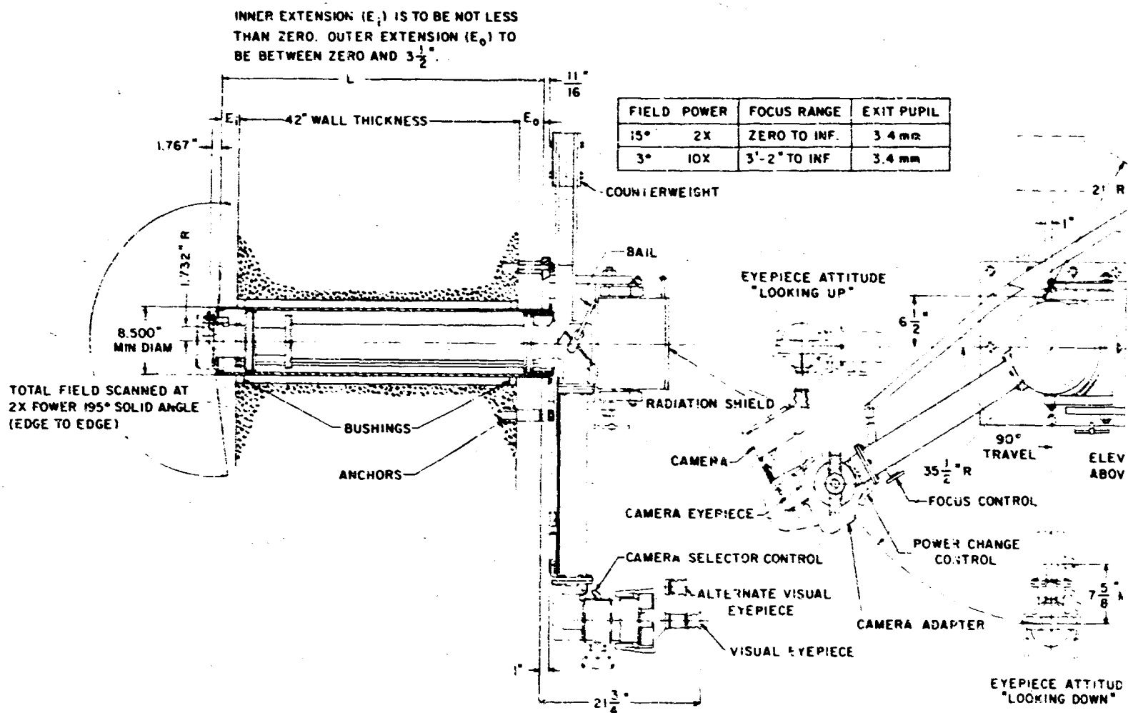
Dwg. 12. Kollmorgen wall periscope, Model 301
