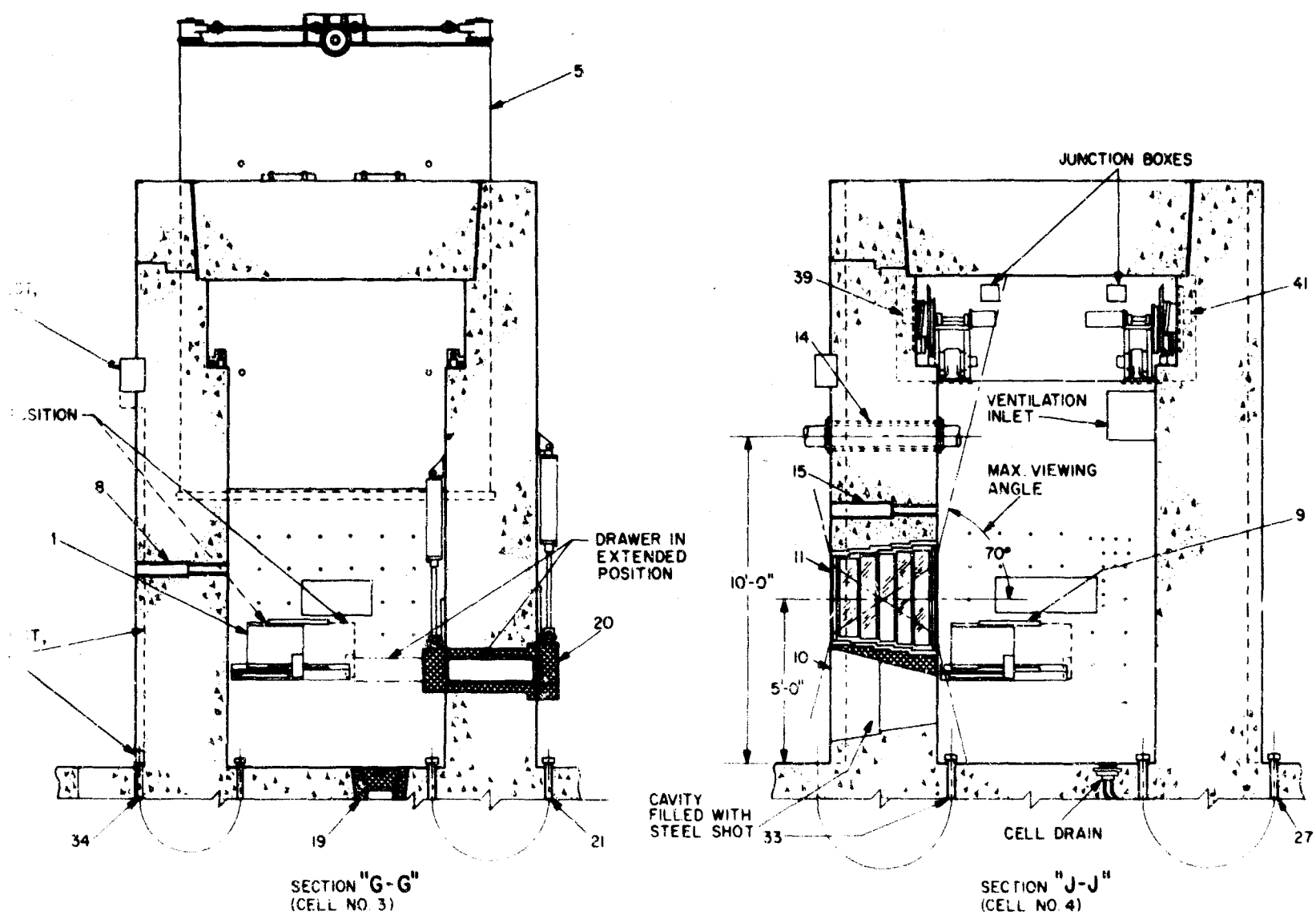
Dwg. 4. Typical elevations of hot-cell ends - sections G-G and J-J (Dwg. 2)
