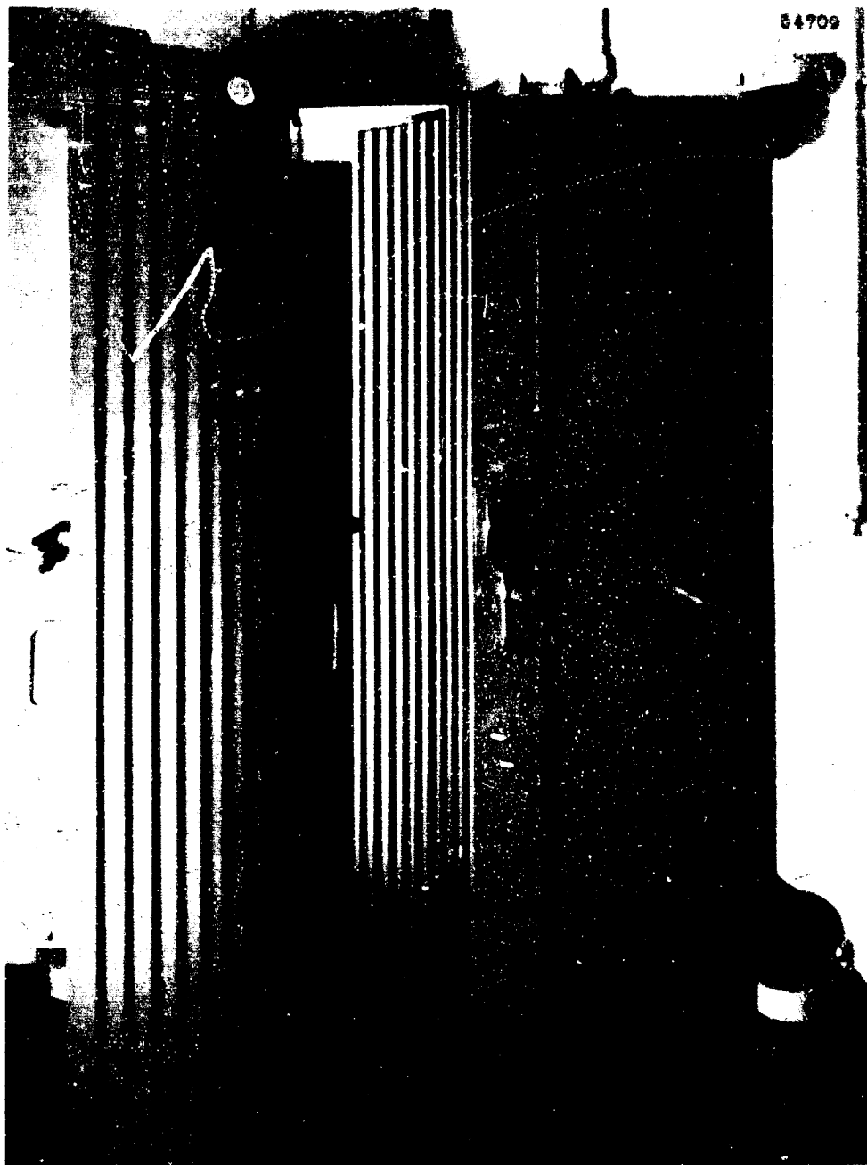
Fig. 18 - Typical construction features of steel cell shielding doors as shown by double door to cell 3
