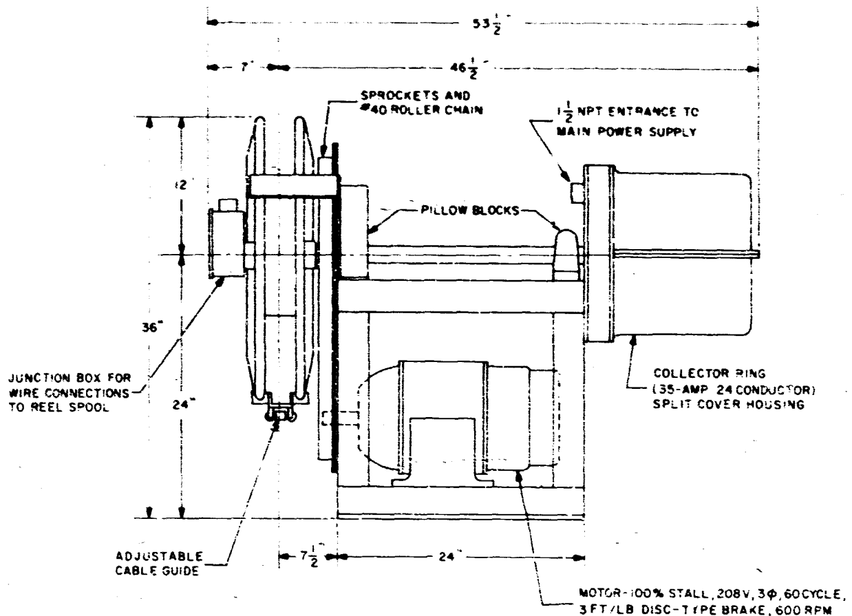
Fig. 63 - Outline of cable take-up reel (designed and mfd by Industrial Electrical Works, Inc.)
