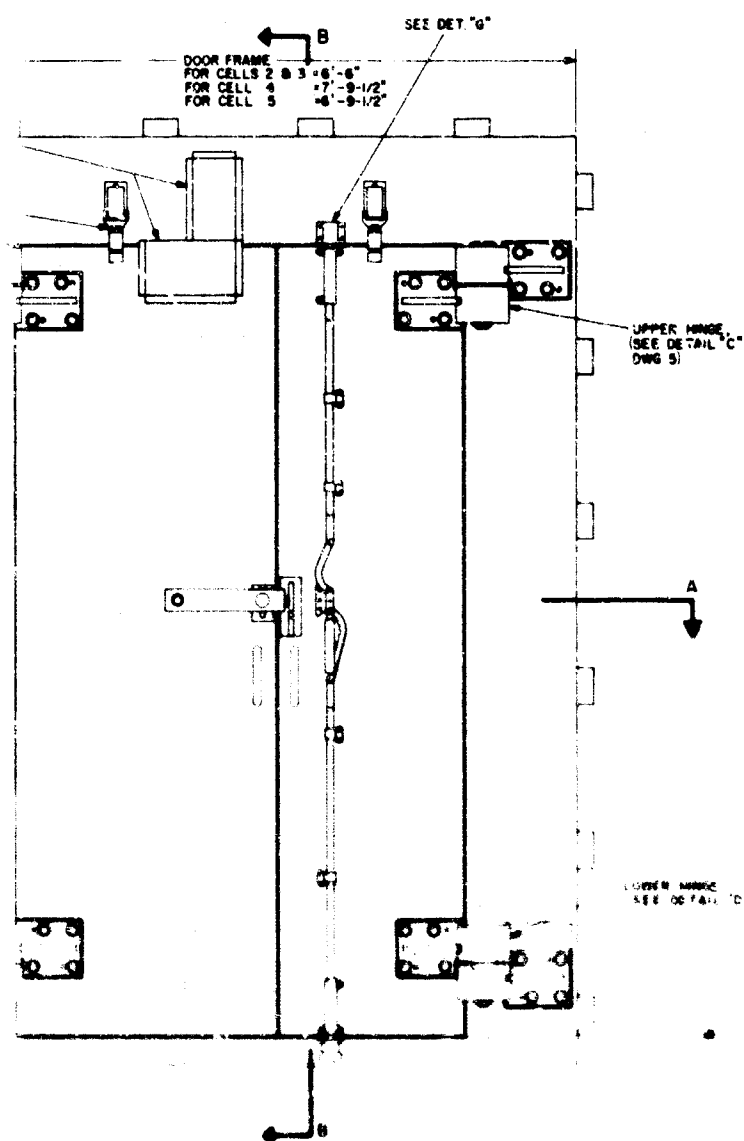
FRONT ELEVATION
