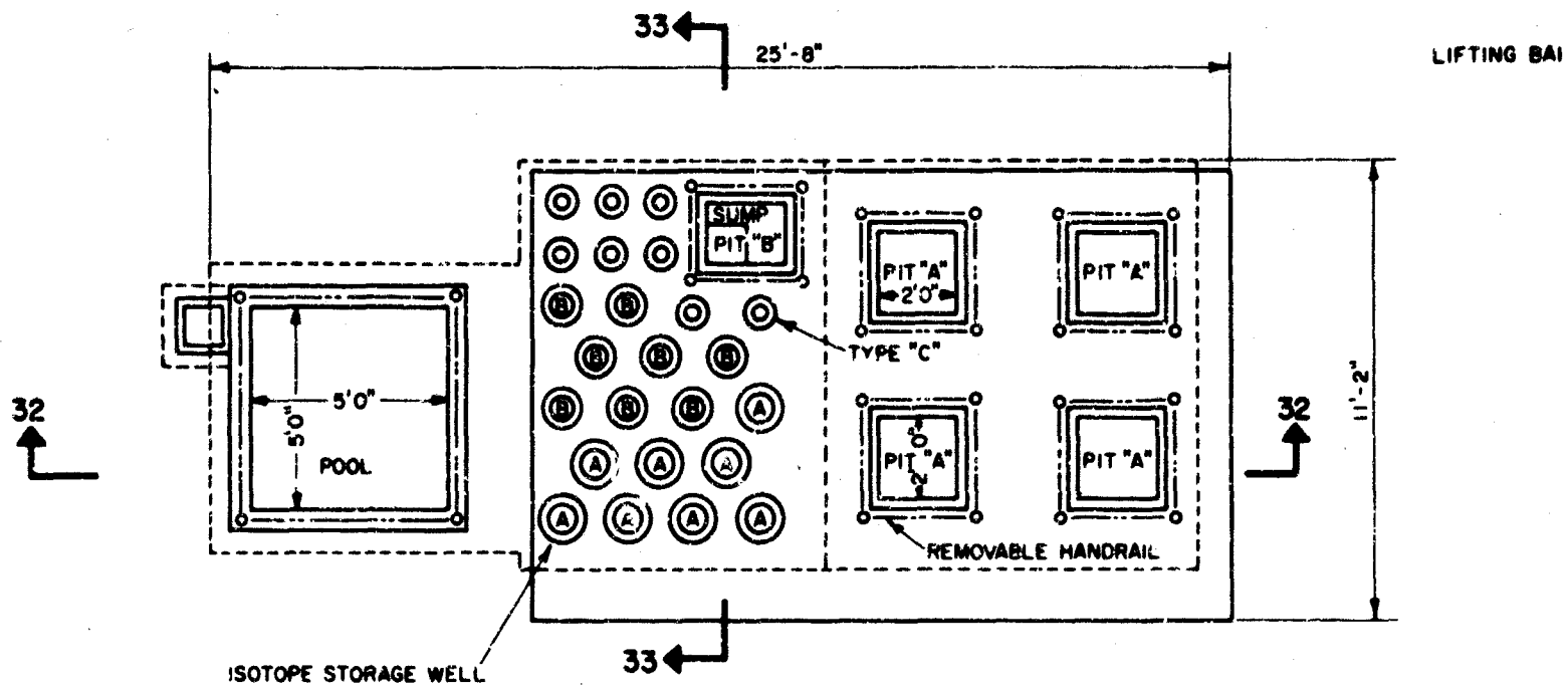
PLAN OF ISOTOPE STORAGE WELLS
