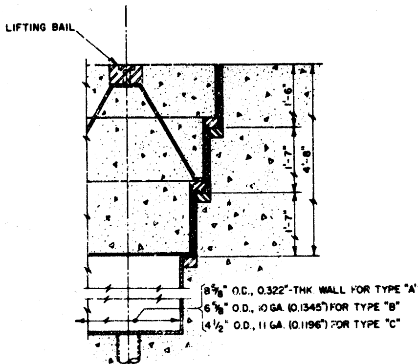
DETAIL OF ISOTOPE STORAGE WELLS (SHOWING TOP PLUG CONFIGURATION AND BOTTOM DRAIN PIPE)
