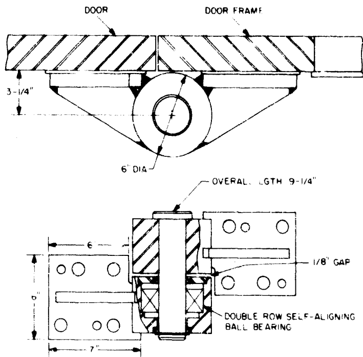
DETAIL "C" UPPER HINGE
