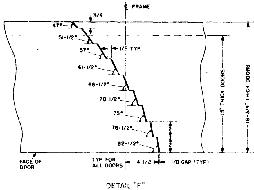
Fig. 4 - Enlarged view of double-door steps
