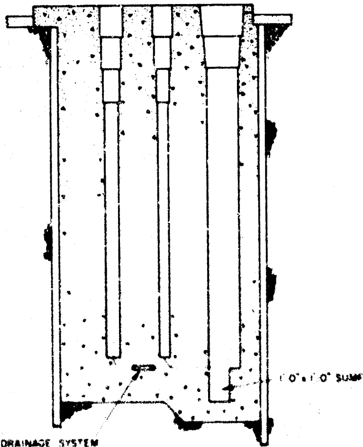
SECTION 33-33
