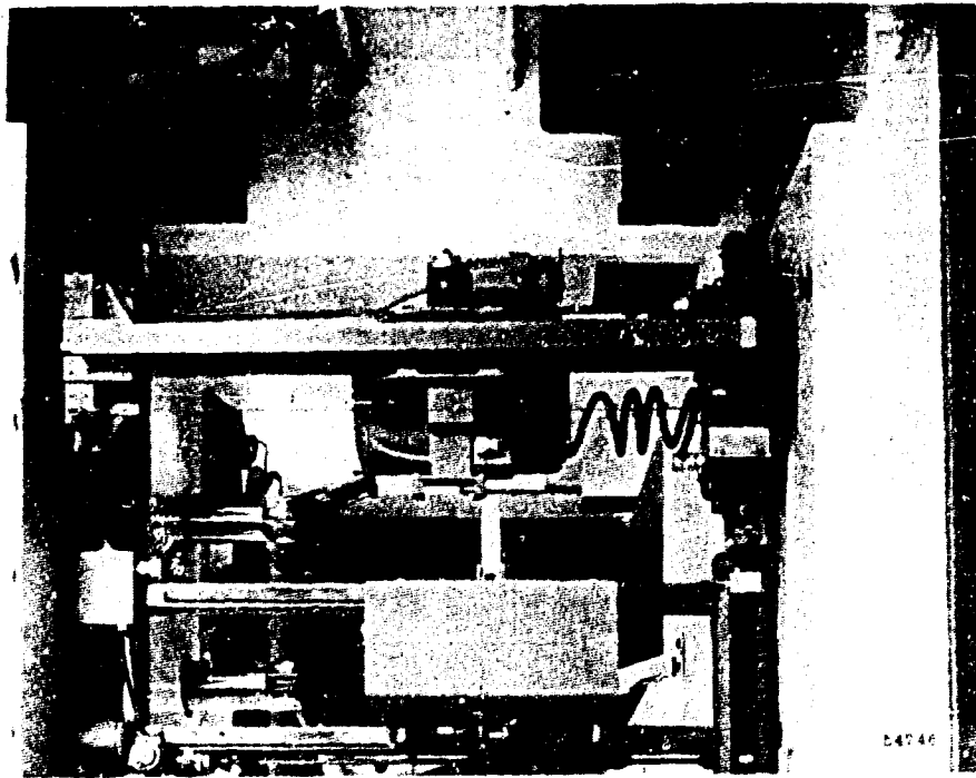
Fig. 55 - View looking down on manipulator bridge (in foreground) and arm carriage
