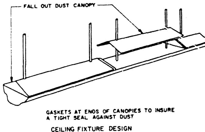
Fig. 10 - Fluorescent fixture canopy design
