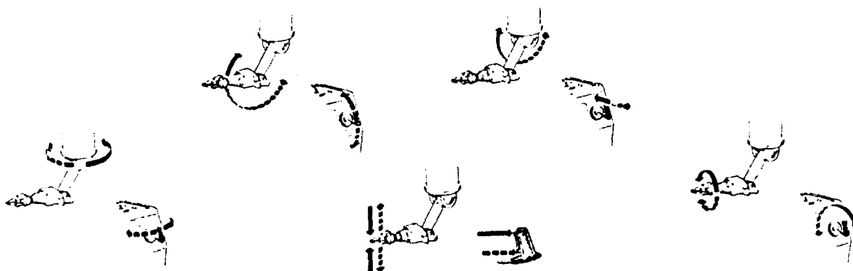
Fig. 58 - Manipulator movements vs control handle displacements
