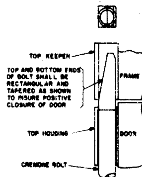
DETAIL "G"
