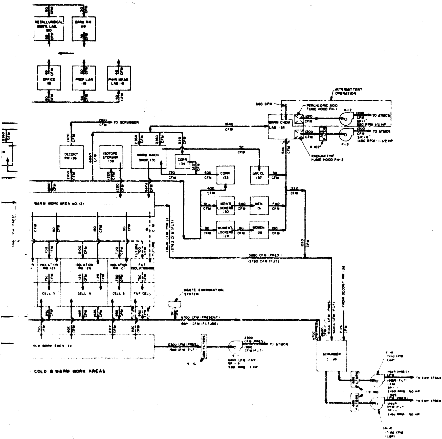
Fig. 9. Ventilation flow diagram
