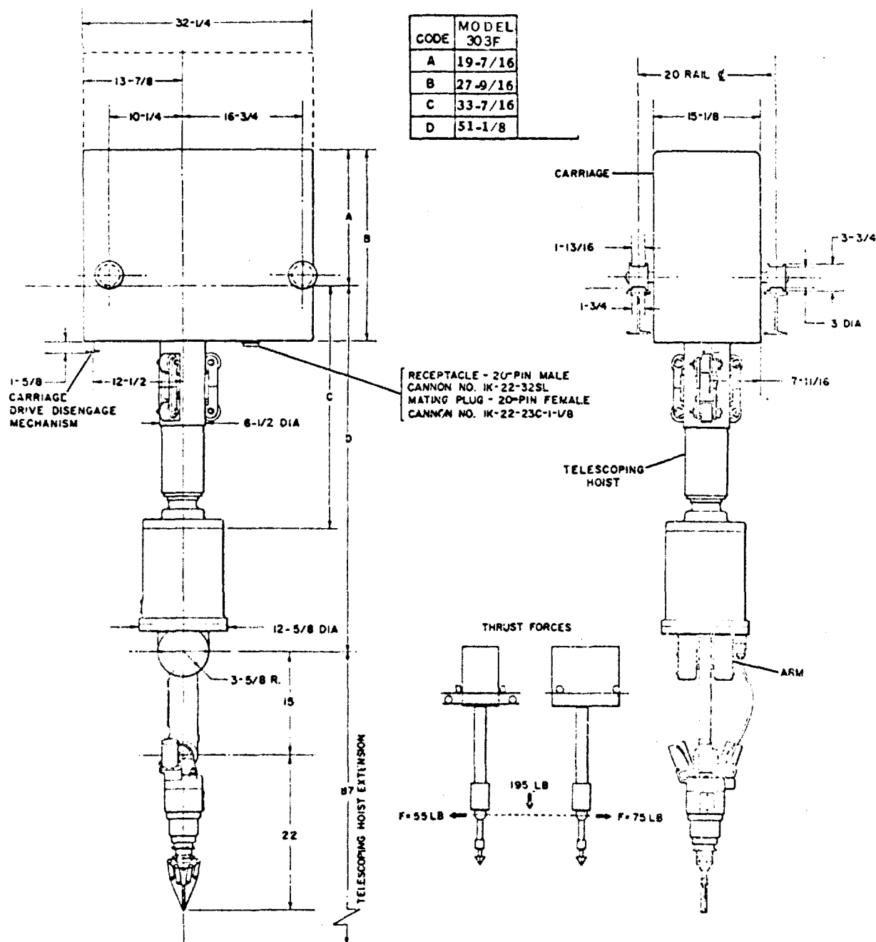
Fig. 50 - Telescoping hoist and carriage dimensions
