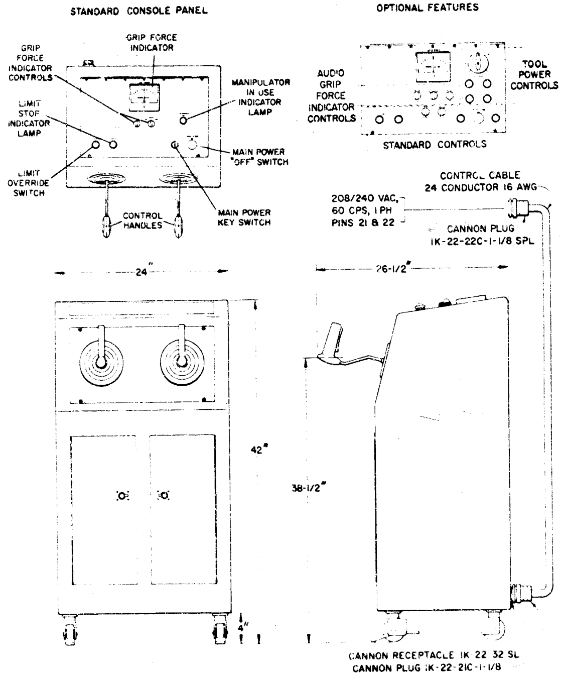
Fig. 56 - Control console dimensions
