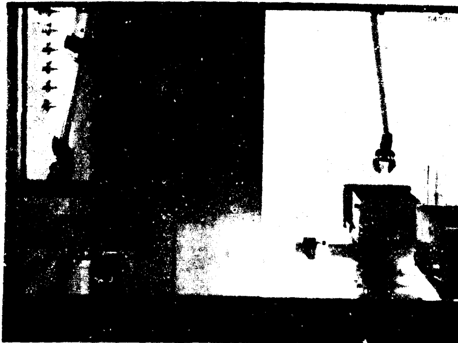
Fig. 46 - Example showing reach capability of heavy duty manipulators without extended reach feature
