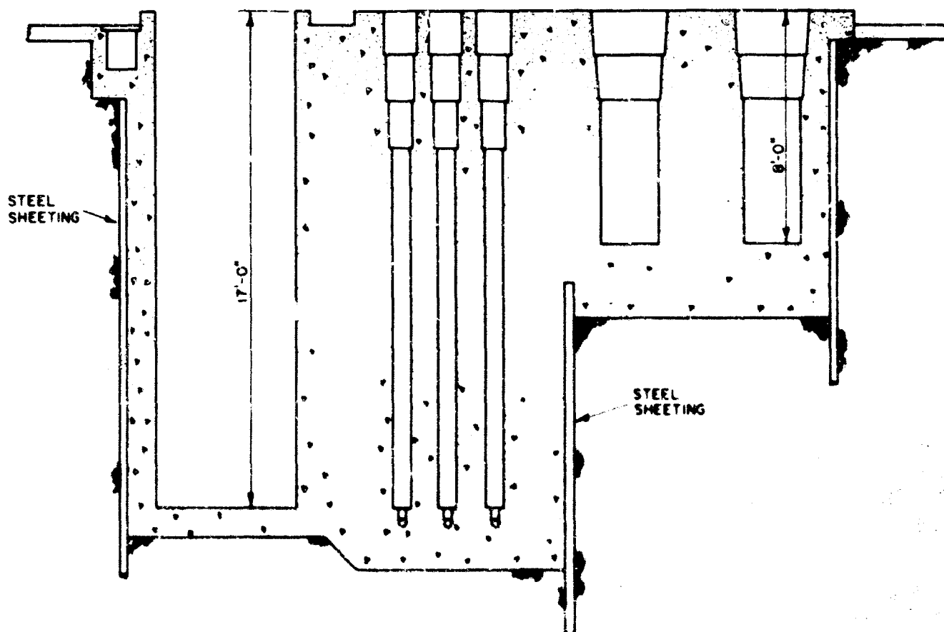
SECTION 32-32
