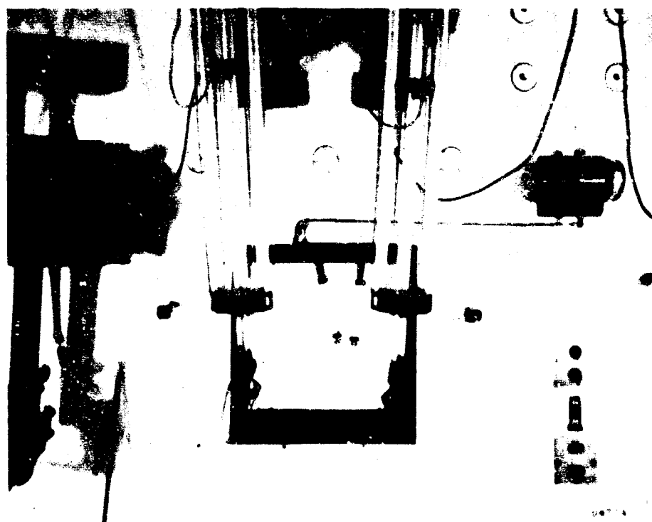
Fig. 45 - Example showing extension of slave arms without comparable extension of master ends
