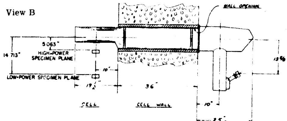
Fig. 64 - Bausch and Lomb remote control stereomicroscope: view A, assembly; view B, wall installation
