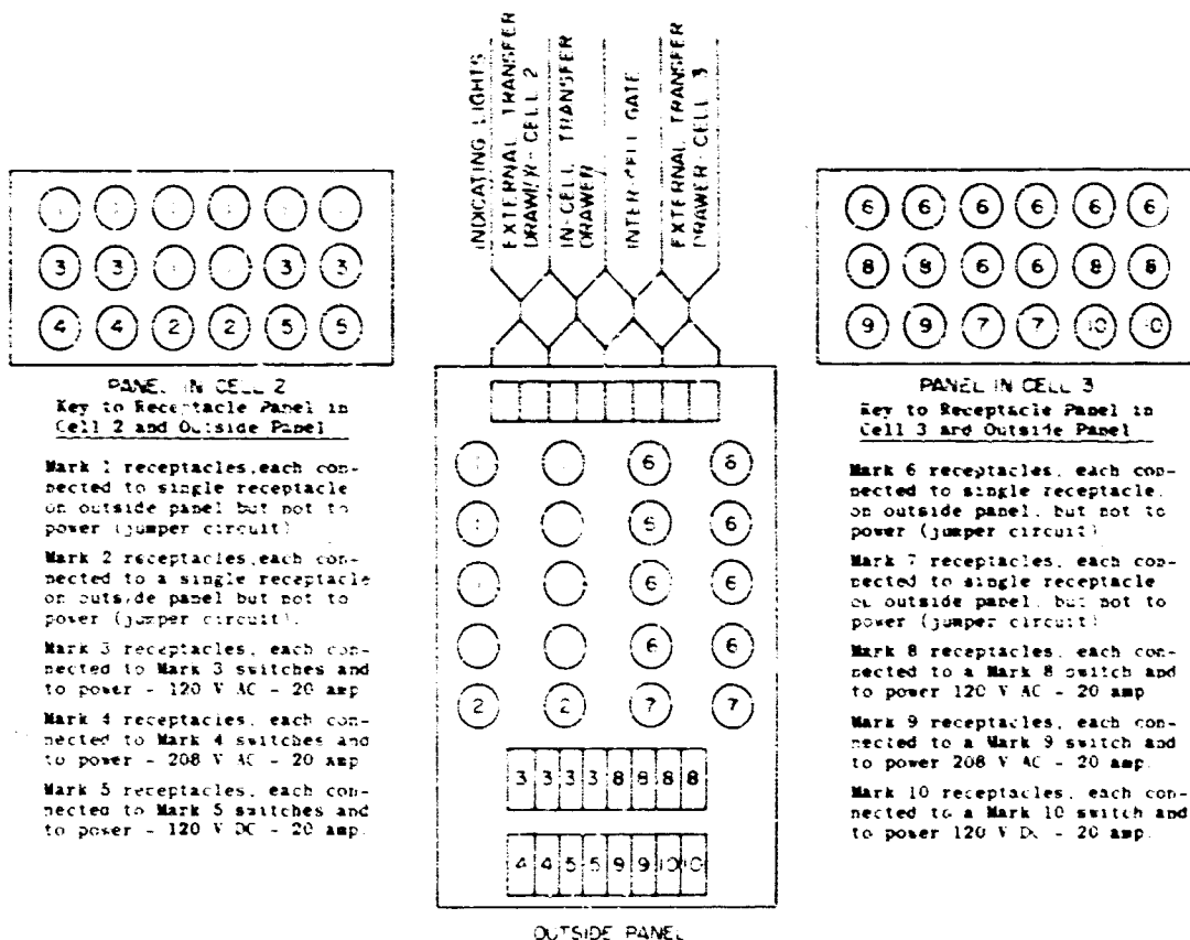
Fig. 5 - Typical example of in-cell and outside interconnected receptacle panels
