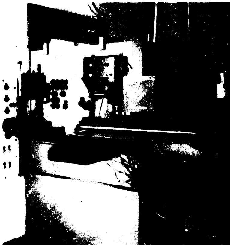
Fig. 66 - View of Reichert remote controlled shielded metallograph mounted against cell wall sealing plate
