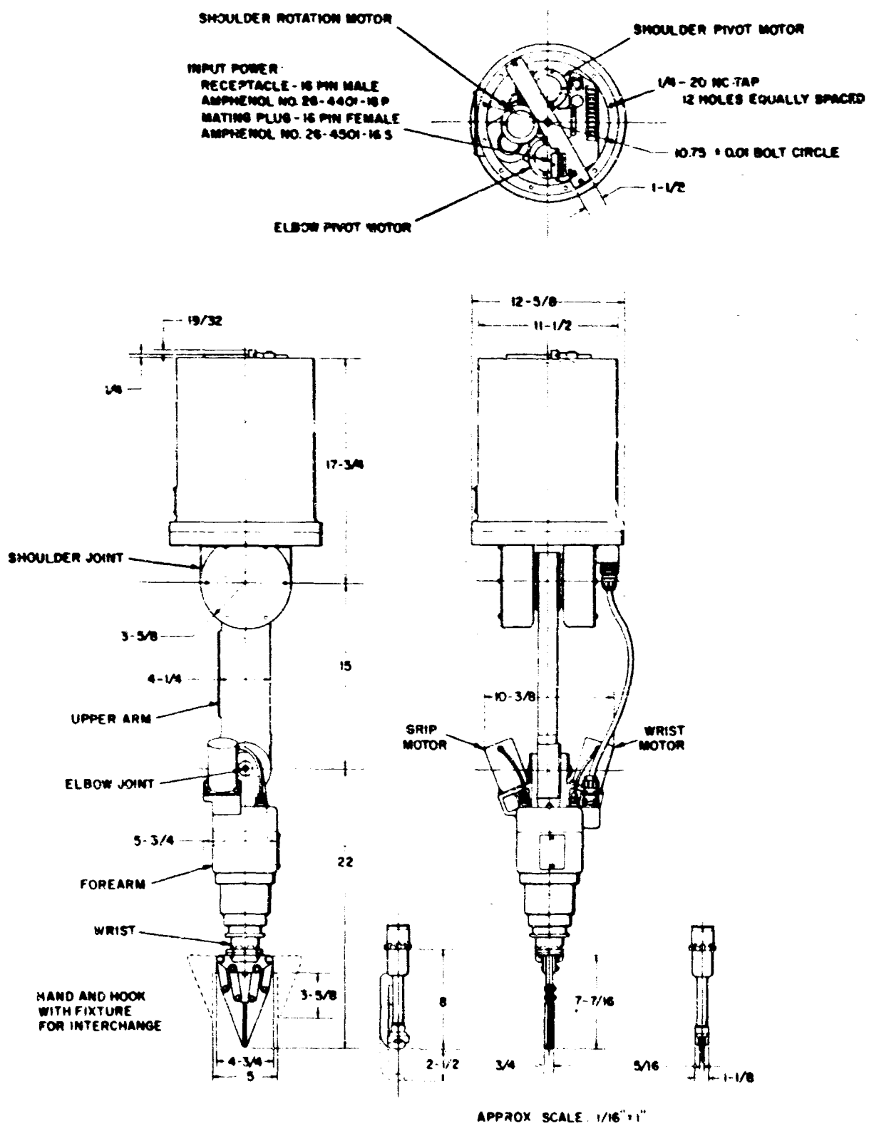
Fig. 52 - Mechanical arm assembly and dimensions
