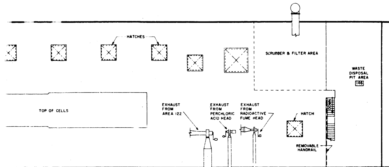
COND FLOOR PLAN
