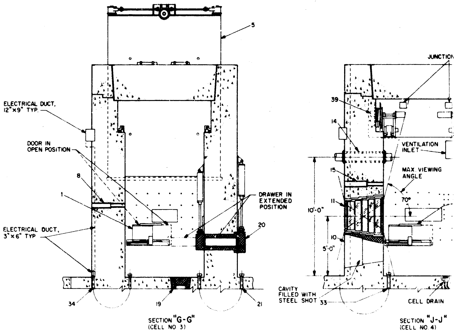
Dwg. 4. Typical elevations of hot-cell ends - sections G-G and J-J (Dwg. 2)
