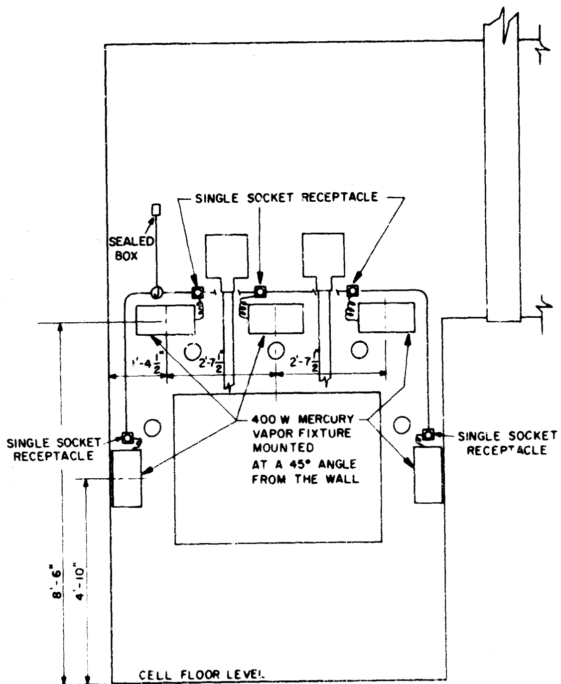
Fig. 7 - Arrangement of mercury lamps around viewing window
