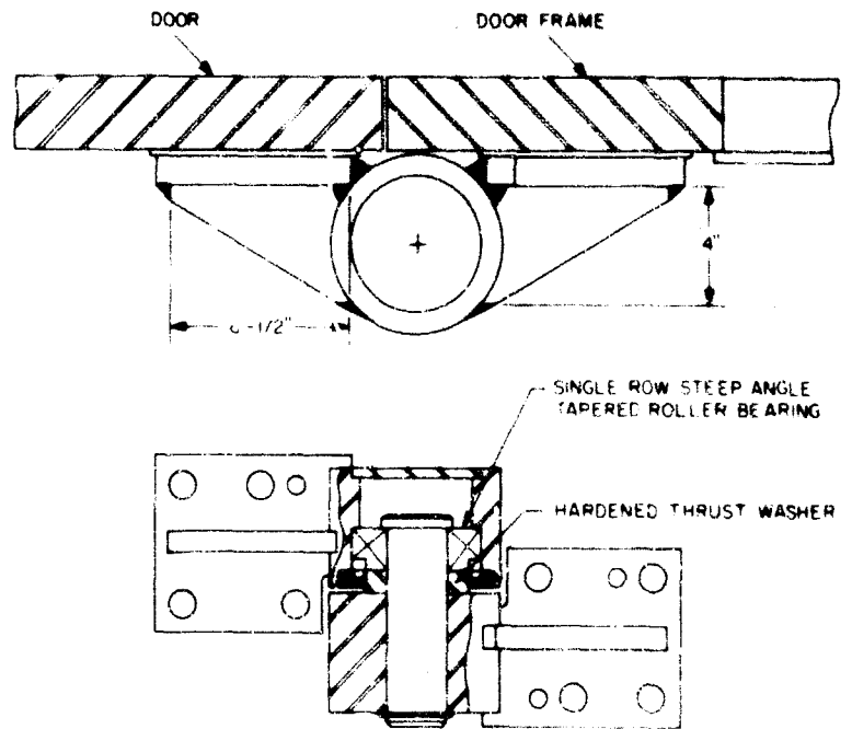
DETAIL "D" LOWER HINGE
