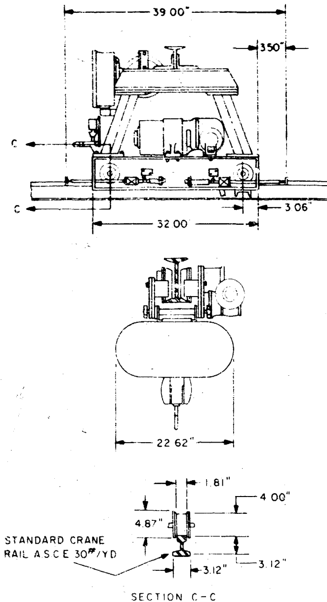
Fig. 61 - Sketches showing "A" frame end supports, bridge I-beam and trolley, and bridge wheel detail.
