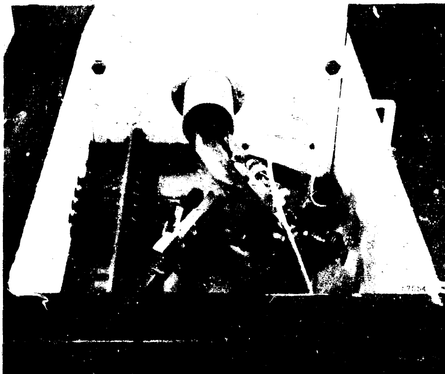
Fig. 68 - View inside shielded enclosure showing specimen transporter and metallograph stage with mechanical linkages
