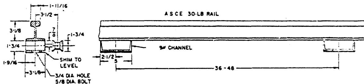
Fig. 49 - Track mounting pad and cable roller arrangement
