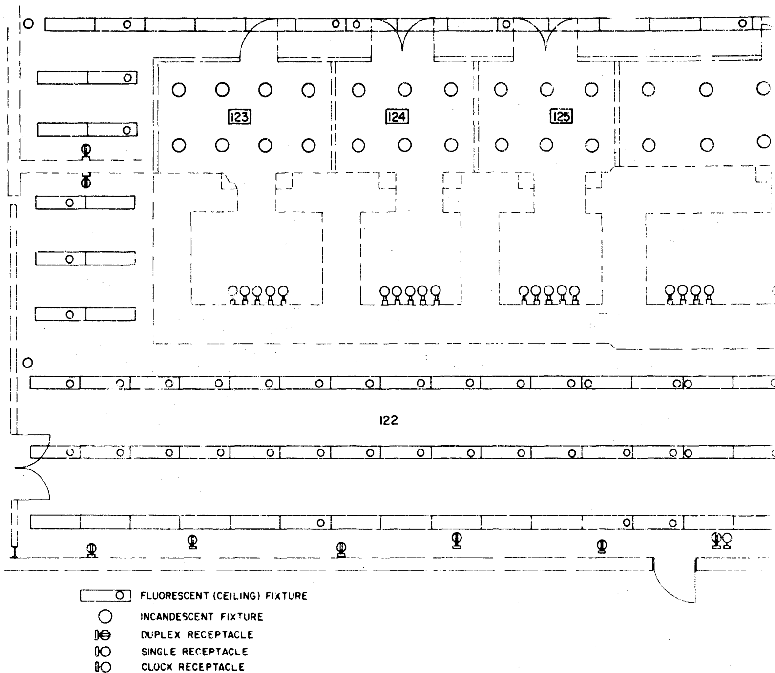
Dwg. 11. Lighting fixture arrangement in "cold" work area (122), hot
