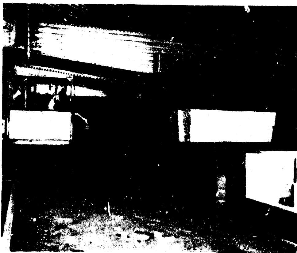
Fig. 22 - View of building crane handling and stacking removable roof plugs
