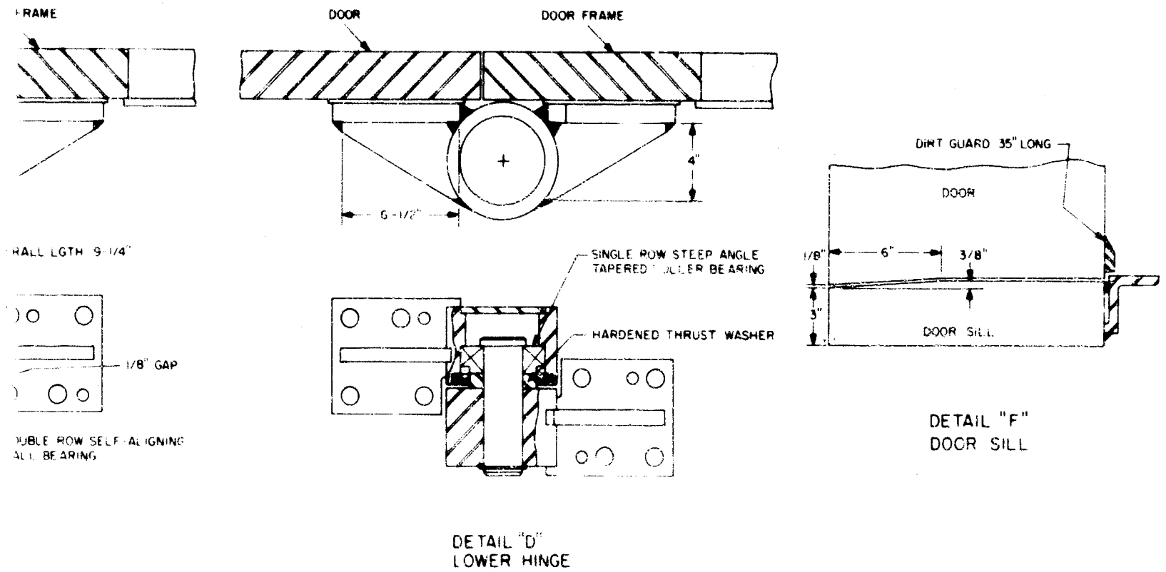
Dwg. 5. Typical upper and lower hinge design for steel shielding doors
