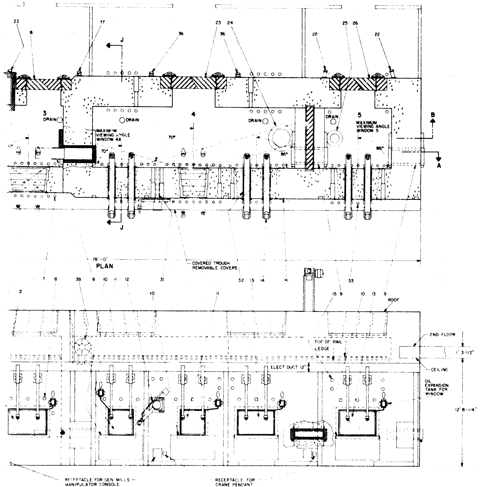
ELEVATION OF SOUTH WALL
