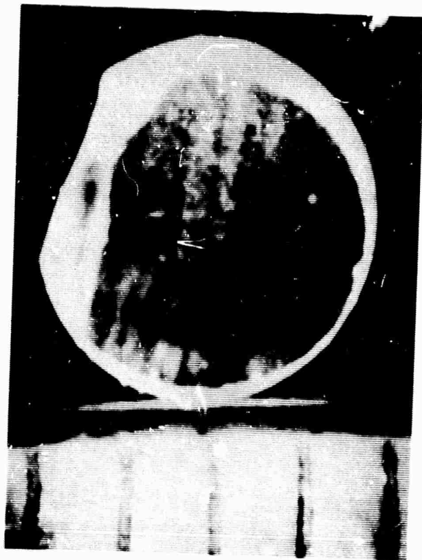
Fig. 5 - Lanthanum Fluoride Samples - Stratified Cloudiness
