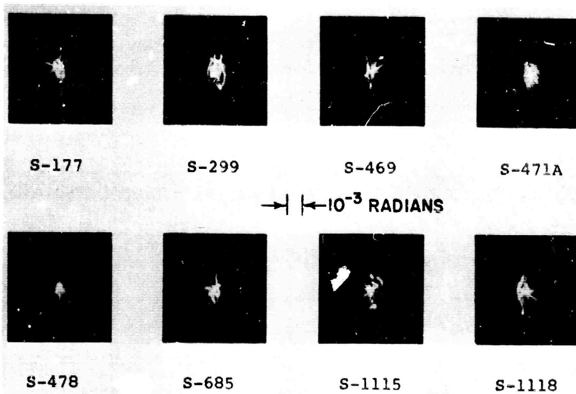
Fig. 7 - Large Ruby Rods - Far Field Patterns
