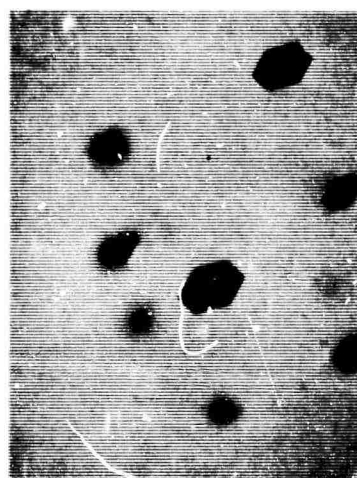
Fig. 3 - Lanthanum Fluoride Samples - Inclusions Seen at Slightly Different Depths
