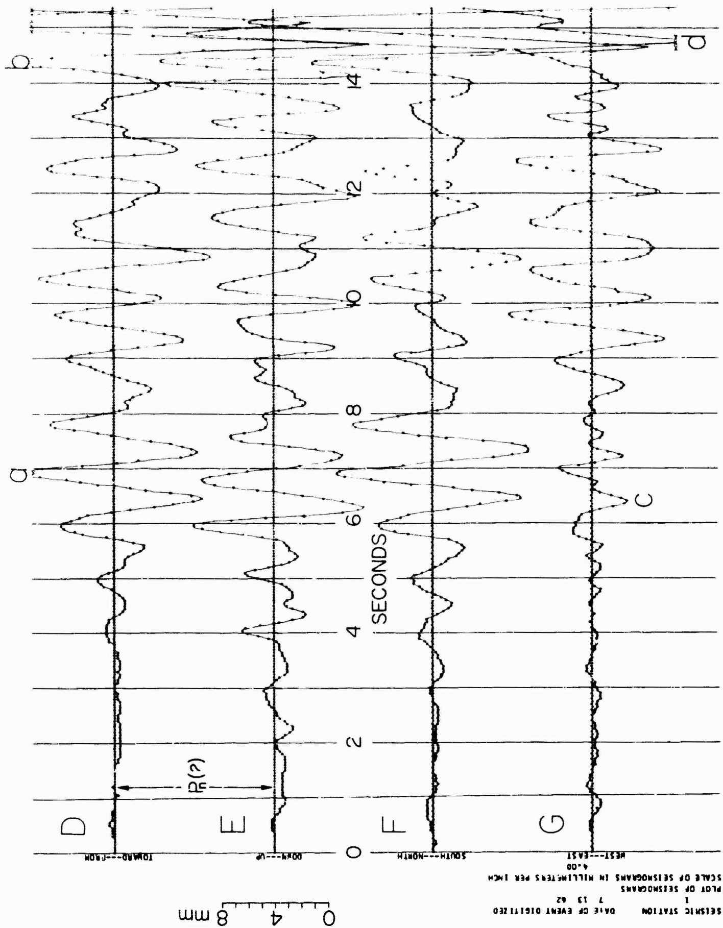
Figure 7-9. Digital-to-analog seismogram, MERRIMAC underground nuclear explosion, Nevada test site, July 13, 1962; 0.00 = 16h 01m 01.0s GCT.
