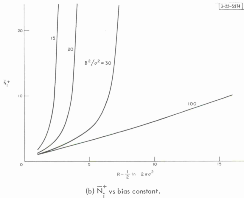
Fig. 11. Behavior of \bar{N} and its components vs bias constant.
