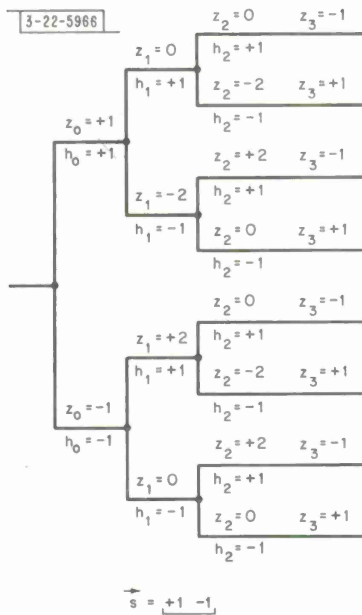
Fig. 3. Tree structure for a 3-component filter and a specific 2-component input.
