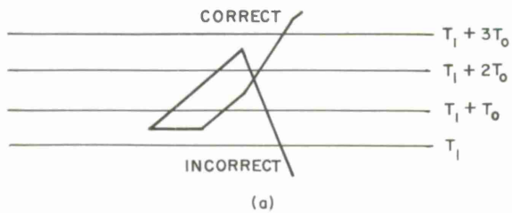
(a) Error when metric increases on correct path.
