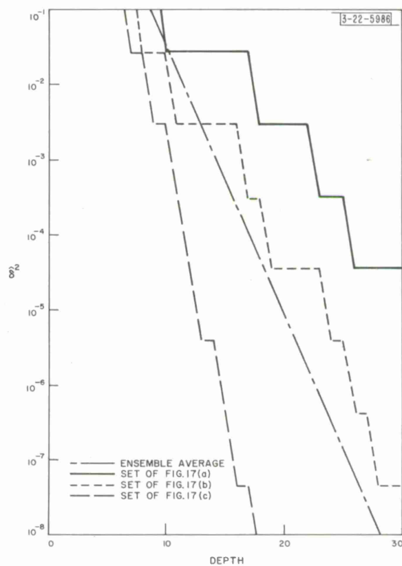
Fig. 19. Estimated \delta^2 vs depth.
