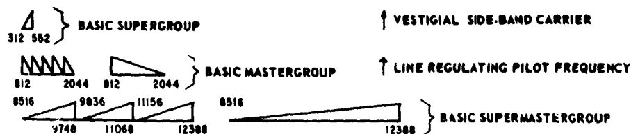
4 MC, 6 MC, 12 MC BASEBAND FREQUENCY ALLOCATIONS Showing Telephone and Television Frequency Allocations
