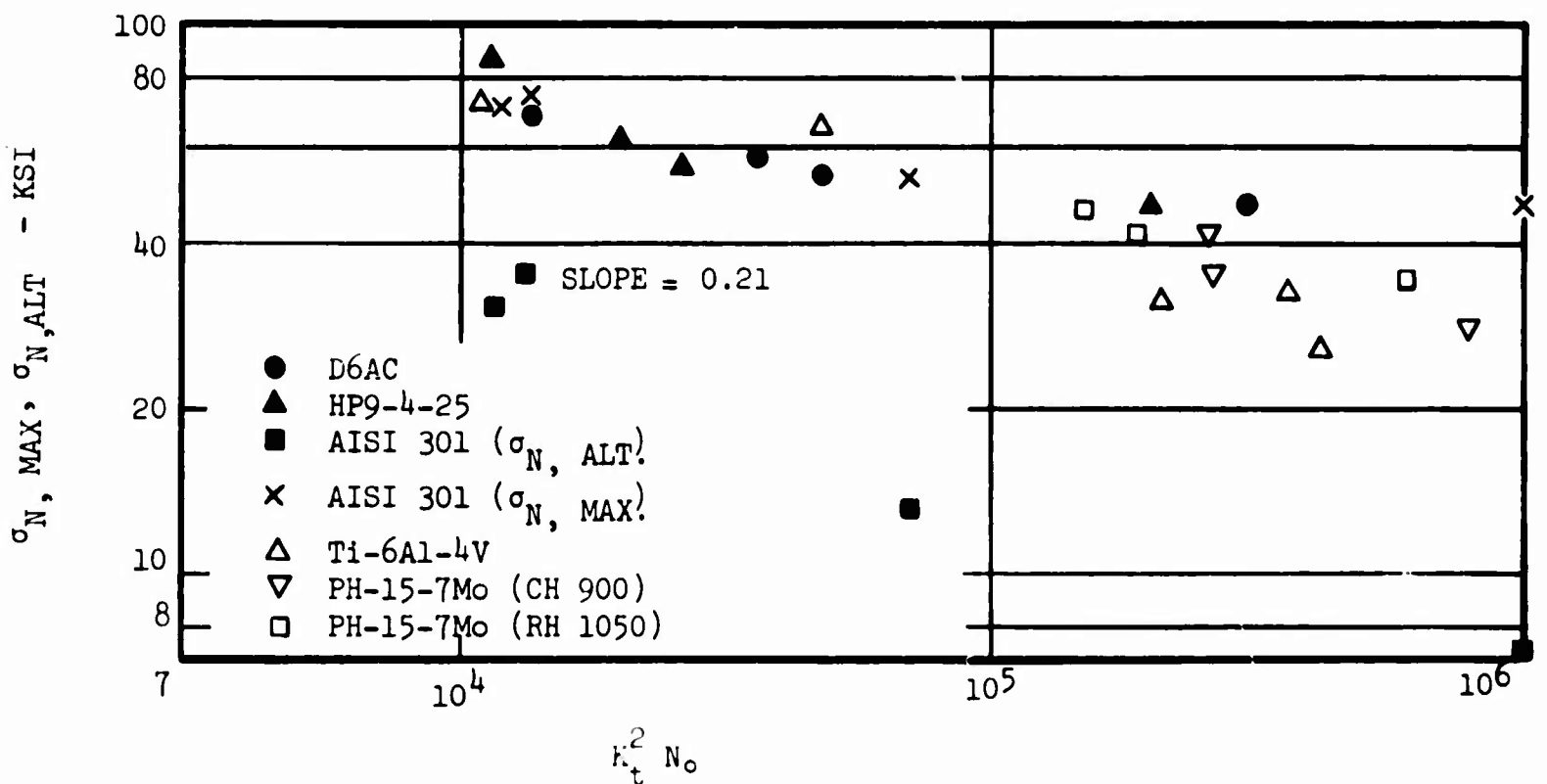
FIG. 41 \sigma_N VS (K_t^2 N_o) CURVE FOR ALL MATERIALS TESTED IN THE PRESENT STUDY
