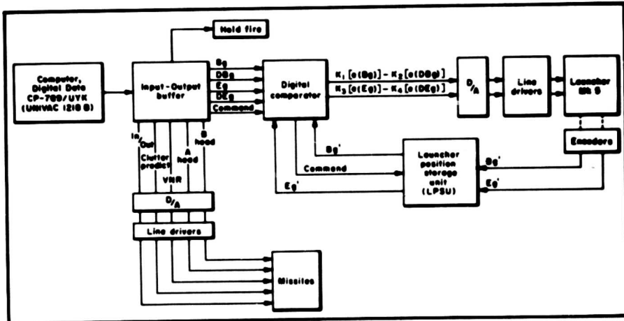
FIG. 6. Block Diagram of Digital-Analog Servo System (DASS).
