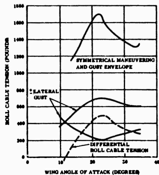
Figure 16. Limit Roll Cable Loads
