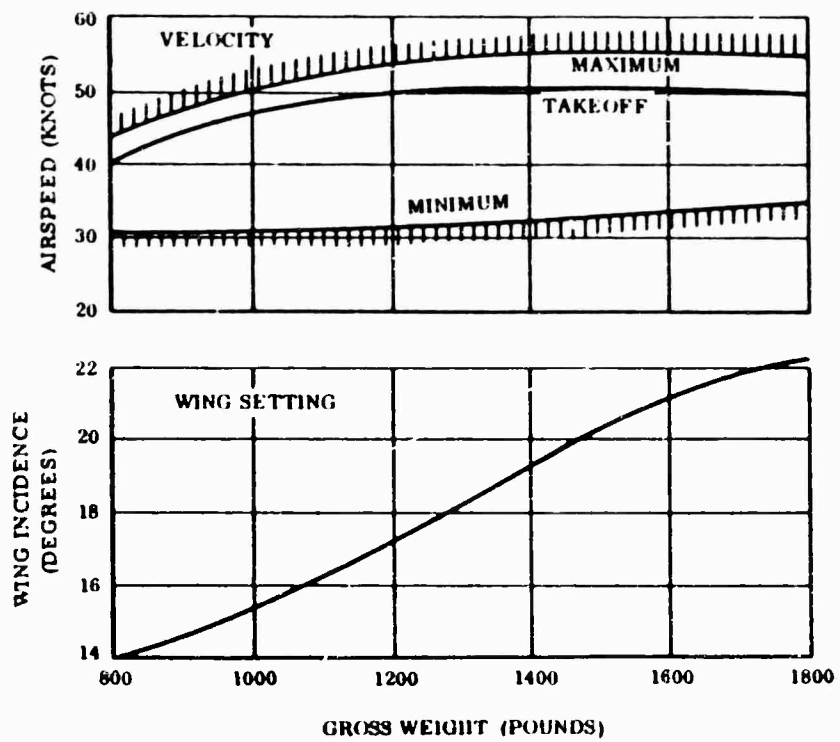
Figure 47. Takeoff (ACG Estimated Operating Parameters)
