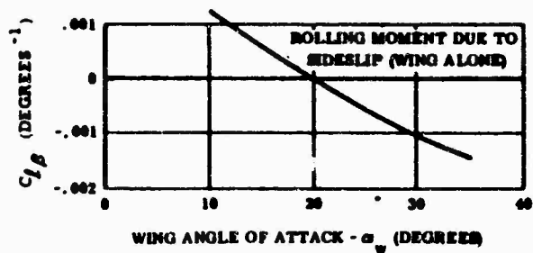
Figure 22. Dihedral Effect Characteristics for Wing Alone
