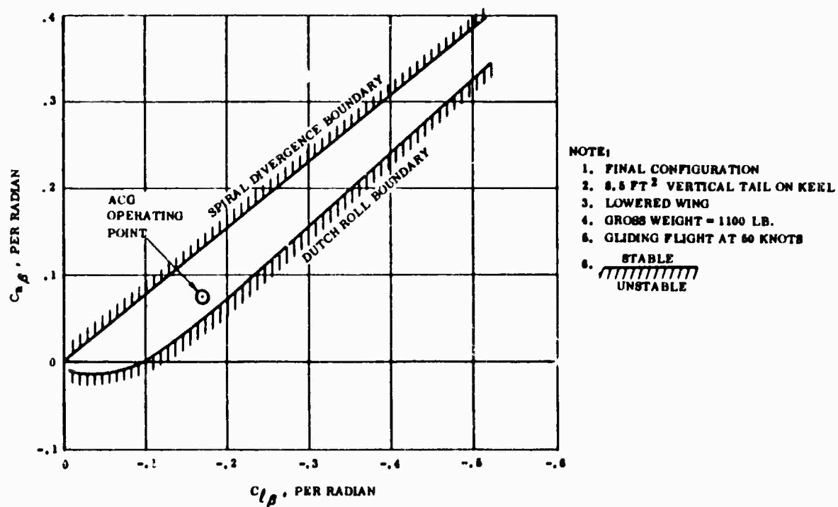
Figure 42. Lateral Directional Stability Boundaries (Final Configuration)
