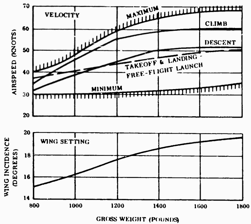
Figure 46. Complete Mission-One Wing Setting (ACG Estimated Operating Parameters)
