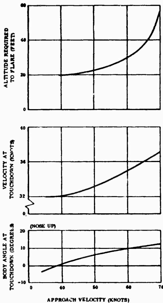
Figure 34. Landing Characteristics
