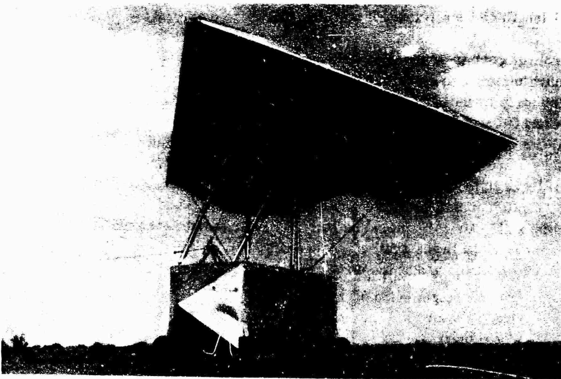
Figure 2. Air Cargo Glider - Left Front View
