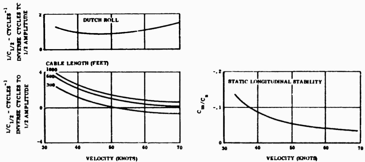
Figure 27. On-Tow Stability
