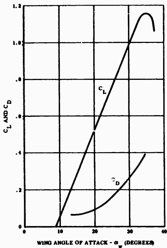
Figure 21. Lift and Drag Characteristics (Wing Only)
