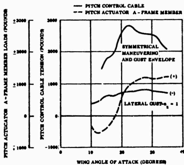
Figure 15. Limit Pitch Control Cable and Pitch Actuator, A-Frame Loads
