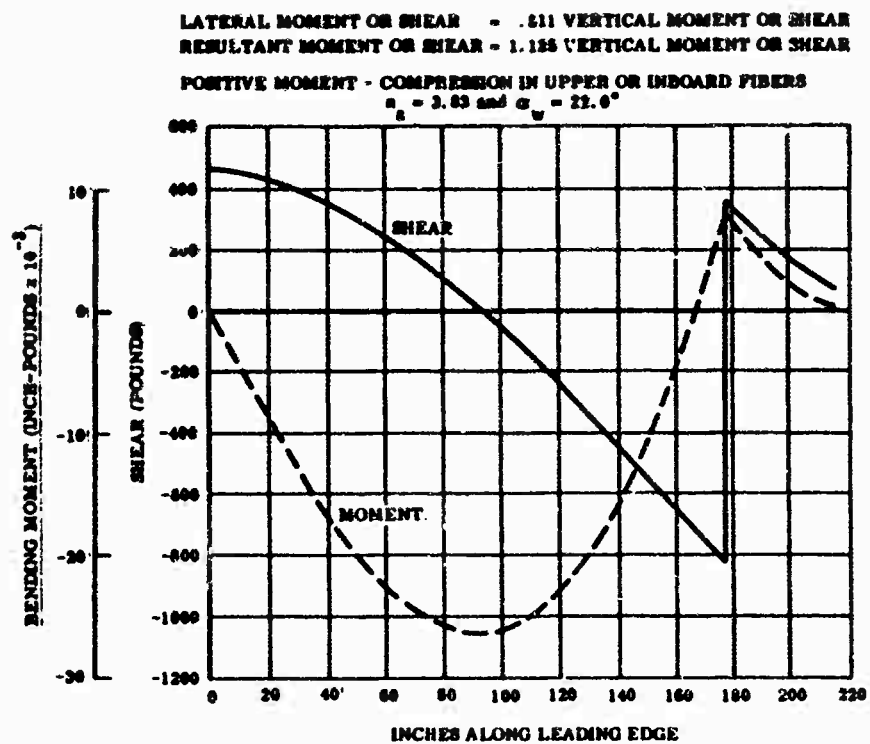
Figure 11. Leading Edge Limit, Vertical Shear and Moment
