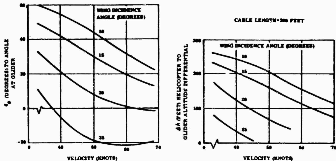
Figure 28. Glider Tow Angle and Associated Altitude Separation
