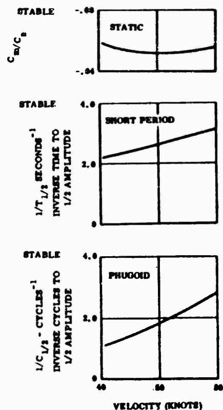
Figure 30. Off-Tow Longitudinal Static and Dynamic Stability
