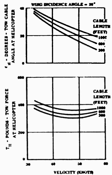
Figure 26. Two Characteristics of the Helicopter
