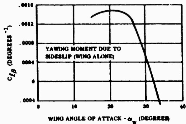
Figure 23. Directional Stability For Wing Alone
