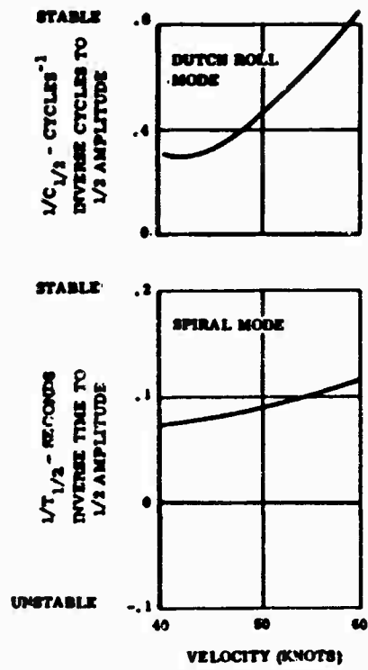
Figure 31. Off-Tow Lateral Directional Stability
