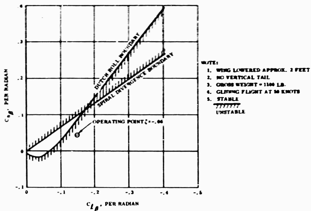
Figure 41. Lateral Directional Stability Boundaries (Lower Wing)
