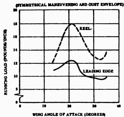
Figure 13. Peak Limit Membrane Running Load at the Leading Edge and Keel
