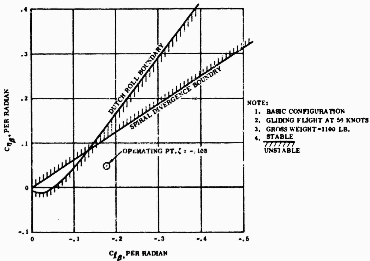
Figure 37. Lateral Directional Stability Boundaries (Basic)
