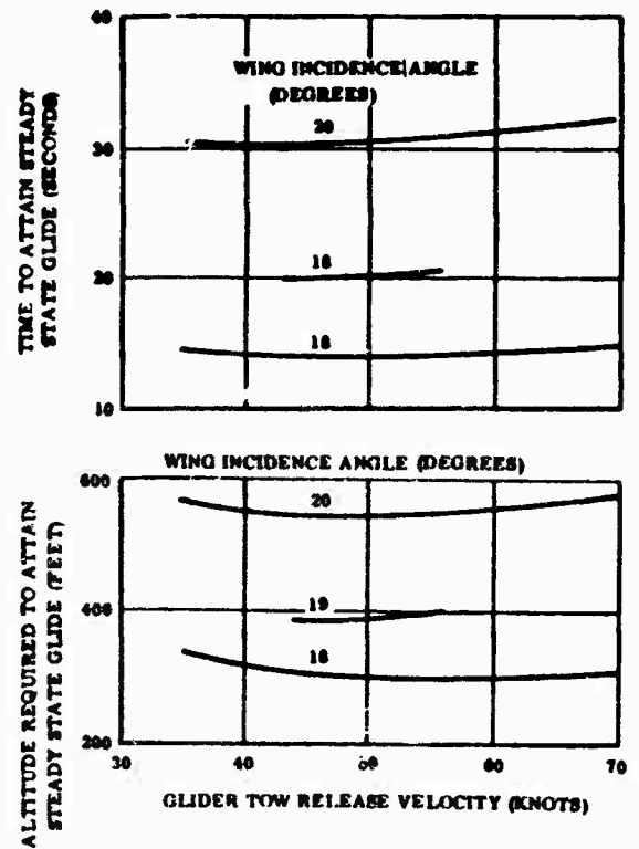
Figure 32. Glider Characteristics At Tow Release
