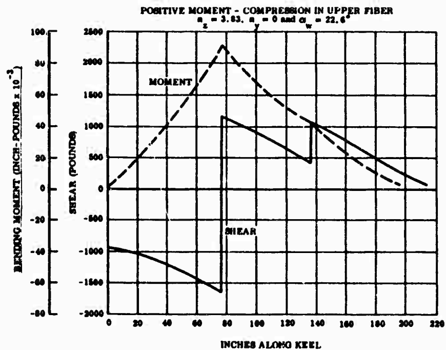
Figure 12. Keel Limit, Vertical Shear and Moment
