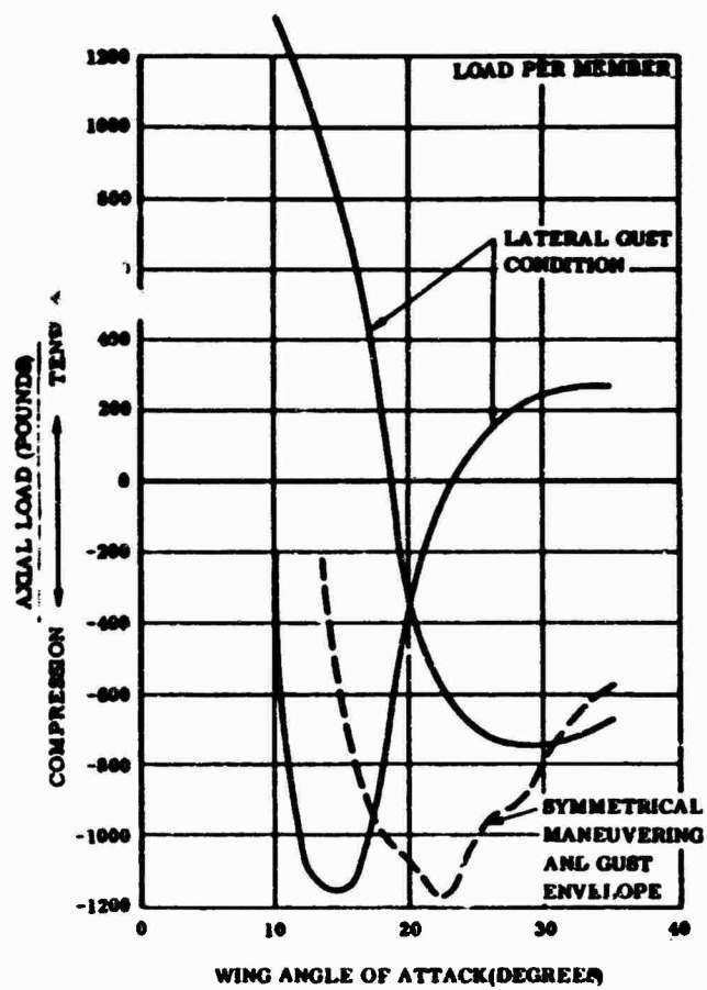
Figure 17. Limit Load in Forward Members of Tripod
