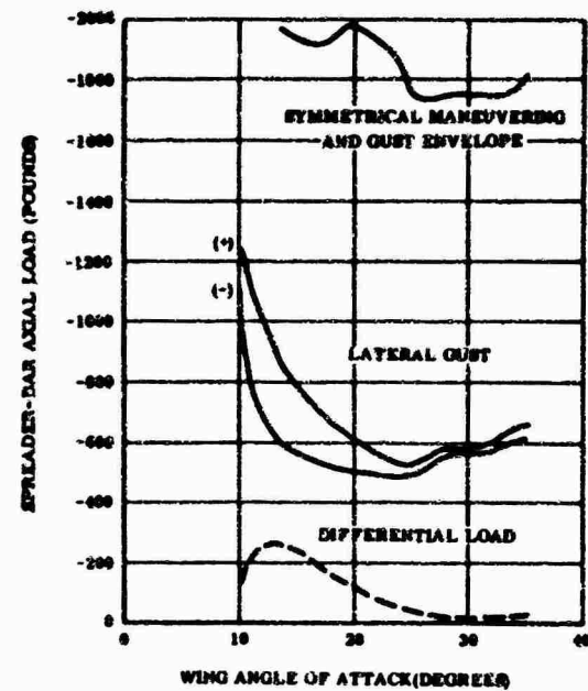
Figure 14. Limit Wing Spreader Bar Loads
