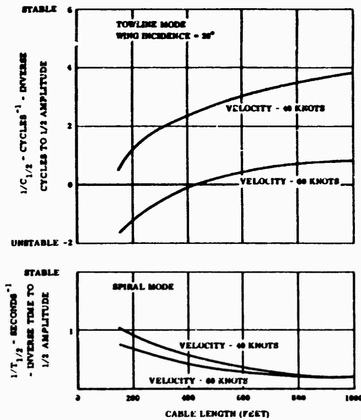
Figure 25. Effect of Cable Length on Lateral Directional On-Tow Stability
