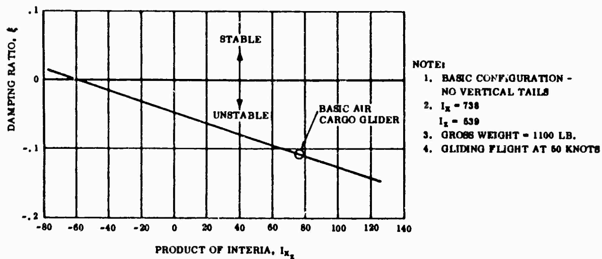
Figure 40. Dutch Roll Damping Ratio as a Function of Product of Inertia
