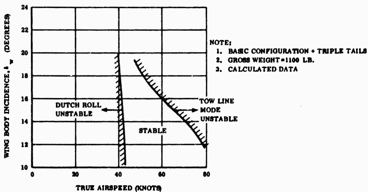
Figure 38. Tow-Speed Boundaries
