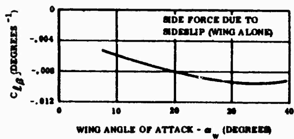
Figure 24. Side Force Variation For Wing Alone
