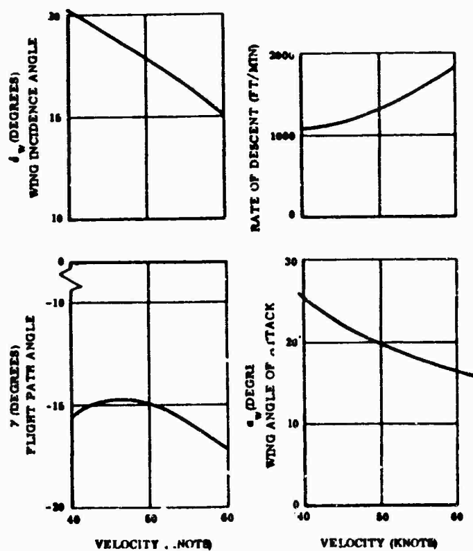
Figure 29. Off-Tow Performance Characteristics
