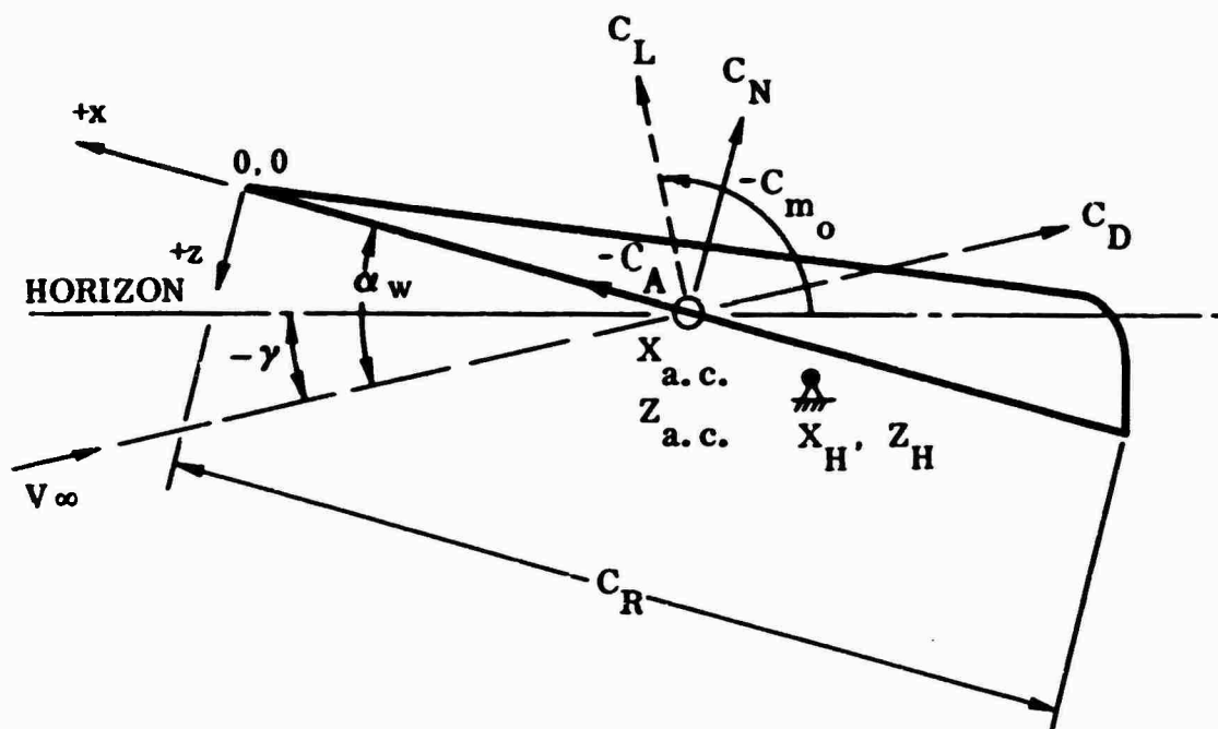
Figure 19. Pictorial Description of Wing Terms (Aerodynamic)
