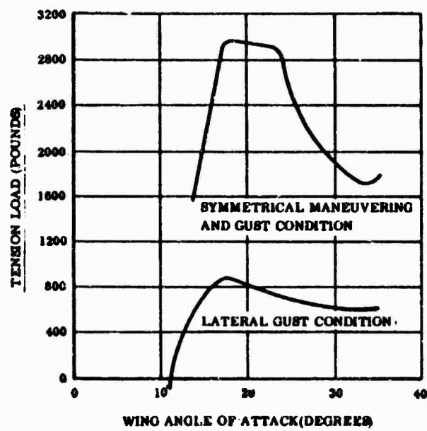
Figure 18. Limit Load in Aft Member of Tripod
