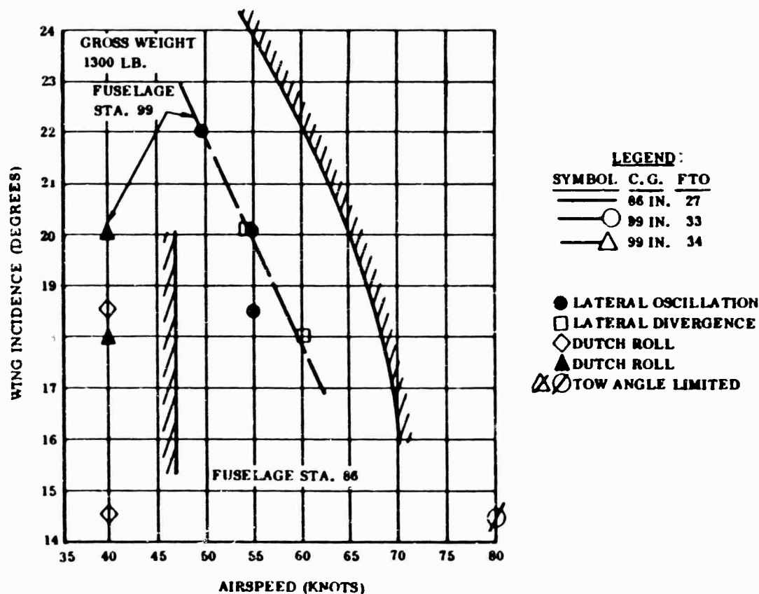
Figure 43. Flight Envelope - C.G. Effect
