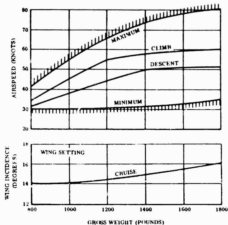
Figure 48. Climb, Cruise and Descent (ACG Estimated Operating Parameters)
