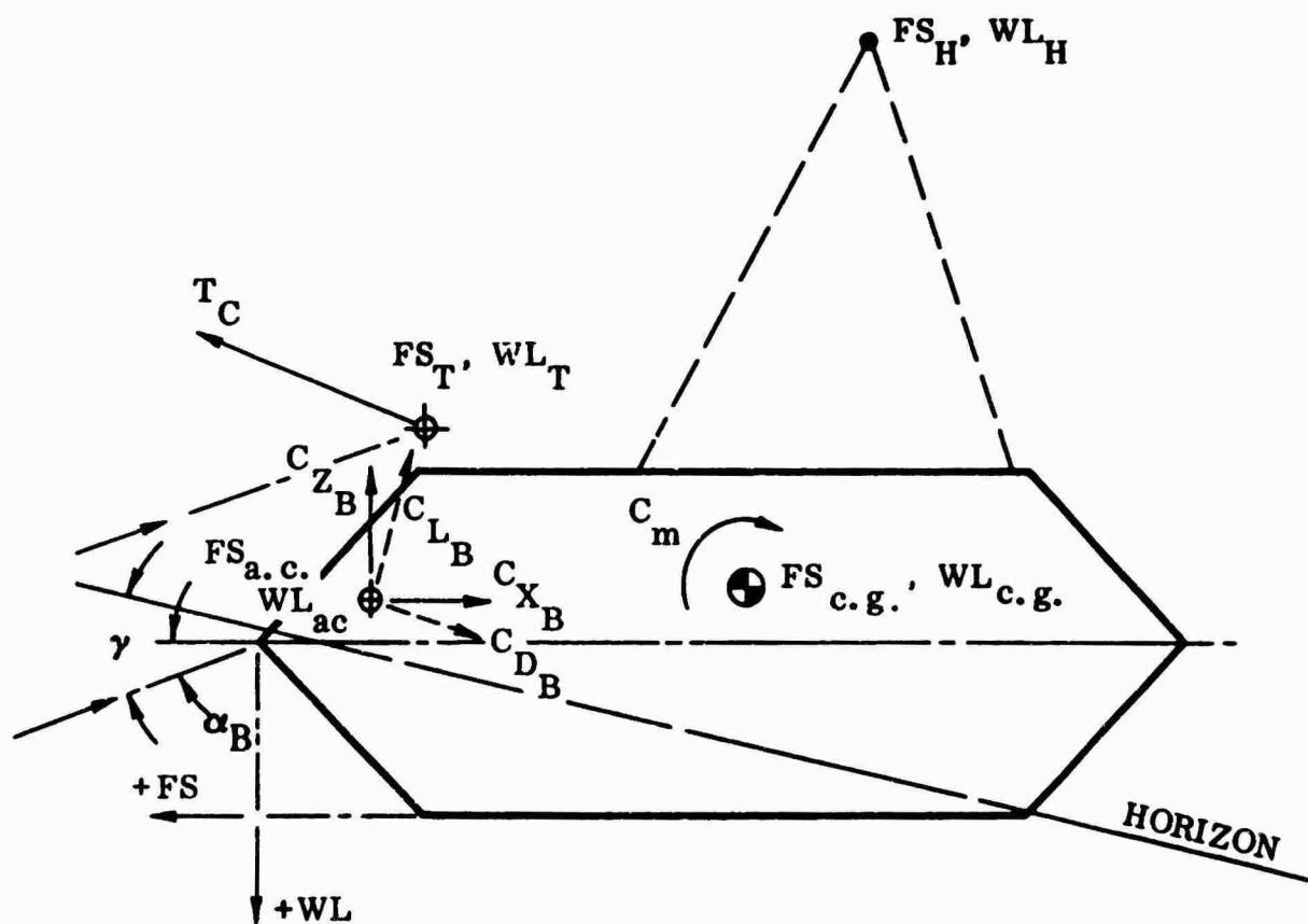
Figure 20. Pictorial Description of Body Terms (Aerodynamic)
