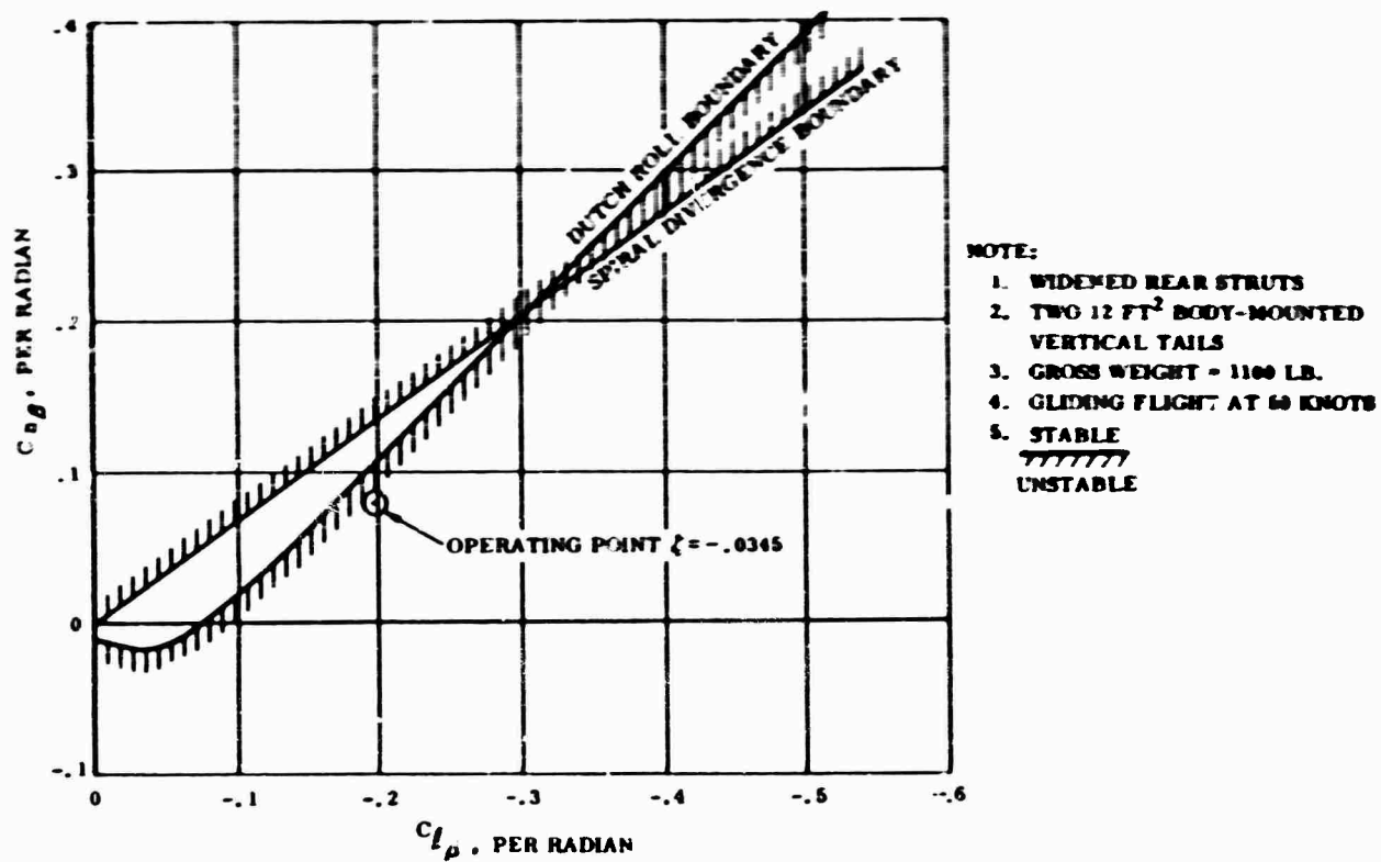
Figure 39. Lateral Directional Stability Boundaries (Two Vertical Tails)
