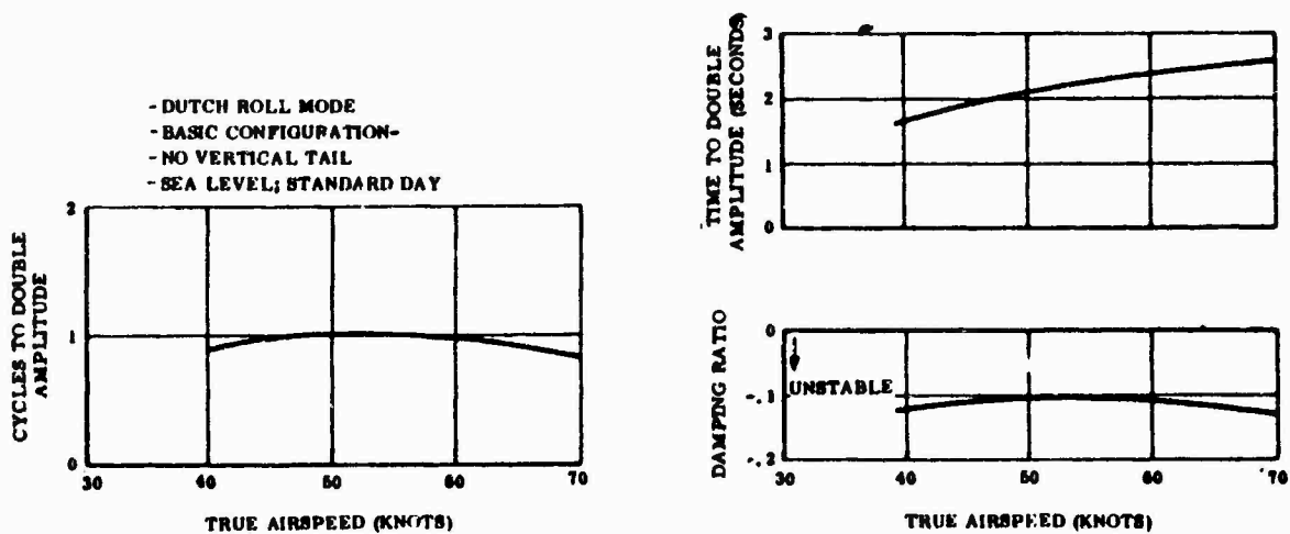
Figure 36. Dynamic Stability
