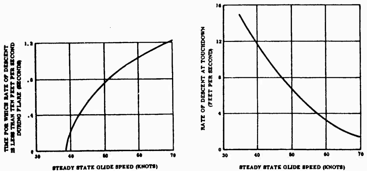
Figure 33. Touchdown Characteristics
