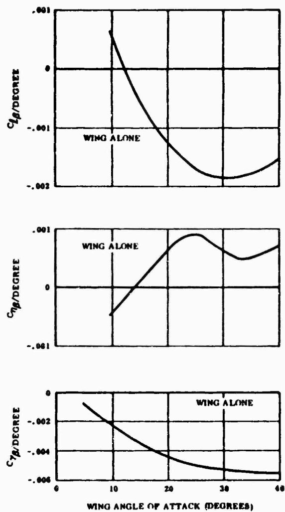
Figure 35. Lateral Directional Static Stability (Wing Only)
