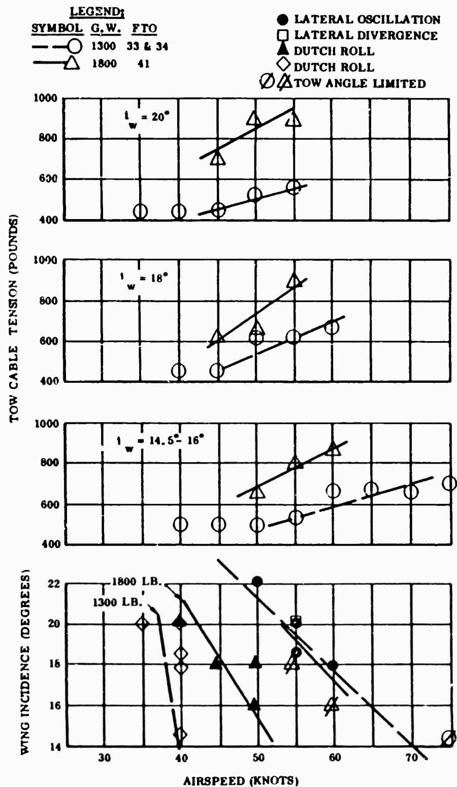
Figure 44. Gross Weight Effect - C.G. Fuselage Station 99
