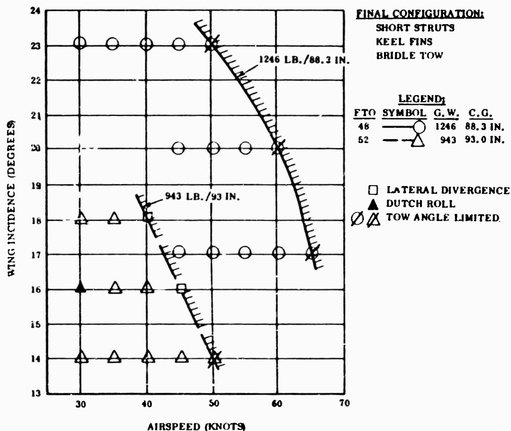
Figure 45. Flight Envelopes - Final Configuration
