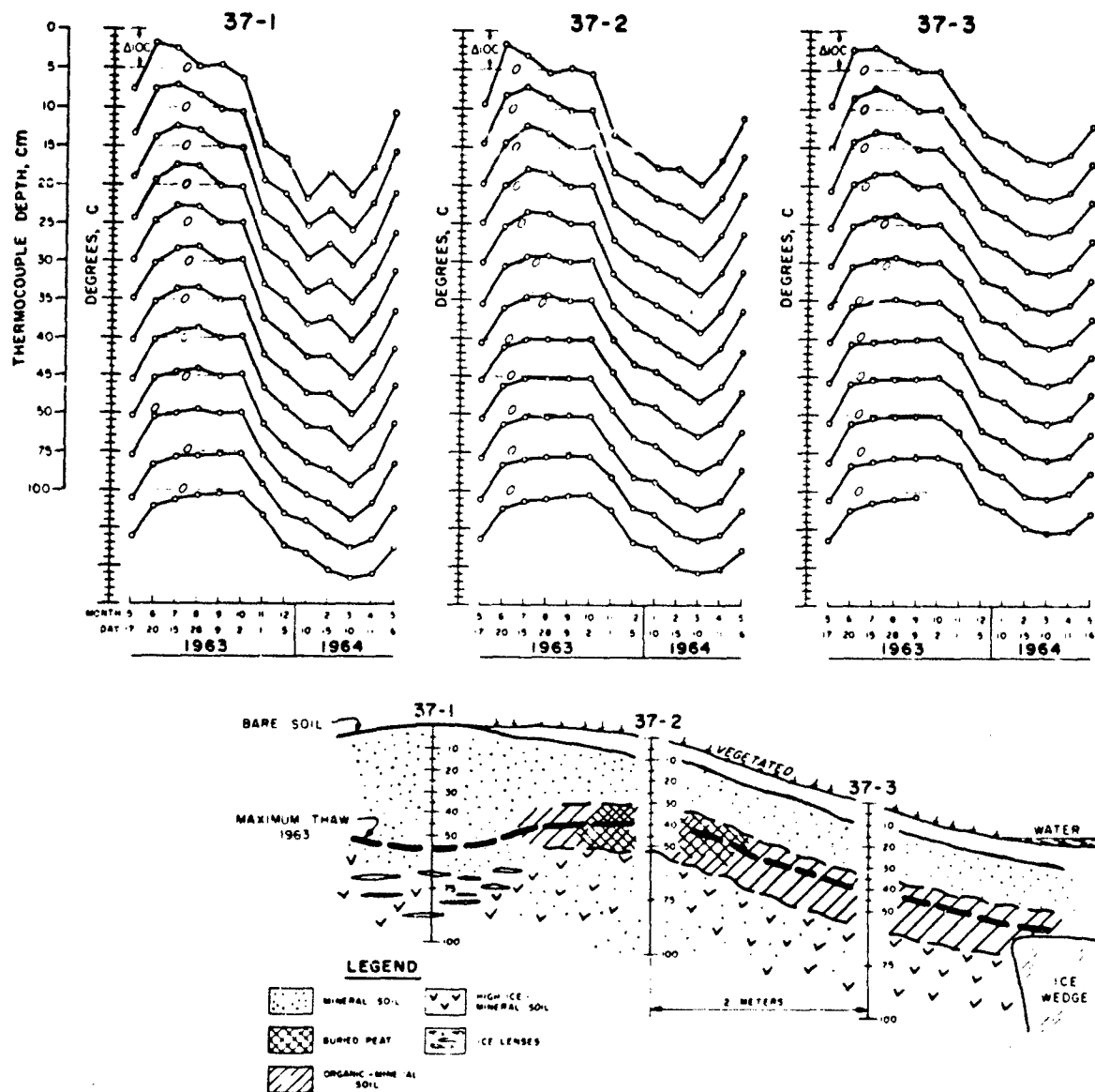
Figure 18. Thermocouple installation and selected soil temperatures, Plot 37, Barrow, Alaska. The vertical temperature scale is read above or below the zero isotherm for each individual thermograph. Each minor scale division represents 2°C.
