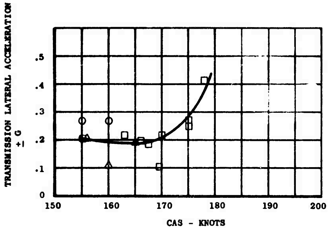
Figure I-25. TRANSMISSION LATERAL VIBRATORY ACCELERATION
