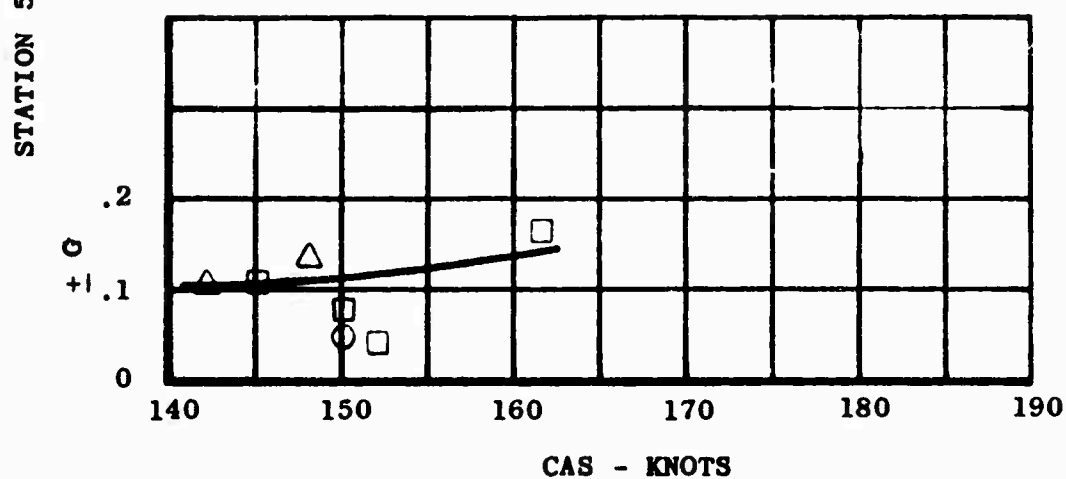
Figure I-23. STATION 50 VERTICAL VIBRATORY ACCELERATION.
