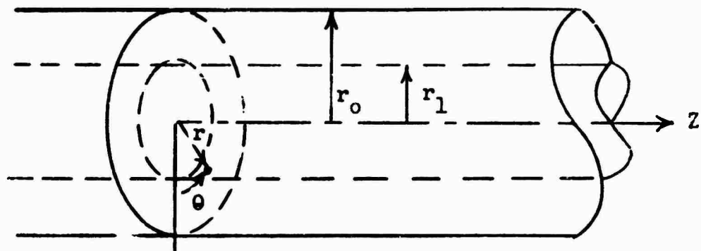
Figure 56. Mathematical Model.
