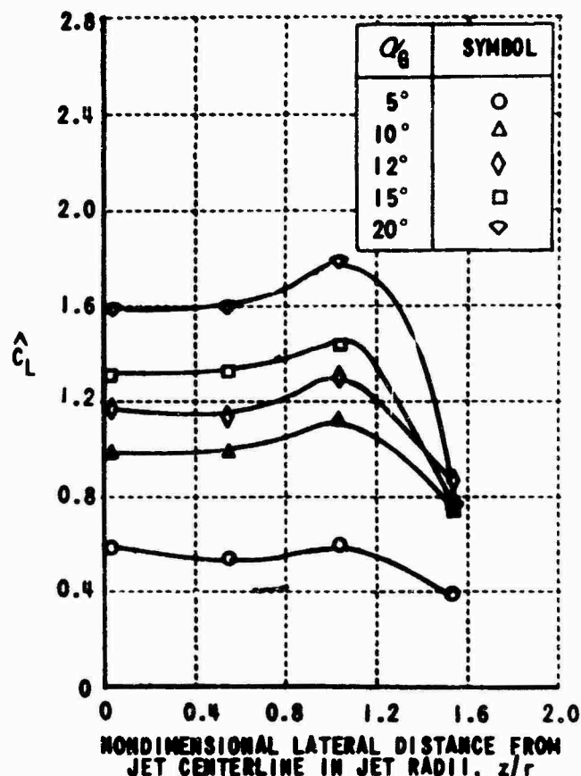
(b) NONDIMENSIONAL HEIGHT OF WING MIDCHORD ABOVE JET CENTERLINE IN JET RADI, h/r = 0.46
