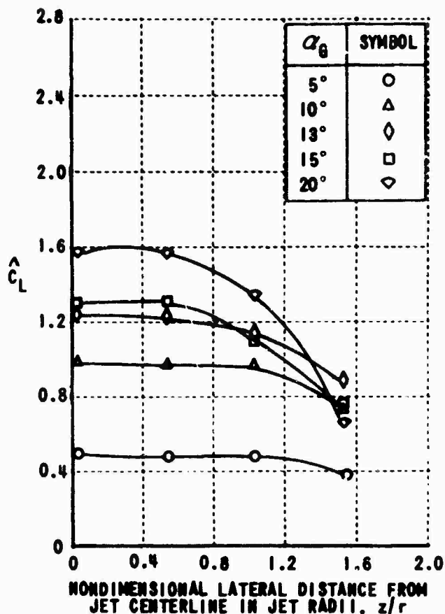
(a) NONDIMENSIONAL HEIGHT OF WING MIDCHORD ABOVE JET CENTERLINE IN JET RADI, h/r = 0.76
