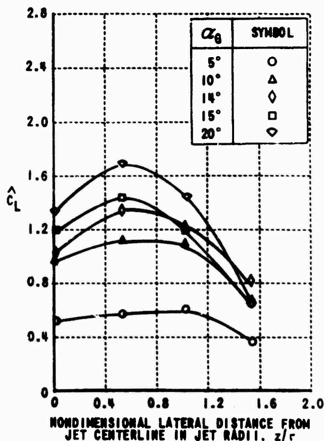
(d) NONDIMENSIONAL HEIGHT OF WING MIDCHORD ABOVE JET CENTERLINE IN JET RADI, h/r = -0.64
