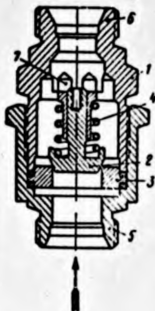
Figure 211. Return valve.
