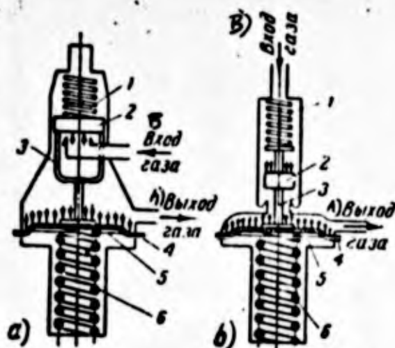
Figure 162. Diagram of the reducers of direct and reverse action.
