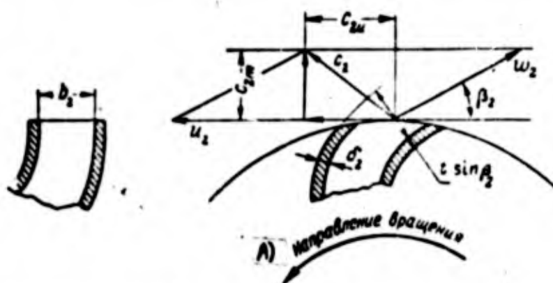
Figure 174. The diagram of velocities at the exit from the wheel.
