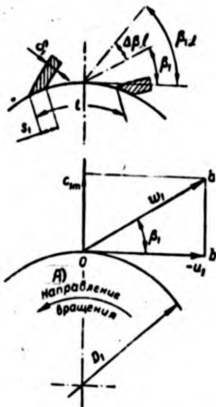
Figure 172. Diagram of velocities at the entrance to the wheel.
