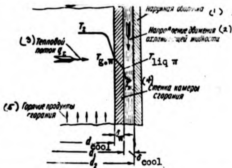
Figure 95. Explanation of the process of heat exchange in the liquid-fuel rocket engine.
