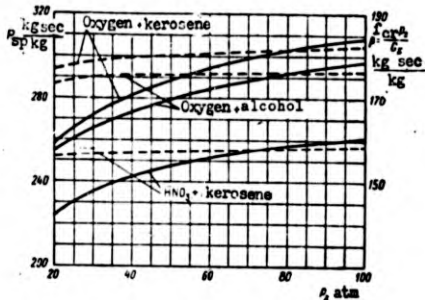
Figure 86. The dependence of specific thrust P_{sp} and the parameter complex \beta = \frac{F_{cr} p_3}{G_1} on the combustion chamber pressure for different fuels ( p_3 = \text{const} = 1 \text{ atm} ). The dotted lines are the graph of \beta .
