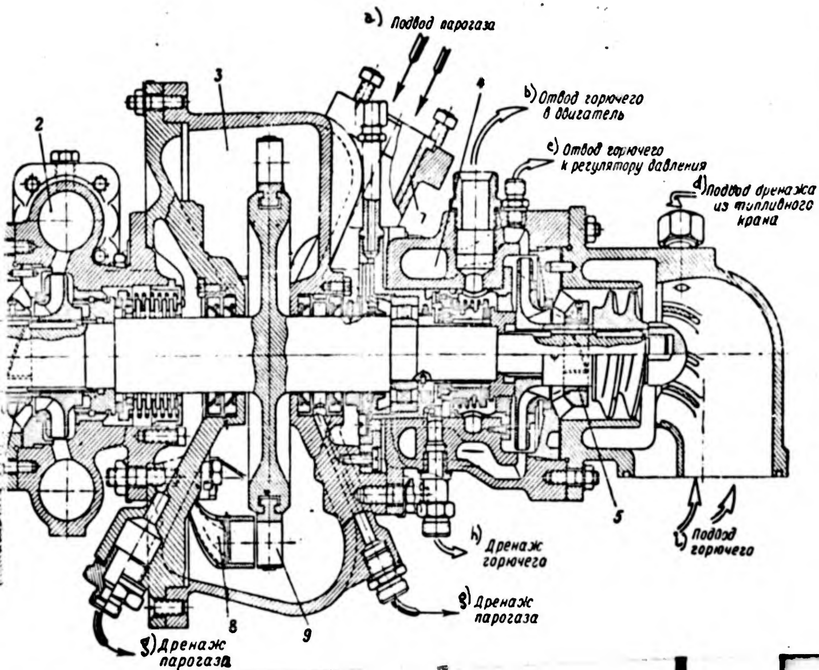
Diagram of the turbo-pump unit of the "Walter" engine
