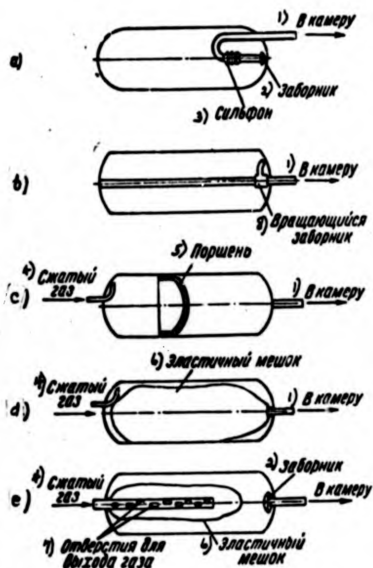
Figure 157. Diagrams of feed structures for feed components from the tanks.
