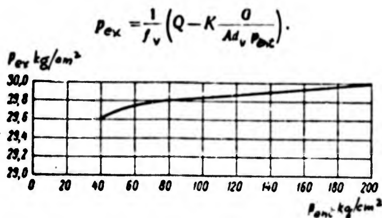
Figure 169. Estimated performance of the reducer.
