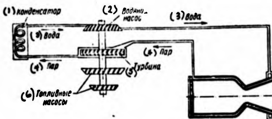
Figure 100. Diagram of cooling the engine chamber with water and subsequently using the stream that has formed to drive a turbine.
