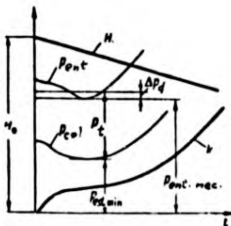
Figure 180. Change in the pressure of the column of liquid during the time of flight of the rocket and determination of the necessary pressure in the tank.
