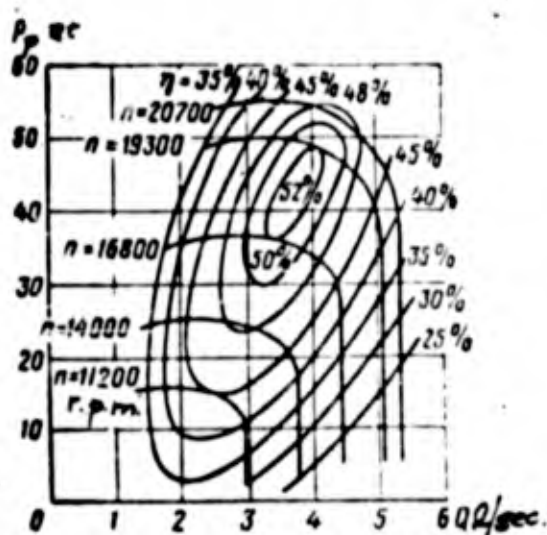
Figure 197. Characteristic of the centrifugal pump for nitric acid of engine R-3395, found in tests with water.
