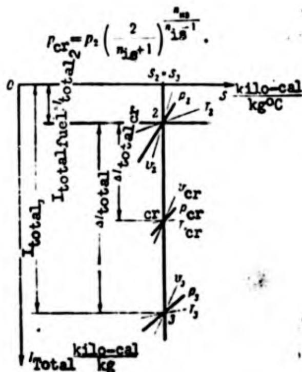
Figure 83. Scheme of the thermal calculation of the rocket engine by the I_{\text{total}}S - diagram.
