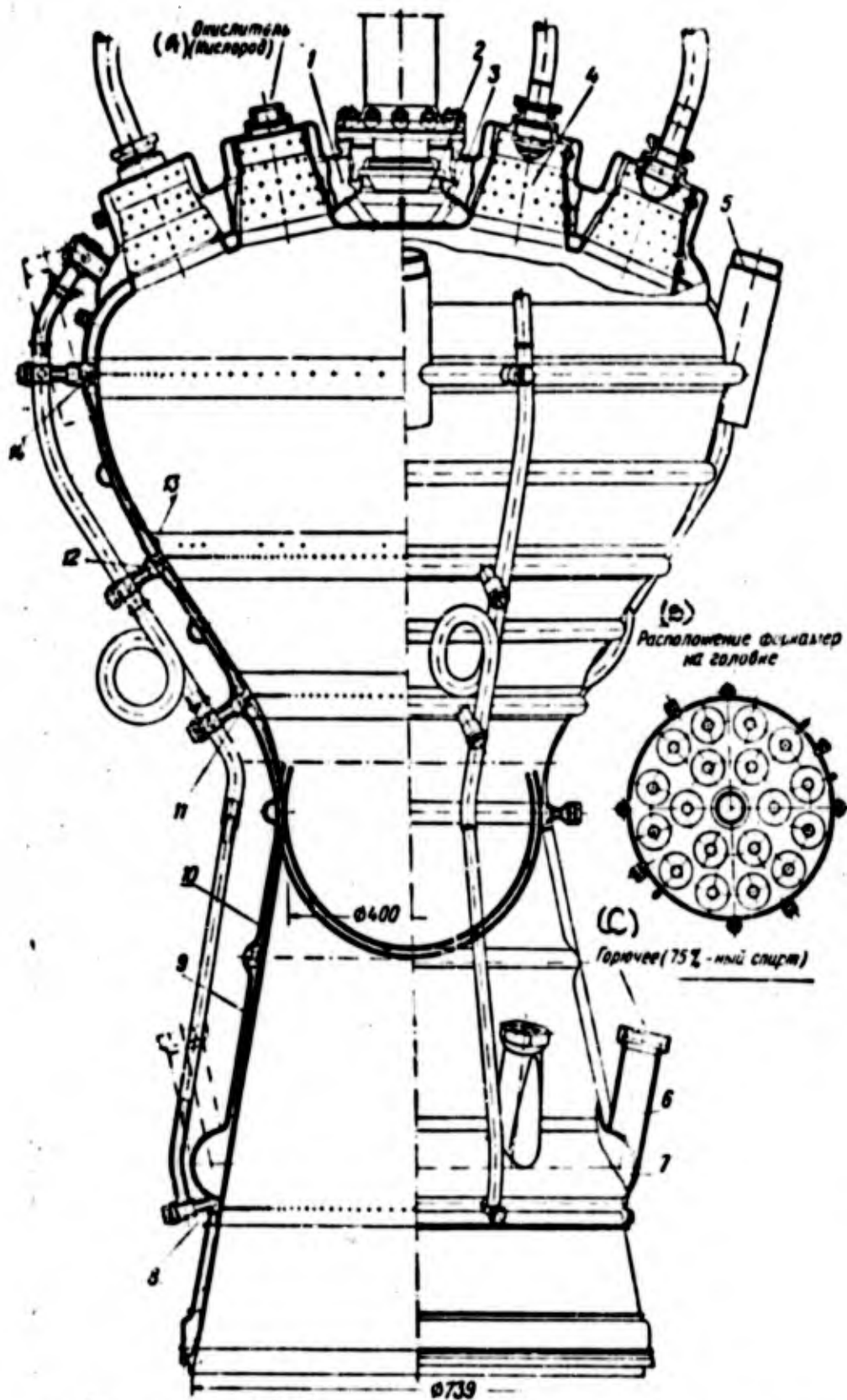
Figure 124. The combustion chamber of the A-4 rocket.
