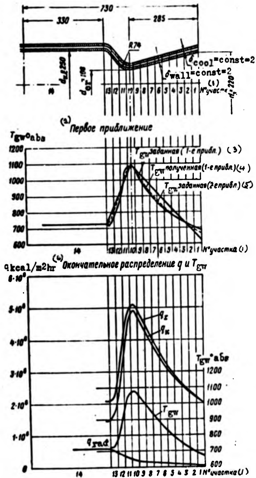
Figure 107. Illustrating the example of calculation of the cooling of an engine chamber.
