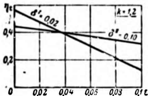
Figure 67. Change in thermal efficiency ( \eta_t ) depending on the change in the degree of possible expansion \varepsilon in the nozzle for an engine having different values for the degree of expansion \delta in the nozzle.
