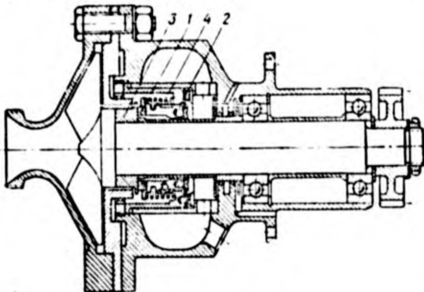
Figure 201. Section of the centrifugal pump for hydrogen peroxide.
