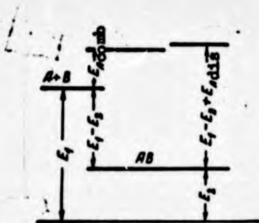
Figure 49. A diagram of the energy levels in simple and reversible reactions.
