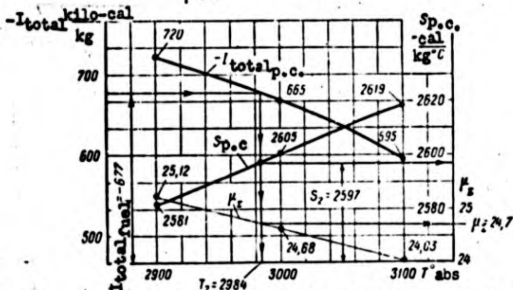
Figure 90. The solution of the example. Determination of T_2 ; S_2 and \mu_2 .
