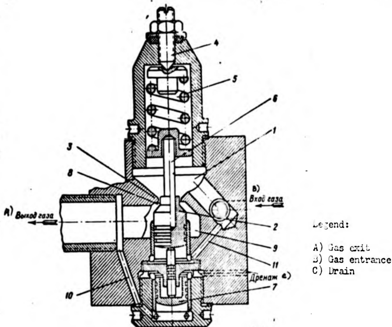
Figure 167. The direct action reducer.
