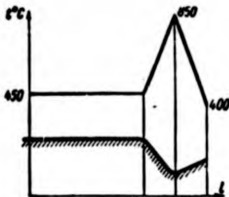
Figure 101. Approximate distribution of T through the length of the chamber for a steel wall.
