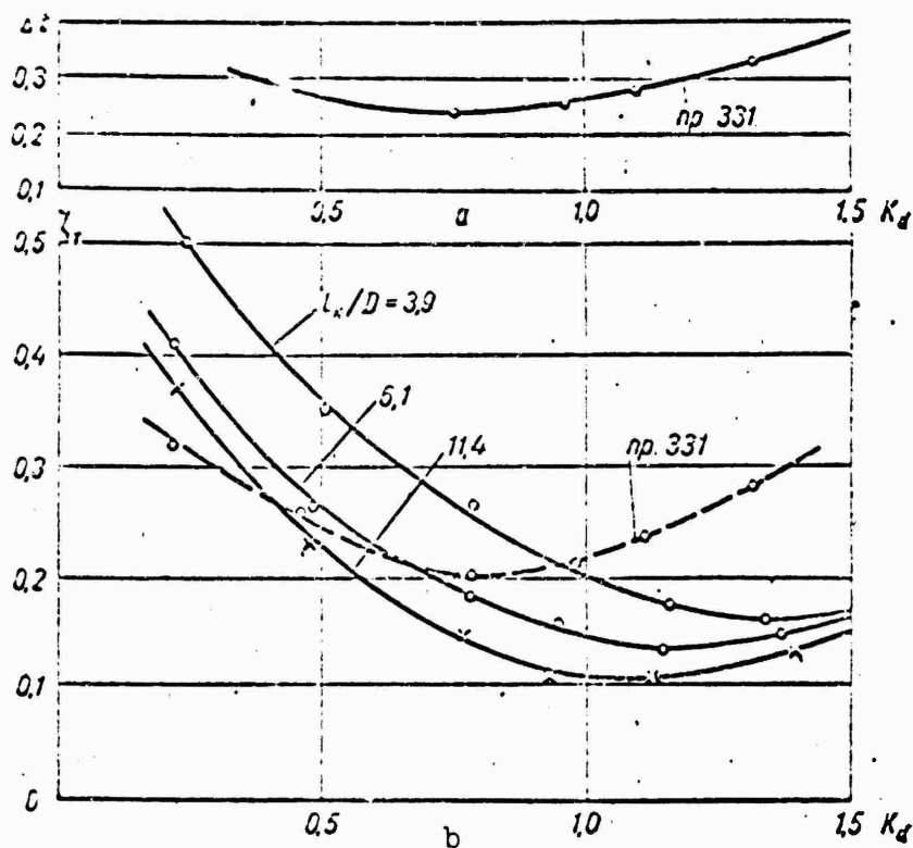
Figure 8. The \zeta_T = f(K_d) magnitude of various alternate shapes of suction part of water duct.
