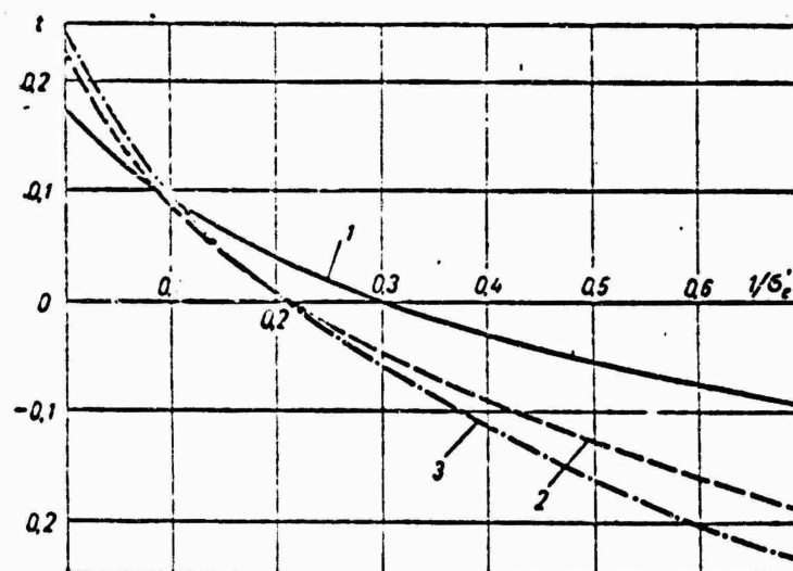
Figure 5. Effect of transversal opening b/D and angle \beta on suction factor t ( h/T > 7 ; T_B/D = 1 ). 1, l_k/D = 5.5 ;
