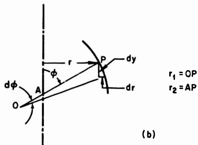
Fig. 1 Notation for a Shell of Revolution
