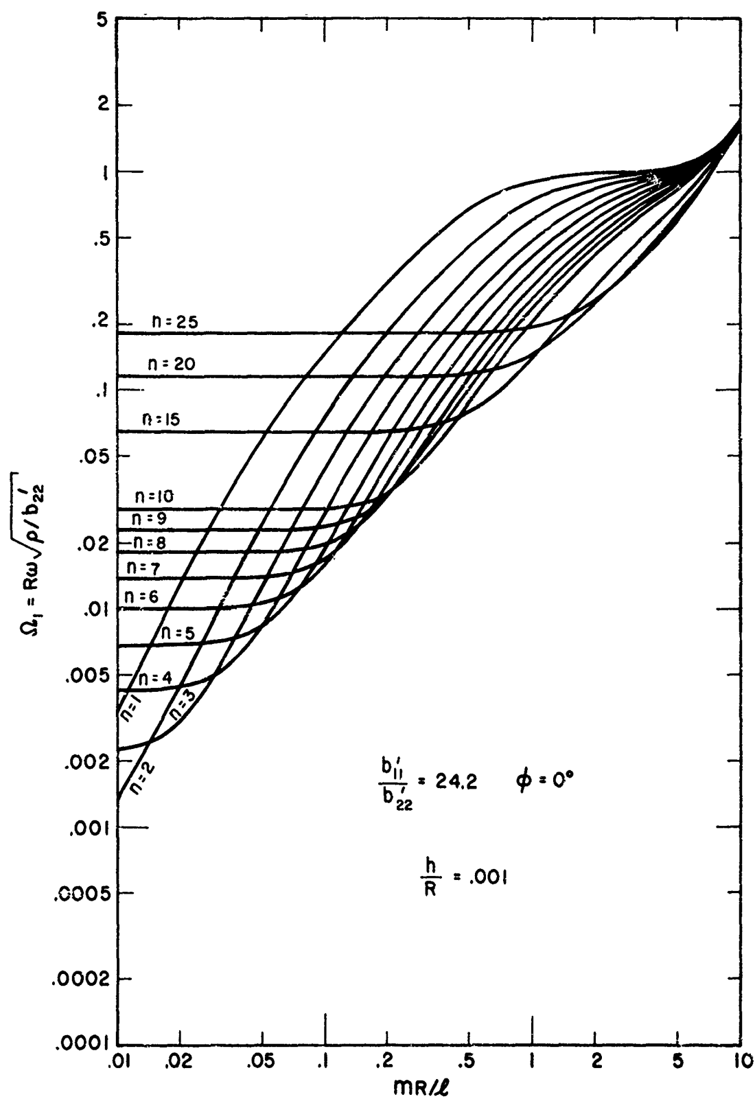
FIG. 13 FREQUENCIES OF n \geq 1 MODES FOR AXIAL STIFFENING - CONSTANT THICKNESS ORTHOTROPIC CYLINDER
