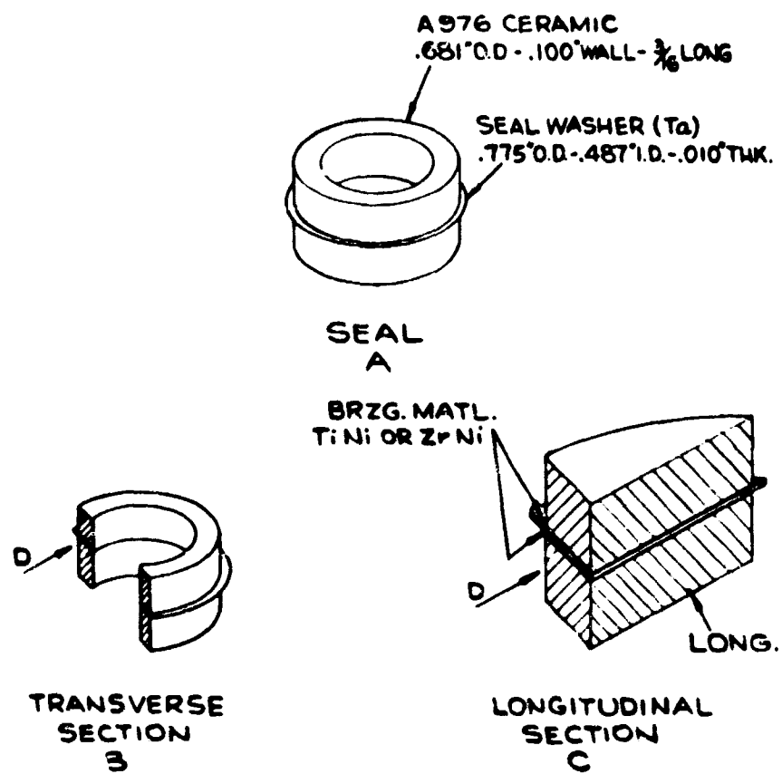
Figure 16 - Metal-to-ceramic seal test sample
