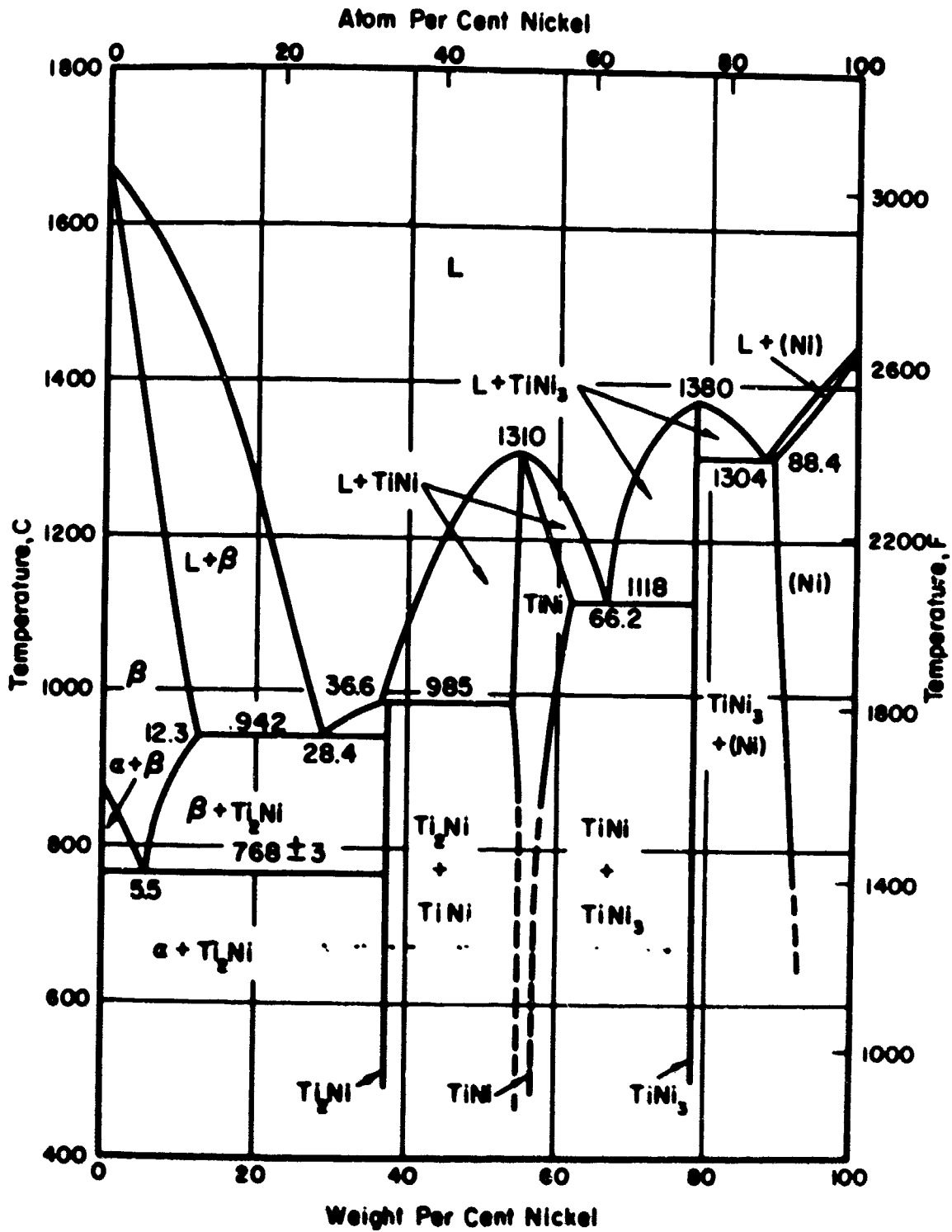
Figure 5 - Titanium-nickel phase diagram 11
