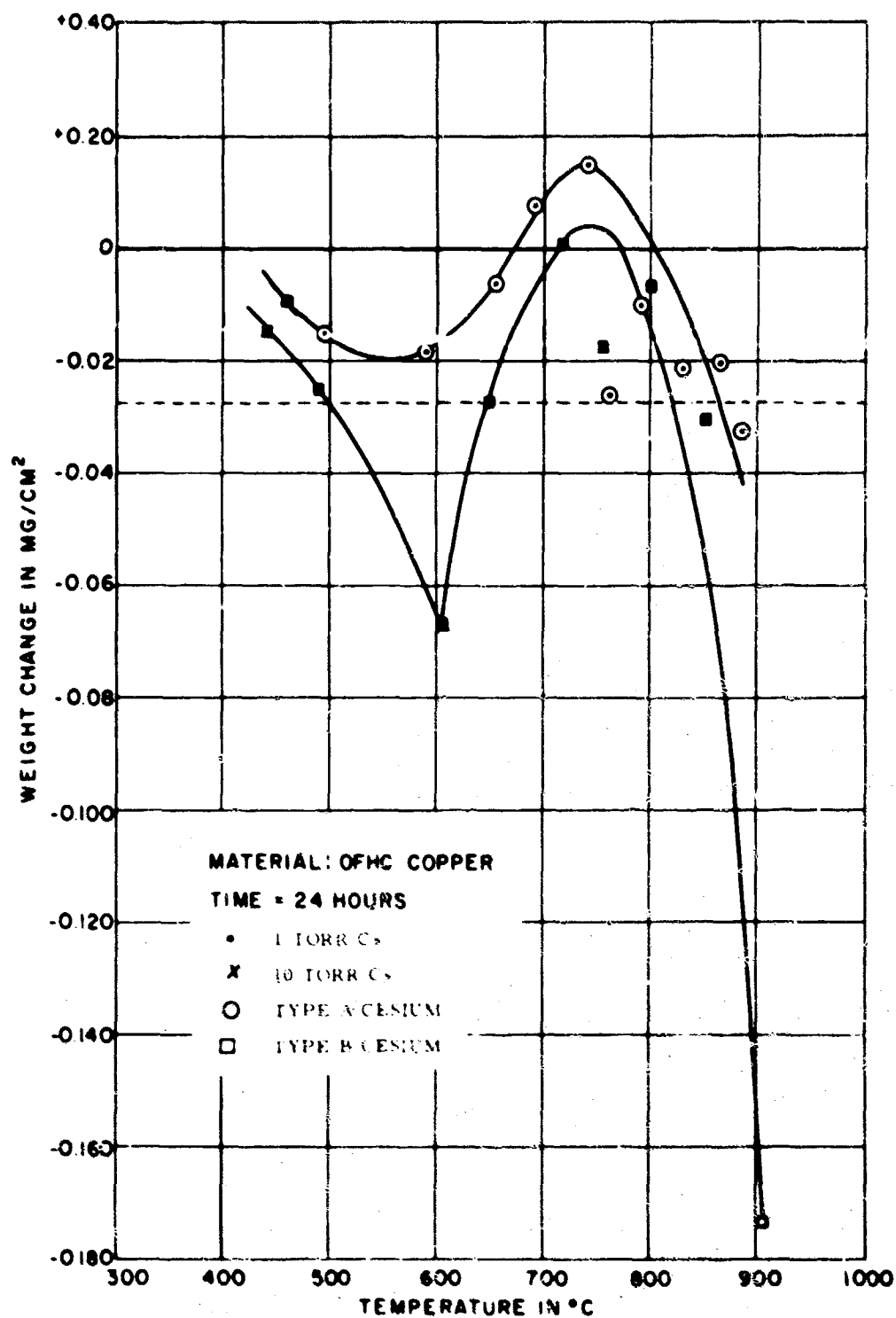
Figure 38 - Weight change in mg/cm 2 versus temperature for OFHC copper
