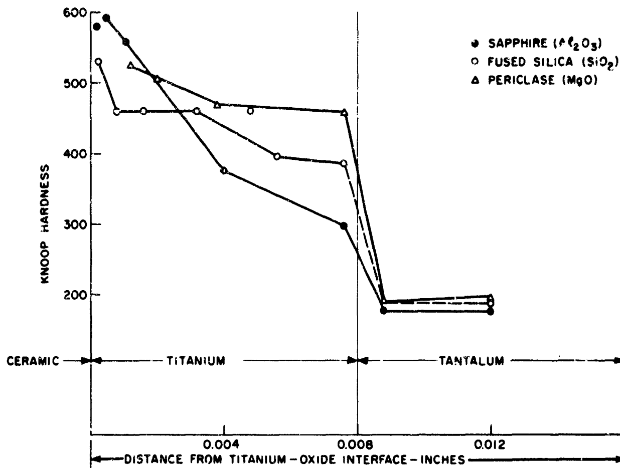
Figure 15 - Knoop hardness transverse across selected titanium-metal oxide seals
