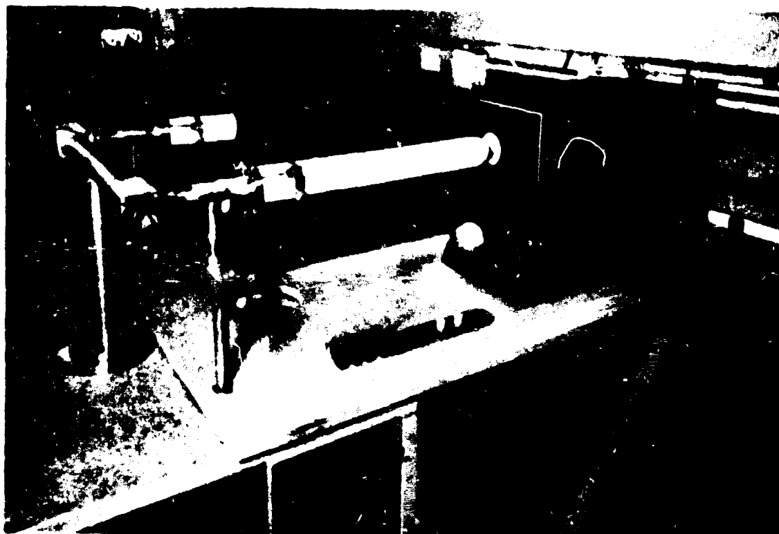
Figure 4 - High-temperature vacuum life test station
