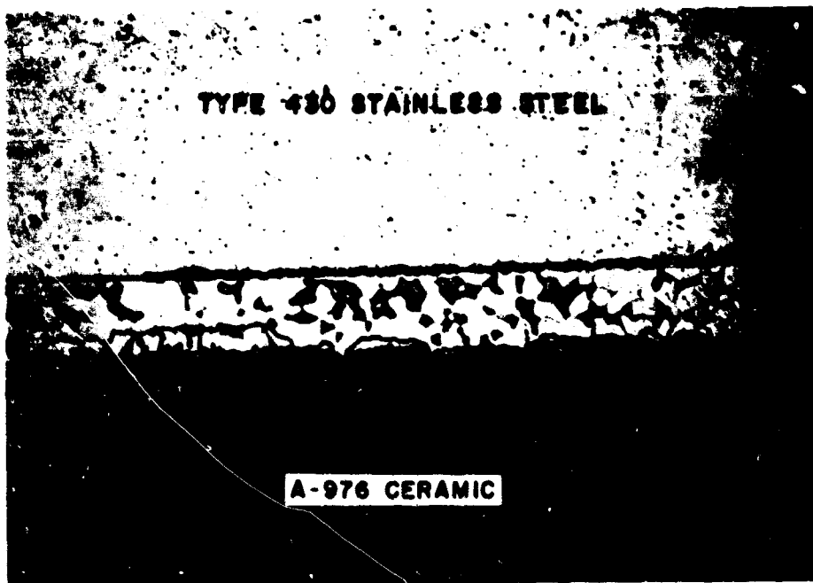
Figure 19 - Photomicrograph of ceramic-to-Type 430 stainless-steel seal, 500 X
