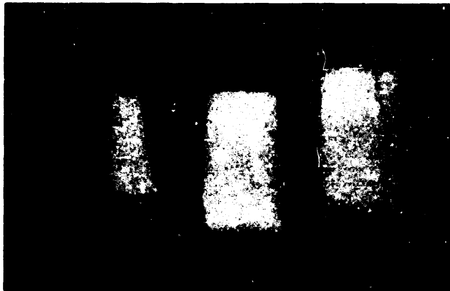
Figure 14 - Cross-sections of Ta-(ZrNi)-97 percent alumina metal-ceramic seals after 24 hours, 15 hours, and 6 hours (left to right) at 800°C in 1 Torr of cesium vapor, 16 X
