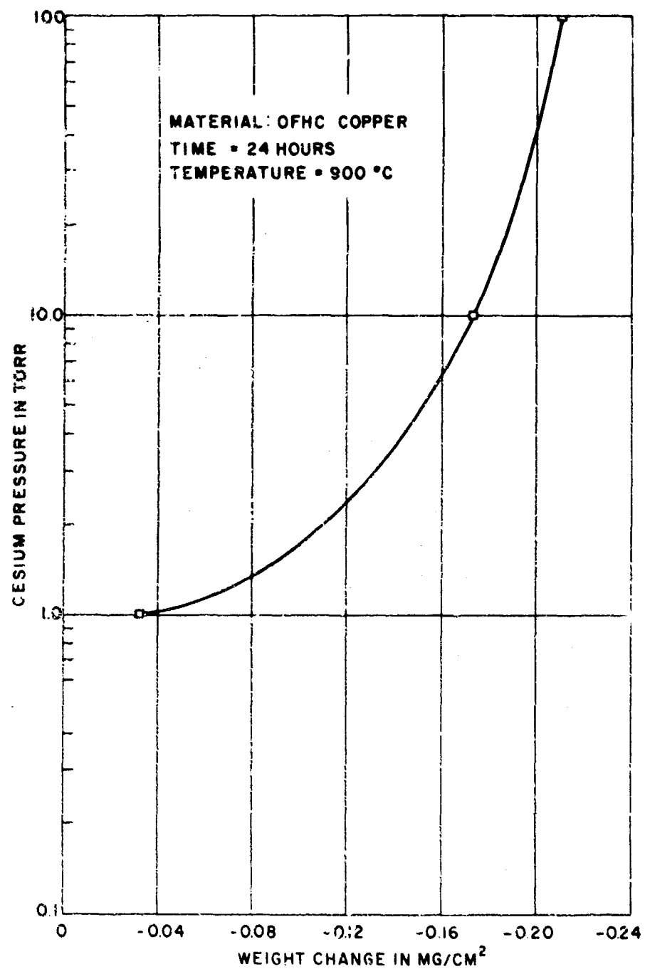
Figure 41 - Weight change in \text{mg}/\text{cm}^2 versus cesium pressure for OFHC copper
