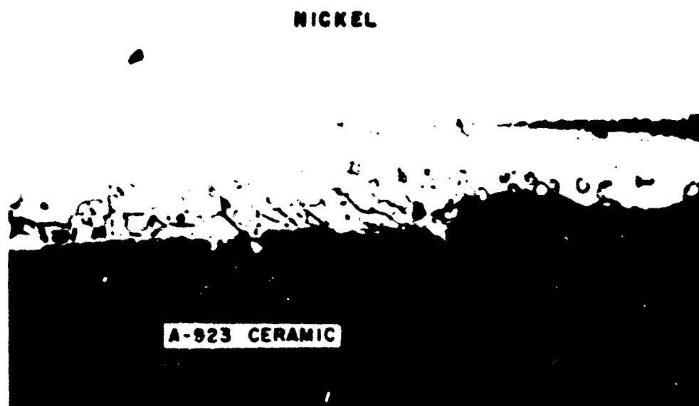
Figure 30 - Photomicrograph of ceramic-to-nickel seal heated for four minutes at a temperature of 1090^{\circ}\text{C} showing crack through \text{TiNi}_3 zone, 500 X
