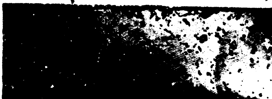
Figure 20 - Photomicrograph of seal sample Z-3B, transverse section, after 144 hours at 900°C in 1 Torr of cesium vapor, 100 X
