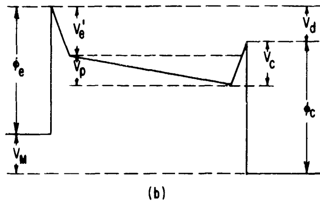
Figure 6 - Electron potential diagrams illustrating the simplified model used for the breakdown (a) and the maintenance (b) processes
