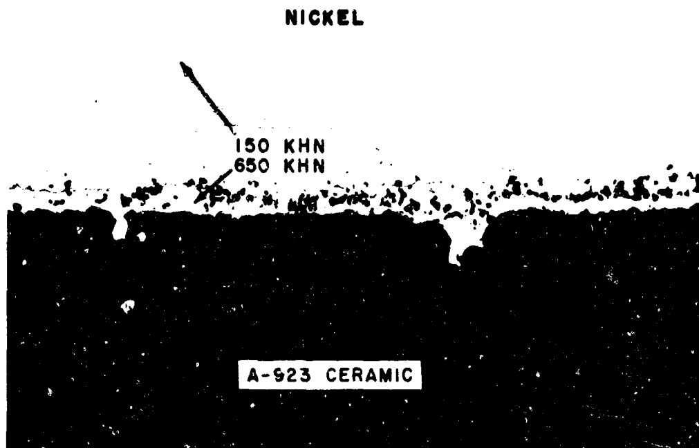
Figure 35 - Photomicrograph of ceramic-to-nickel seal after 480 hours at a temperature of 900^{\circ}\text{C} , 750 X
