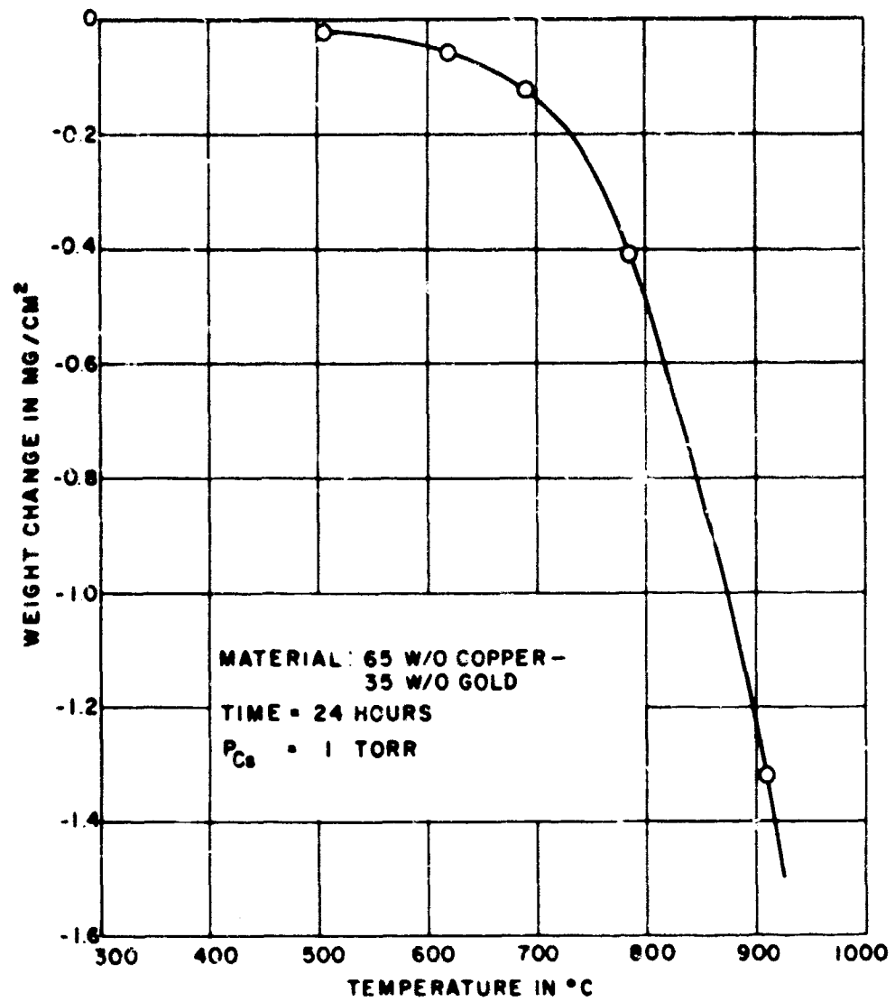
Figure 39 - Weight change in mg/cm 2 versus temperature for 65 w/o copper-35 w/o gold alloy
