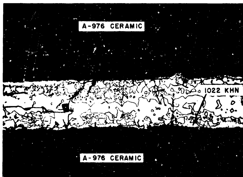
Figure 36 - Photomicrograph of seal shown in Figure 33 after 1680 hours at a temperature of 700^{\circ}\text{C} , 500 X
