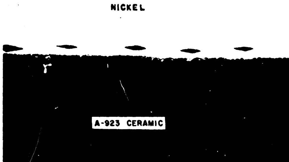
Figure 29 - Photomicrograph of ceramic-to-nickel seal made at a temperature of 1315^{\circ}\text{C} , 500 X
