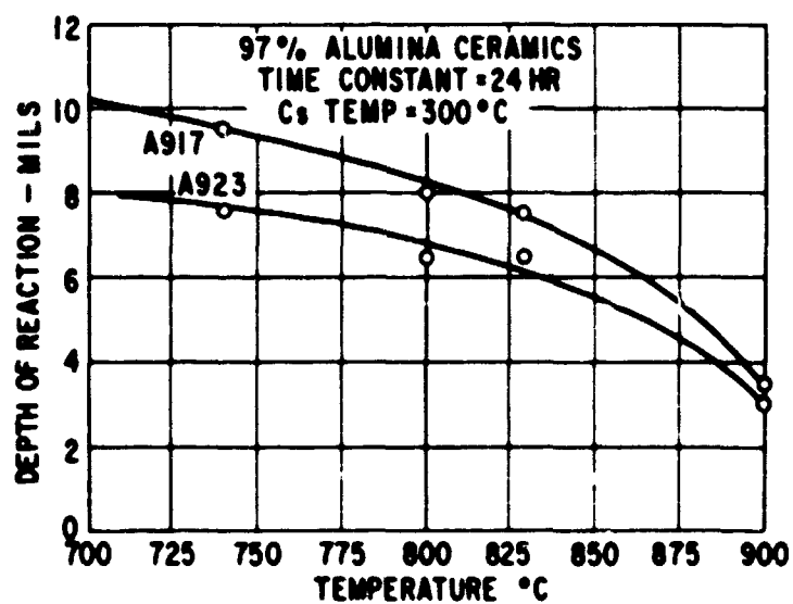
Figure 10 - Depth of reaction in 24 hours versus temperature for two 97 percent alumina ceramics
