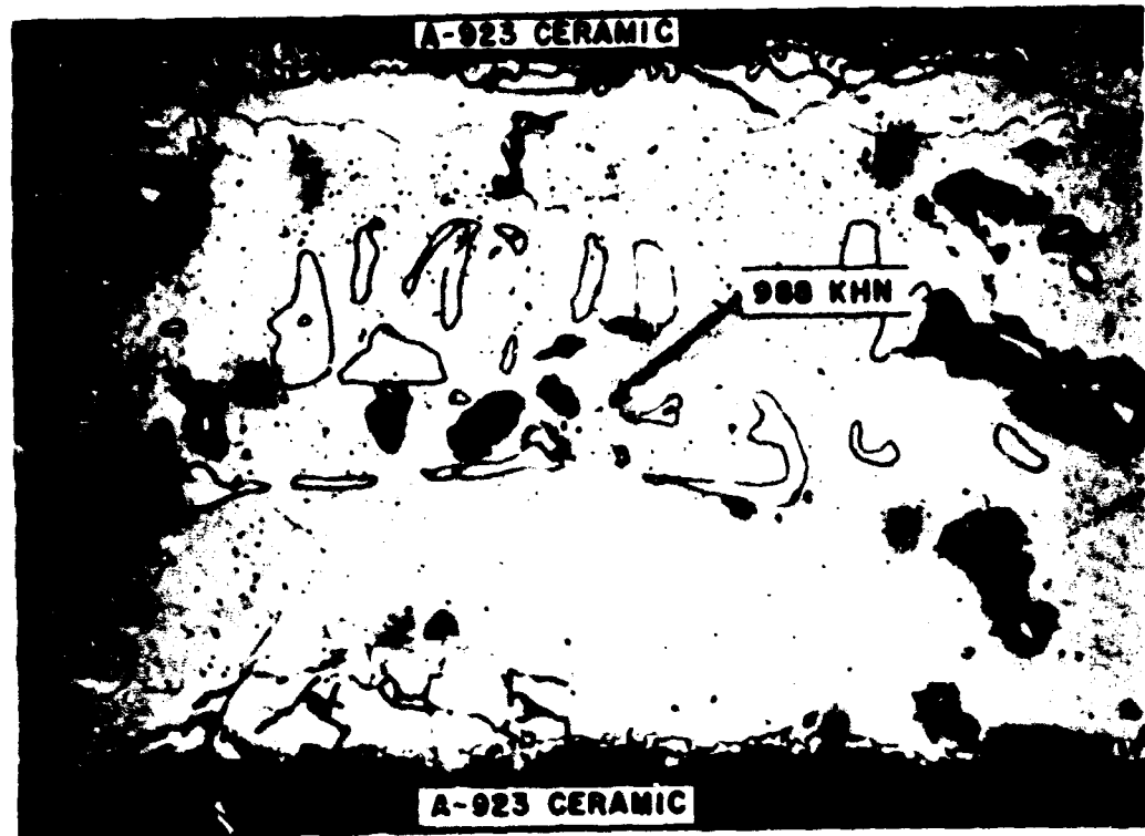
Figure 31 - Photomicrograph of wrapped ceramic-to-titanium seal after 240 hours at a temperature of 900^{\circ}\text{C} , 500 X
