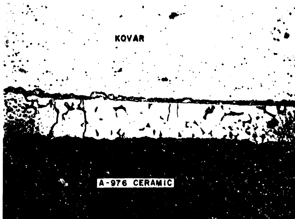
Figure 17 - Photomicrograph of ceramic-to-Kovar seal, 500 X
