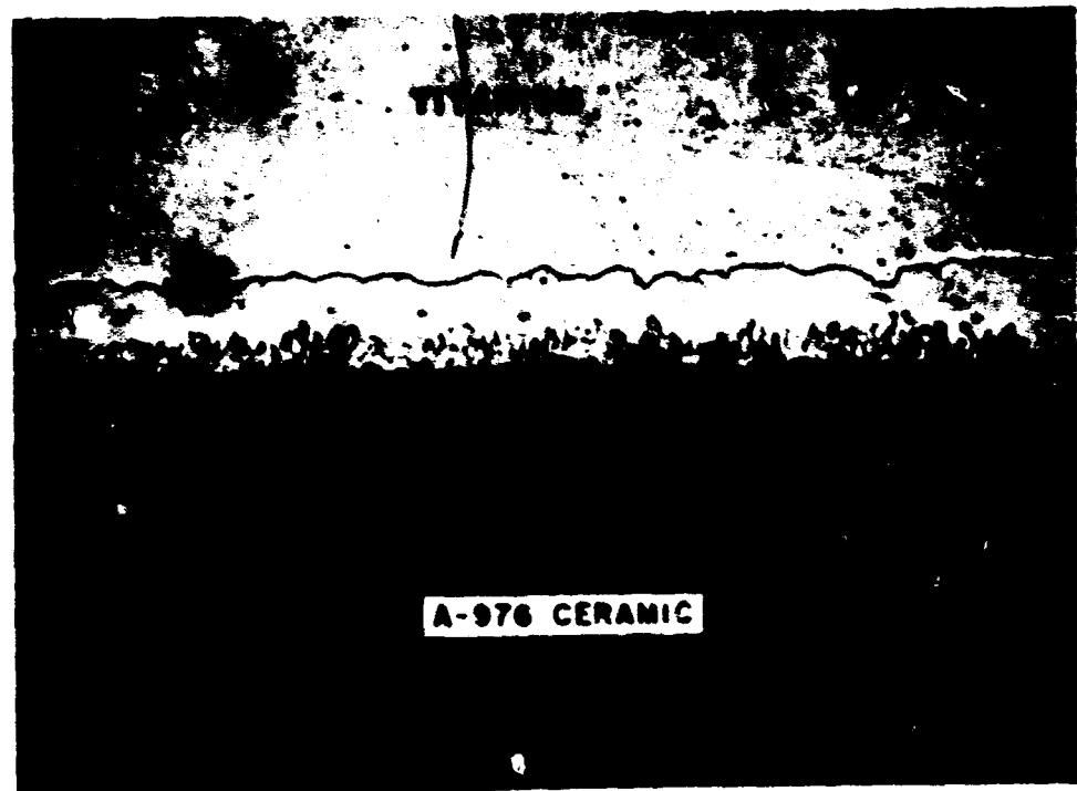
Figure 32 - Photomicrograph of ceramic-titanium "reaction" specimen after 240 hours at a temperature of 900^{\circ}\text{C} , 500 X
