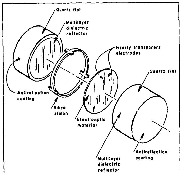
FIG. 8. Exploded View of Modified Electrooptic Laser Modulator.
