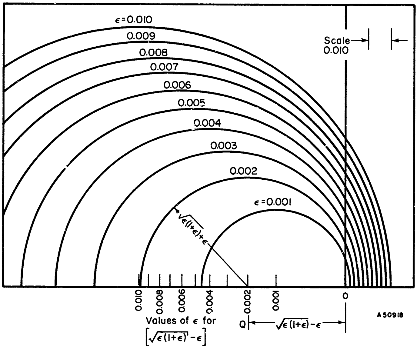
FIGURE 6. NOMOGRAM NUMBER TWO BATTELLE MEMORIAL INSTITUTE
