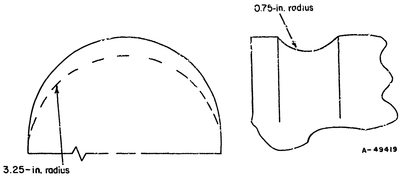
FIGURE 33. HOOK GEOMETRY
