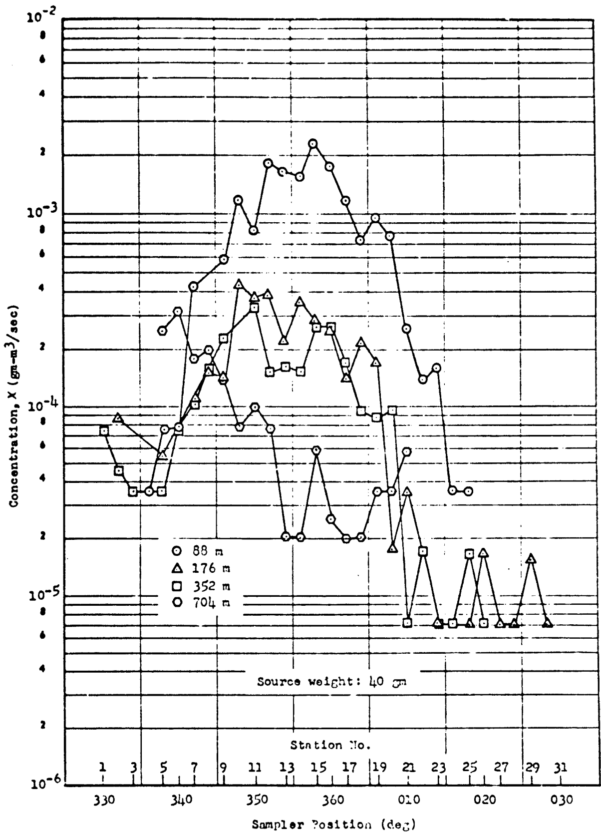
Figure 18 Arc Profiles of Uranine Samples Collected under Mild Lapse for Test 1
