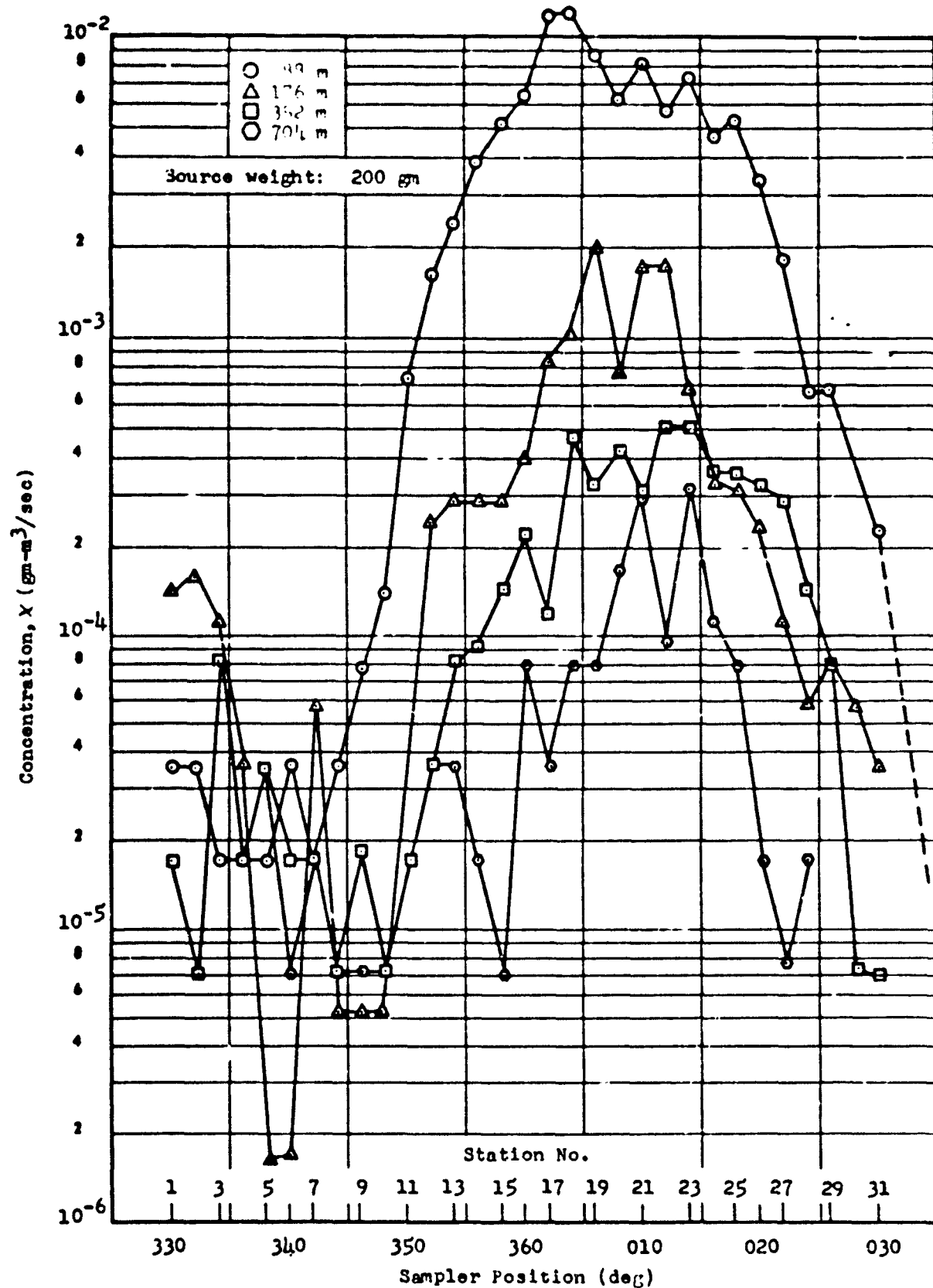
Figure 20 Arc Profiles of Uranine Samples Collected under Mild Lapse for Test 3
