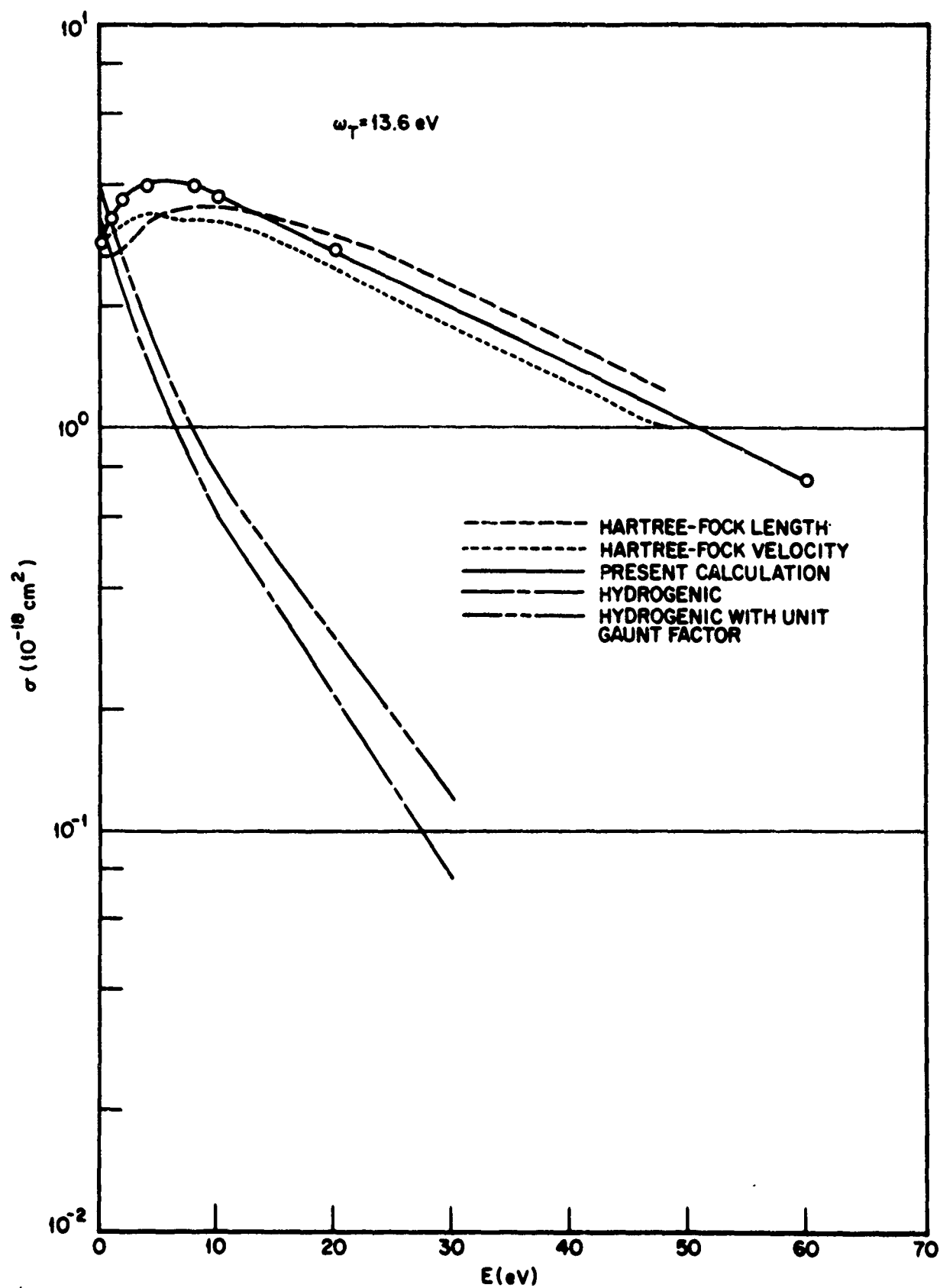
Fig. V-1 Comparison of photoionization cross section obtained with Hartree-Fock calculations of Ref. 100 and those obtained with Eq. (5.22) – OI: 2s^2 2p^4 ({}^3P) \rightarrow 2s^2 2p^3 ({}^4S)\epsilon
