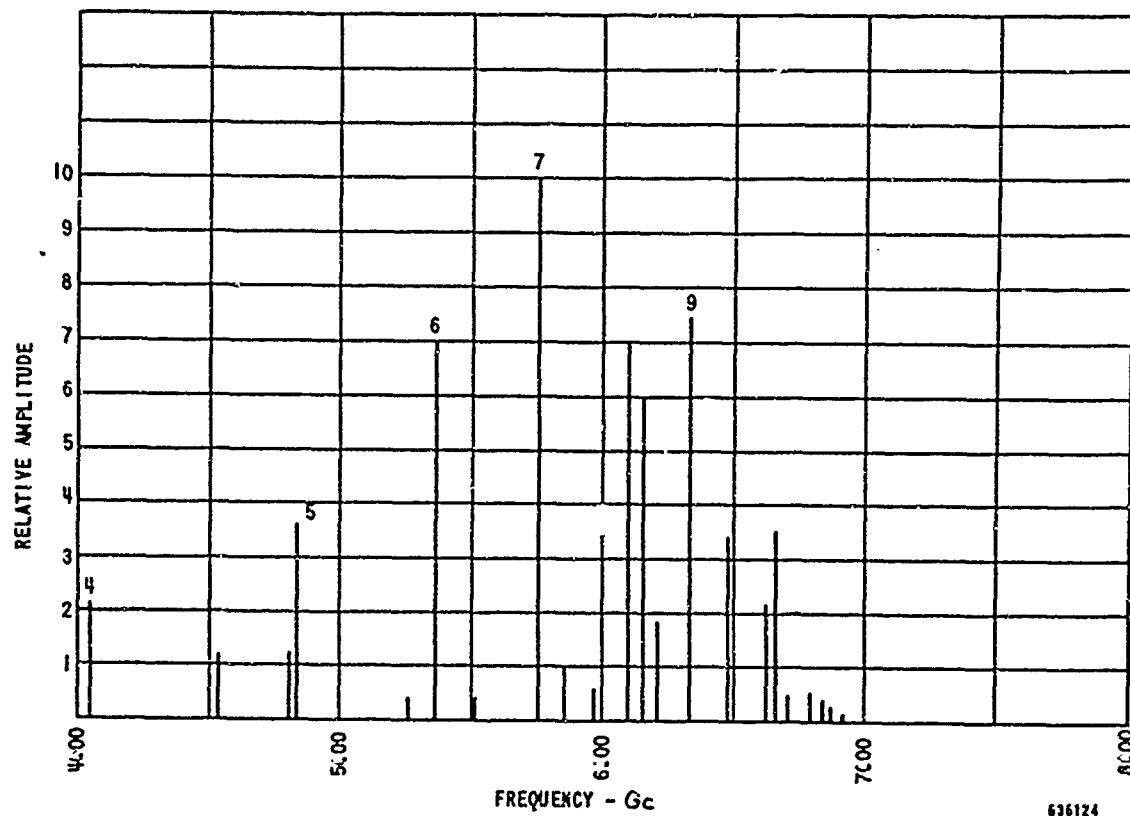
Figure 23 Relative Amplitude of Lower Order Modes With Cathode Ring
