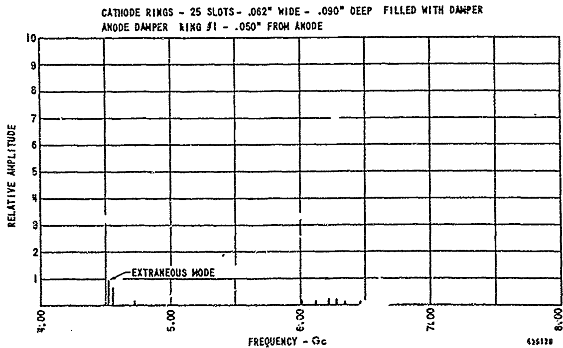
Figure 28 Suppression of Lower Order Modes With Cathode and Anode Dampers
