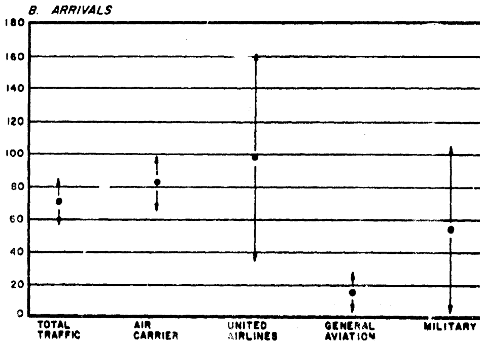
FIGURE 11. COMPOSITE OF DELAY
