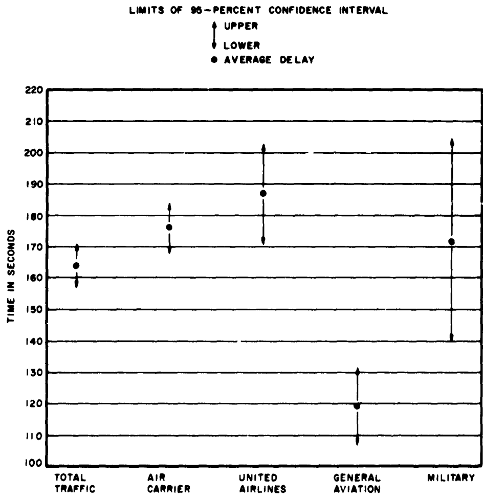
FIGURE 12. OVERALL COMPOSITE OF DELAY
