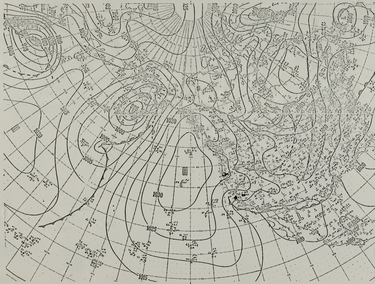
Fig. 19b. Surface Weather Map 1230Z 8 December 1943.
