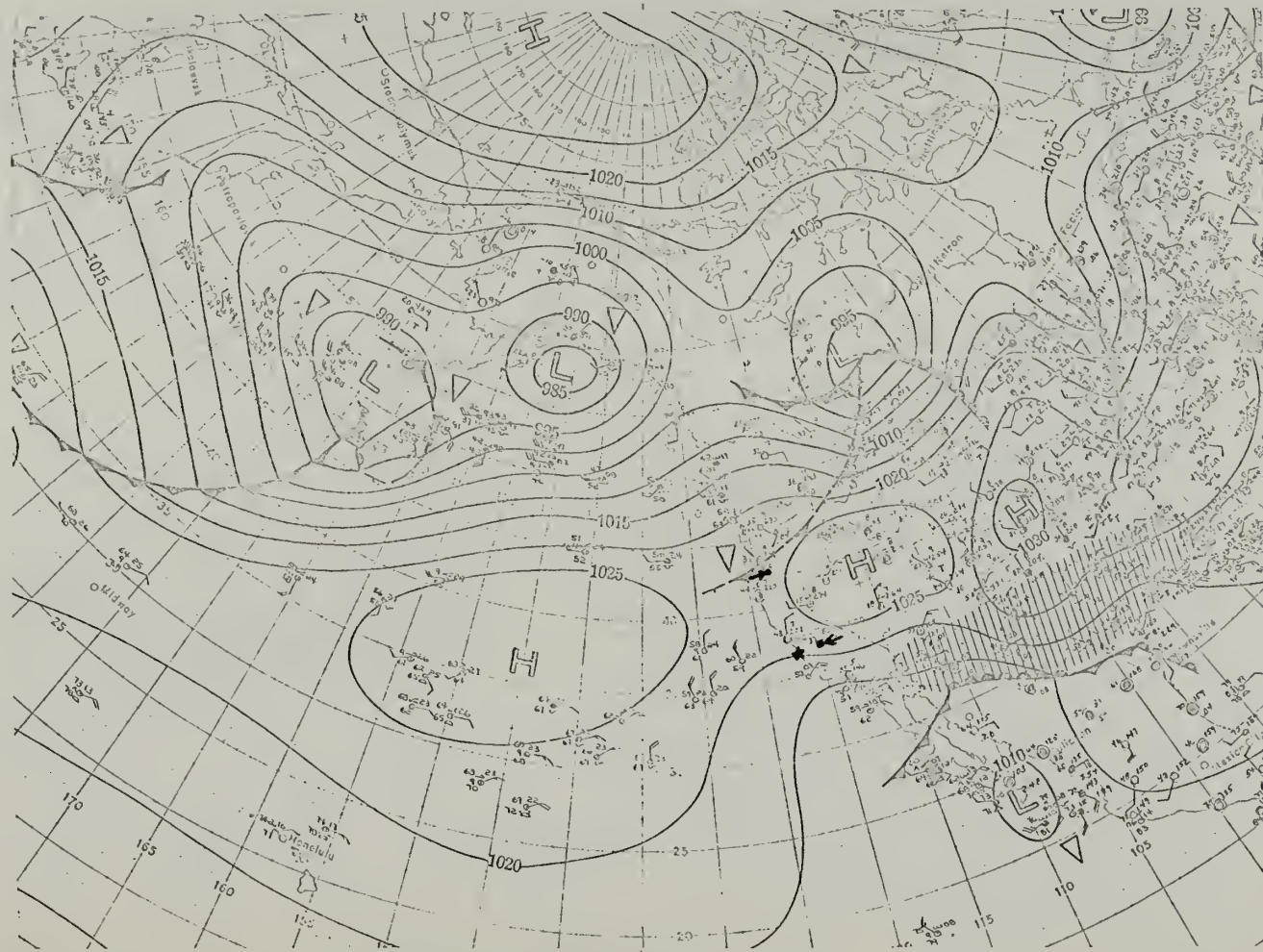
Fig. 23e. Surface Weather Map 1200Z 2 December 1923.
