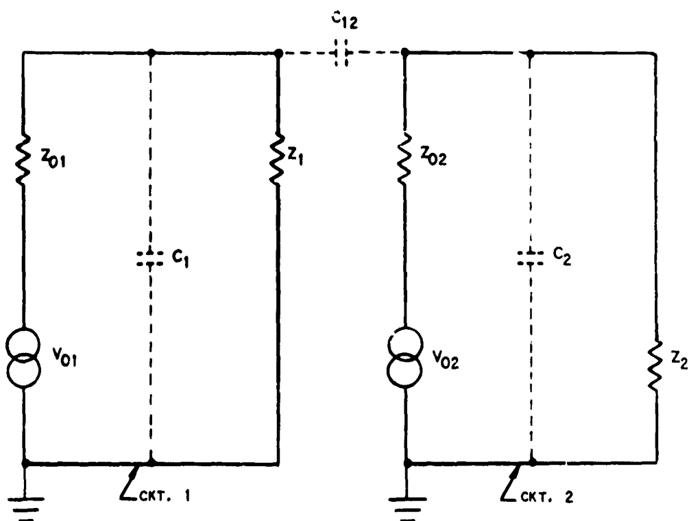
Figure 2-100. Capacitively-Coupled Circuits
