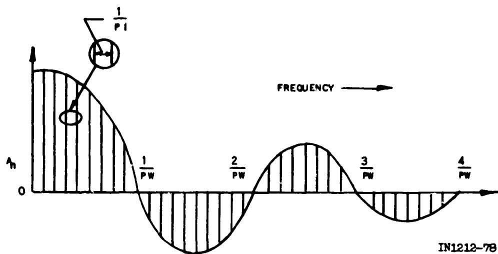
Figure 1-6. Doubling the Pulse Repetition Rate of Figure 1-5 Plot (Spacing Between Harmonics Doubled and Amplitude of Harmonics Increased)
