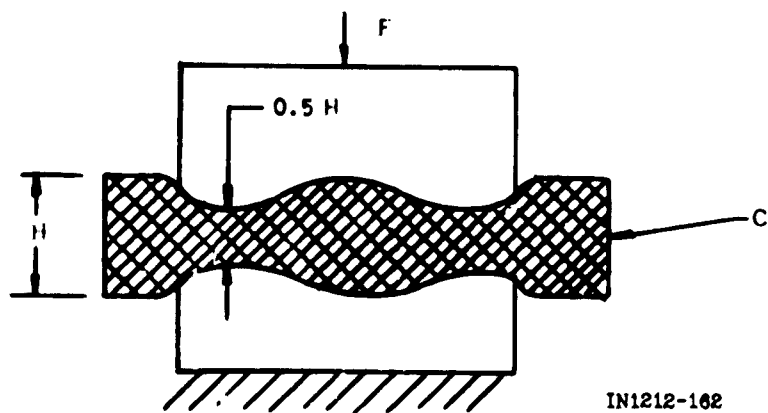
Figure 2-70. Gasket C in Simulated Joint
