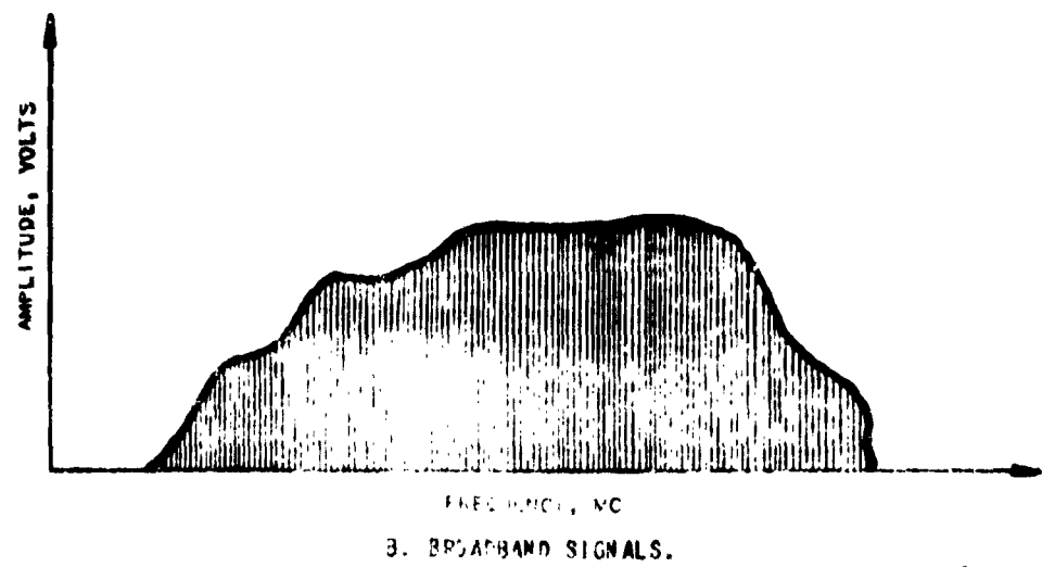
Figure 1-1. Interference Signals
