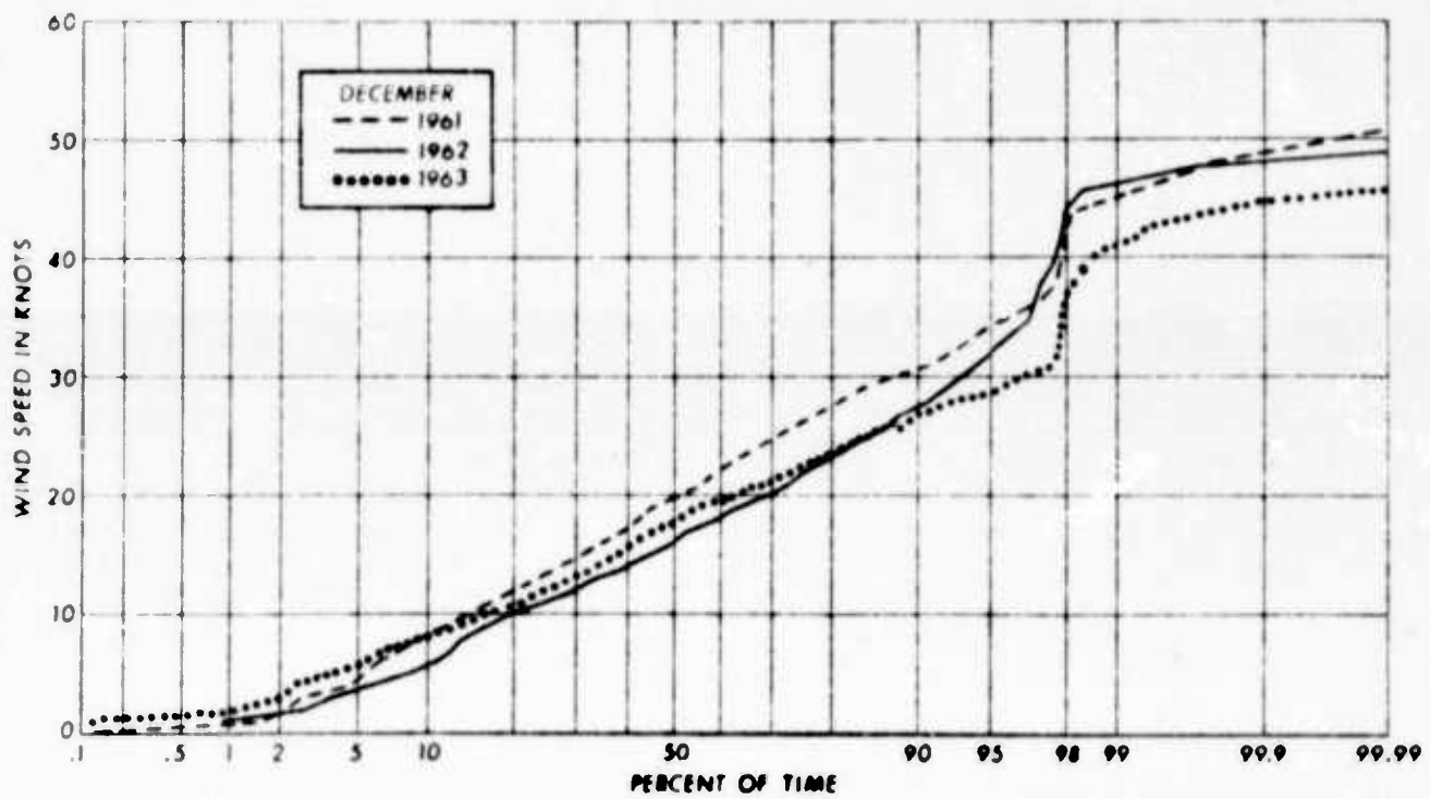
Fig. 8 (Cont'd) - Cumulative Wind-Speed Distributions
