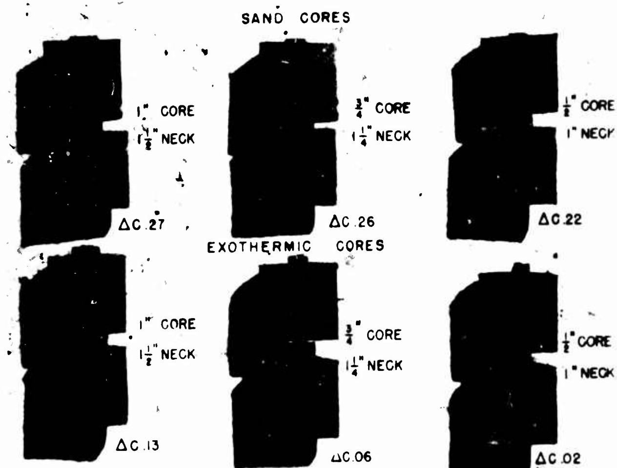
Fig. 12 - Sectioned casting showing how segregation can be reduced by the use of exothermic cores
