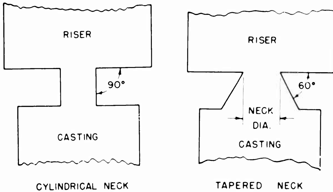
Fig. 1 - Contact neck types used on experimental castings
