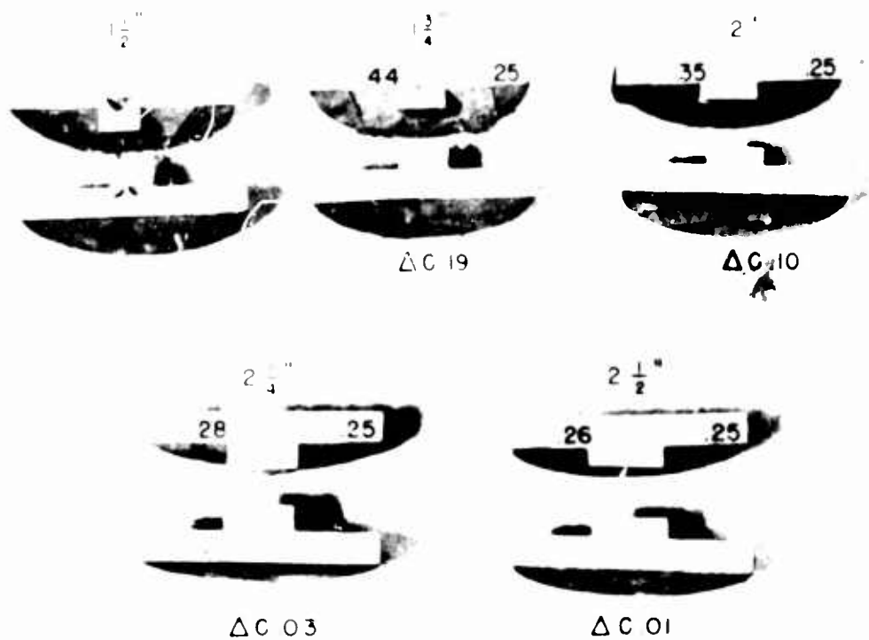
Fig. 19 - Degree of segregation for a given size and shape of casting with varying diameters of cylindrical neck. Carbon contents and neck diameters as indicated. Fixed casting dimensions: Diameter, 8" - Height, 1" - Neck Length, 1\frac{1}{2} "
