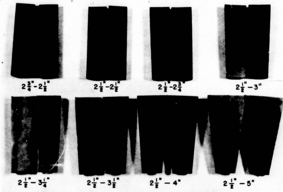
Fig. 41 - Sectioned and etched tapered castings ten inches long, bottom-gated, and with bottom and top diameters as indicated, showing how shrinkage and segregation are influenced by taper
