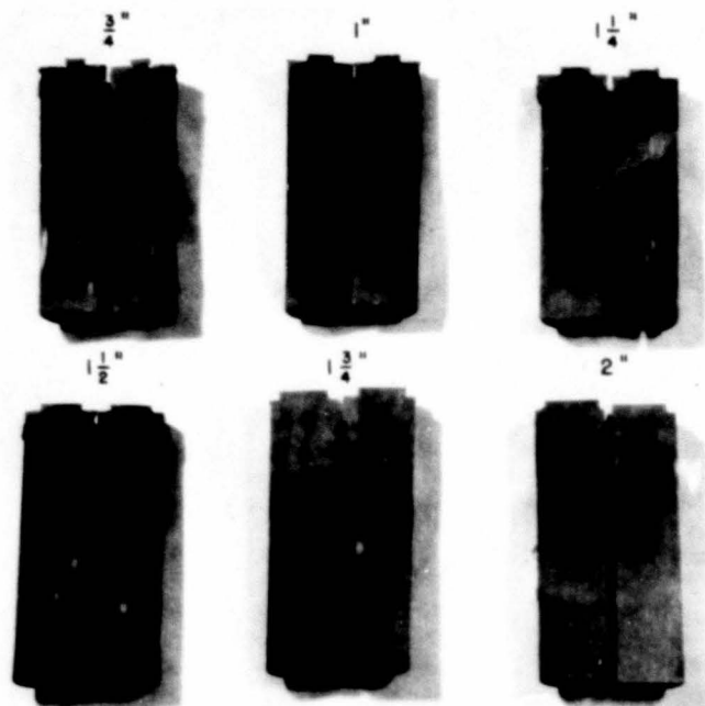
Fig. 35 - Degree of segregation for a given size and shape of top-gated casting with varying diameters of cylindrical neck. Neck diameters as indicated. Fixed casting dimensions: Diameter, 2\frac{1}{2} " - Height, 10" - Neck Length, \frac{3}{4} "
