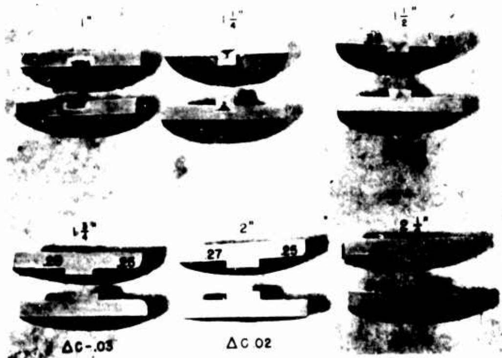
Fig. 18 - Degree of segregation for a given size and shape of casting with varying diameters of cylindrical neck. Carbon contents and neck diameters as indicated. Fixed casting dimensions: Diameter, 8" - Height, 1" - Neck Length, 1"
