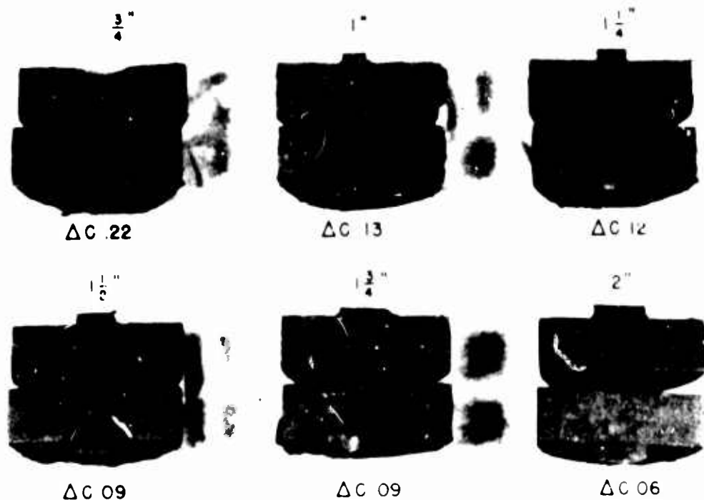
Fig. 21 - Degree of segregation for a given size and shape of casting with varying diameters of cylindrical neck. Carbon contents and neck diameters as indicated. Fixed casting dimensions: Diameter, 6" - Height, 2" - Neck Length, \frac{3}{4} "
