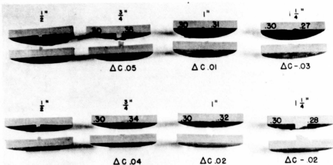
Fig. 33 - Degree of segregation for a given size and shape of casting with varying diameters of cylindrical neck. Carbon contents and neck diameters as indicated. Castings in bottom row gated over core. Fixed casting dimensions: Diameter 8\frac{1}{4} " - Height, 1" - Neck Length, \frac{1}{2} " - Fixed riser dimensions: Diameter, 3\frac{1}{2} " - Height, 4"
