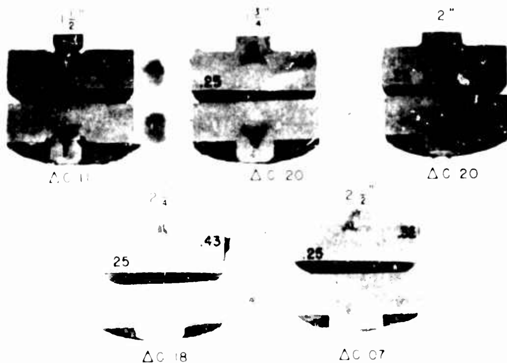
Fig. 23 - Degree of segregation for a given size and shape of casting with varying diameters of cylindrical neck. Carbon contents and neck diameters as indicated. Fixed casting dimensions: Diameter, 6" - Height, 2" - Neck Length, 1 1/4"
