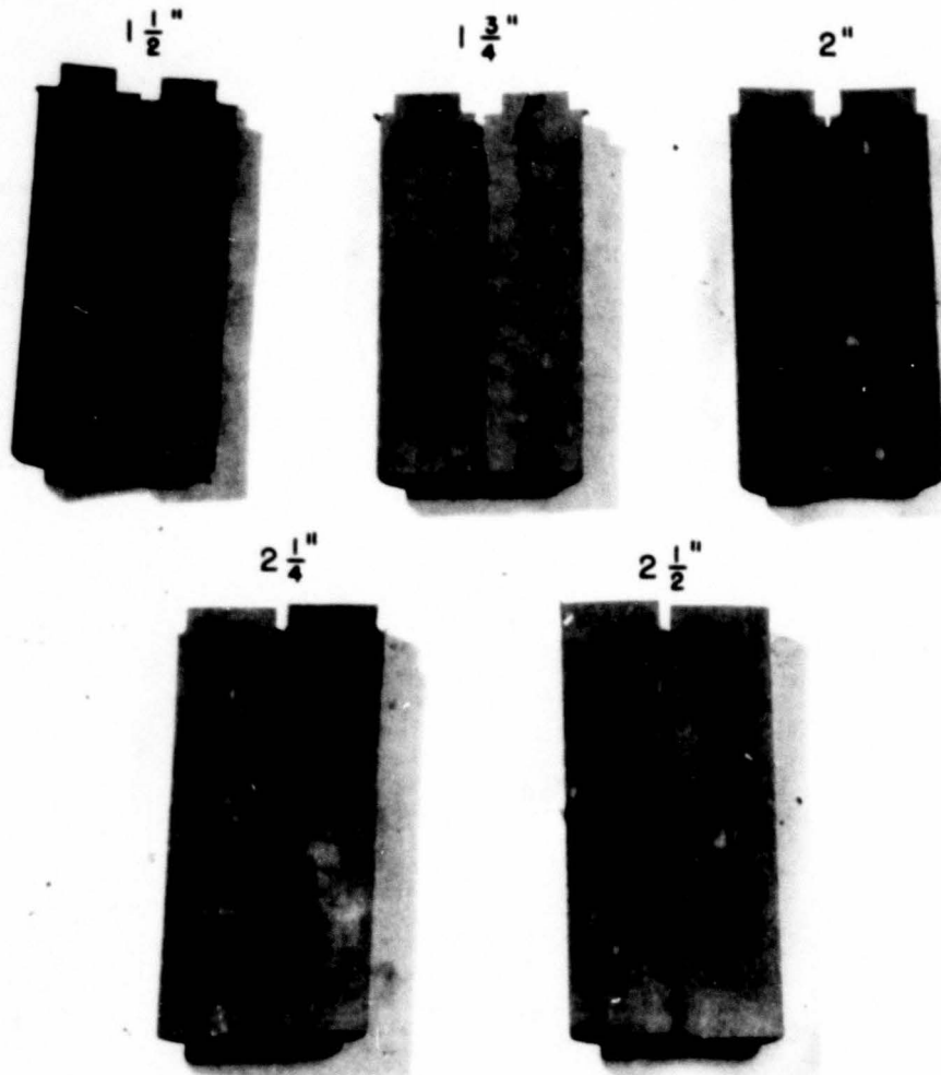
Fig. 37 - Degree of segregation for a given size and shape of top-gated casting with varying diameters of cylindrical neck. Neck diameters as indicated. Fixed casting dimensions: Diameter, 2\frac{1}{2} " - Height, 10" - Neck Length, 1\frac{1}{2} "
