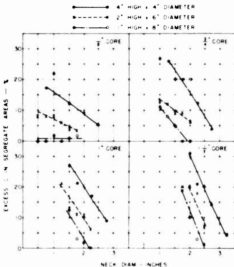
Fig. 32 - Relation between carbon segregation and neck diameter in castings of different thicknesses but of equal volumes. All castings fed by 5-inch-diameter riser
