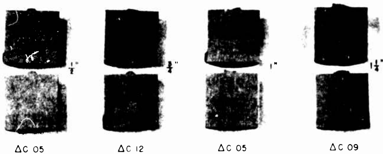
Fig. 15 - Sectioned and etched castings made with special core—neck diameters and carbon contents as indicated
