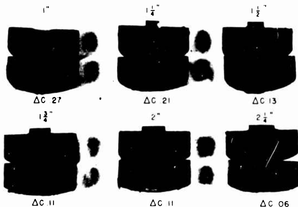
Fig. 22 - Degree of segregation for a given size and shape of casting with varying diameters of cylindrical neck. Carbon contents and neck diameters as indicated. Fixed casting dimensions: Diameter, 6" - Height, 2" - Neck Length, 1"
