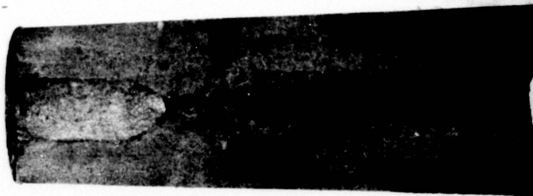
Fig. 39 - Section of a casting bled near the end of solidification
