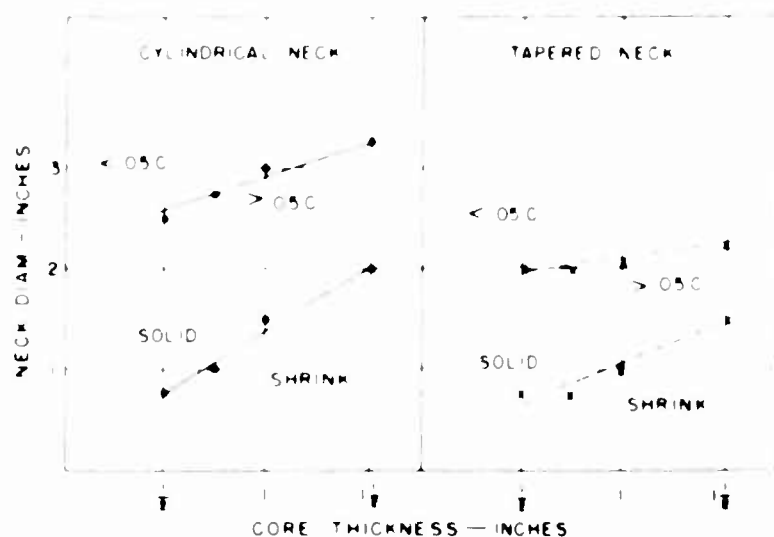
Fig. 11 - Relation of core thickness and neck diameter required on 4-inch-diameter cylinders to (1) produce sound castings and (2) keep segregation less than 0.05 percent carbon
