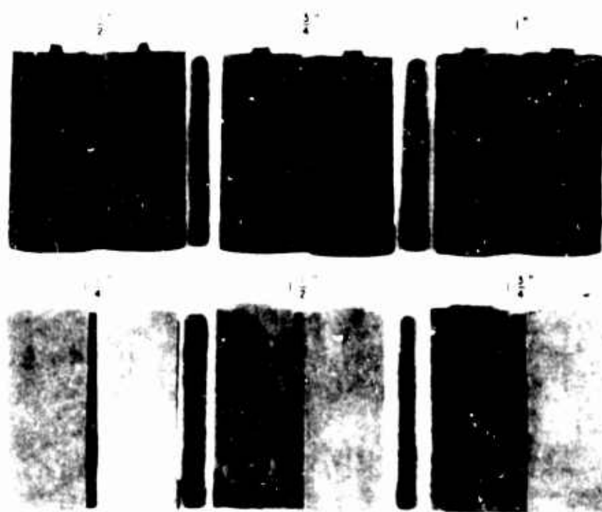
Fig. 24 - Degree of segregation for a given size and shape of casting with varying diameters of cylindrical neck. Neck diameters as indicated. Fixed casting dimensions: Diameter, 3" - Height, 7" - Neck Length, 1/2"
