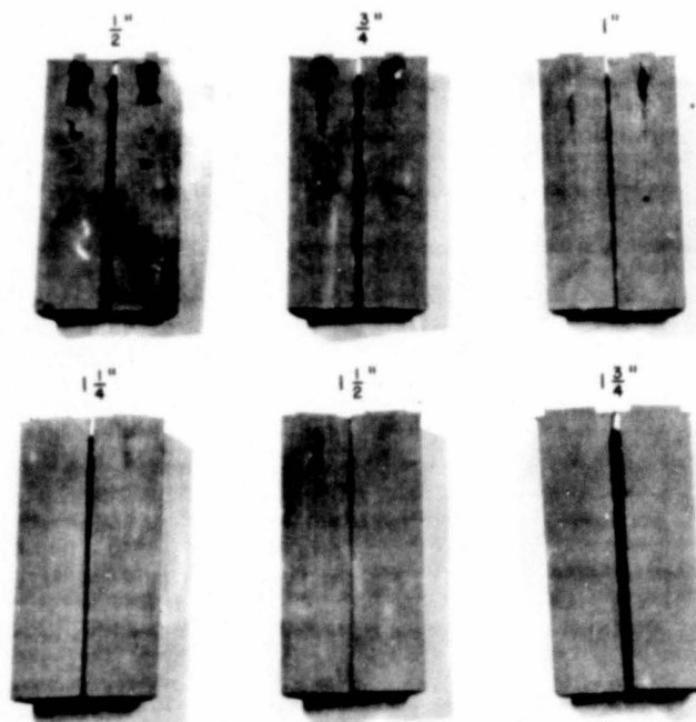
Fig. 34 - Degree of segregation for a given size and shape of top-gated casting with varying diameters of cylindrical neck. Neck diameters as indicated. Fixed casting dimensions: Diameter, 2\frac{1}{2} " - Height, 10" - Neck Length, \frac{1}{2} "
