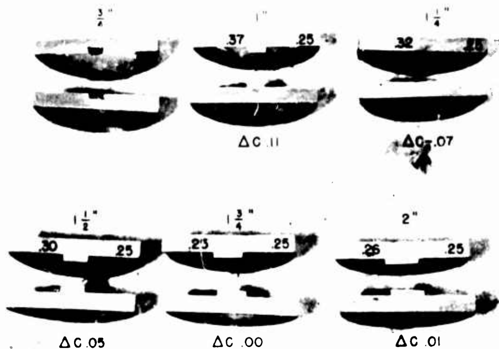
Fig. 17 - Degree of segregation for a given size and shape of casting with varying diameters of cylindrical neck. Carbon contents and neck diameters as indicated. Fixed casting dimensions: Diameter, 8" - Height, 1" - Neck Length, \frac{1}{4} "
