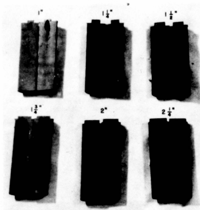
Fig. 36 - Degree of segregation for a given size and shape of top-gated casting with varying diameters of cylindrical neck. Neck diameters as indicated. Fixed casting dimensions: Diameter, 2\frac{1}{2} " - Height, 10" - Neck Length, 1"
