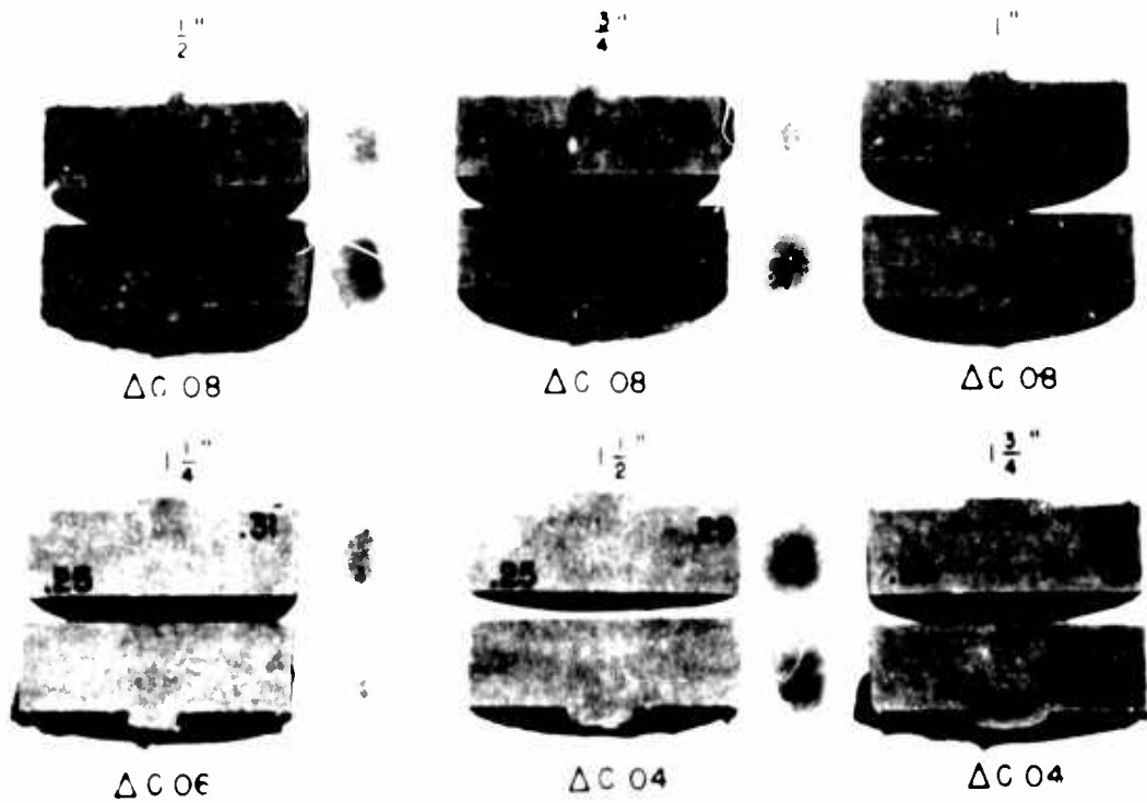
Fig. 20 - Degree of segregation for a given size and shape of casting with varying diameters of cylindrical neck. Carbon contents and neck diameters as indicated. Fixed casting dimensions: Diameter, 6" - Height, 2" - Neck Length, 1\frac{1}{2} "
