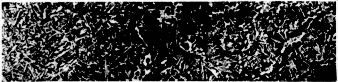
Fig. 38 - Photomicrograph through a V segregate (35x)
