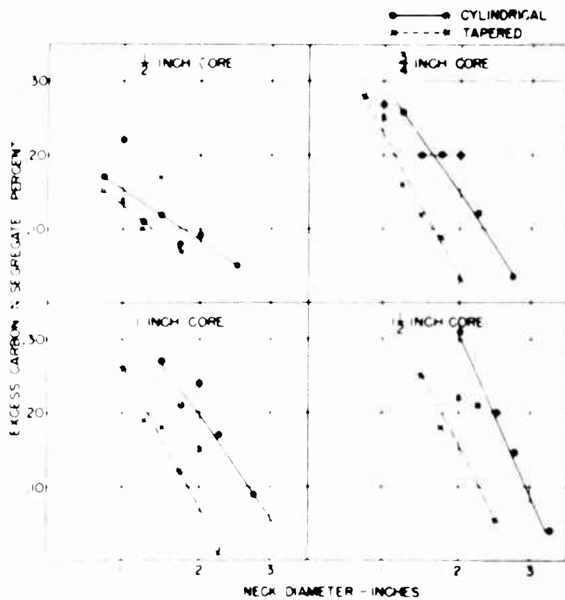
Fig. 10 - Relation of segregation to neck type, core thickness (neck length), and neck diameter in 4-inch-diameter cylinders
