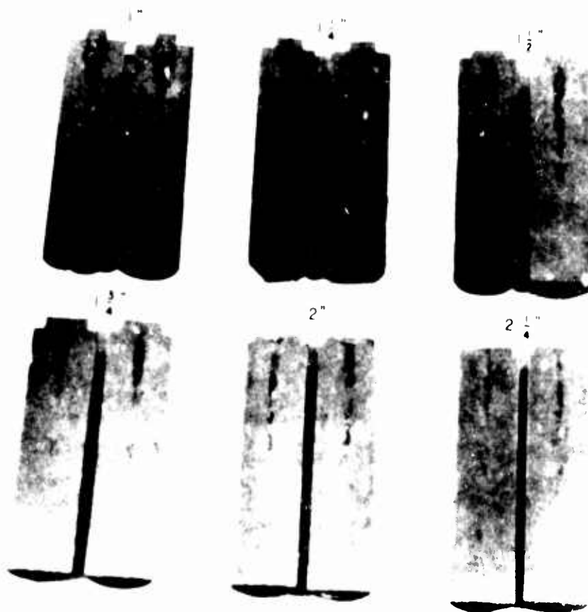
Fig. 30 - Degree of segregation for a given size and shape of casting with varying diameters of cylindrical neck. Neck diameters as indicated. Fixed casting dimensions: Diameter, 2" - Height, 10" - Neck Length, 1"
