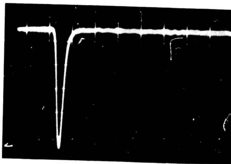
Fig. 24 Voltage Envelope of Backward-Wave Output Pulse as Seen with Tektronix 535 Oscilloscope, Model K "Plug In"
