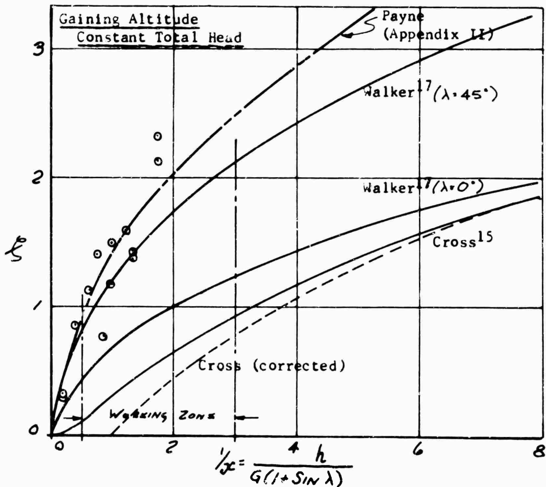
Figure 37. Comparison of Experimental Results with Different Estimates of the Damping Ratio " \xi ".
