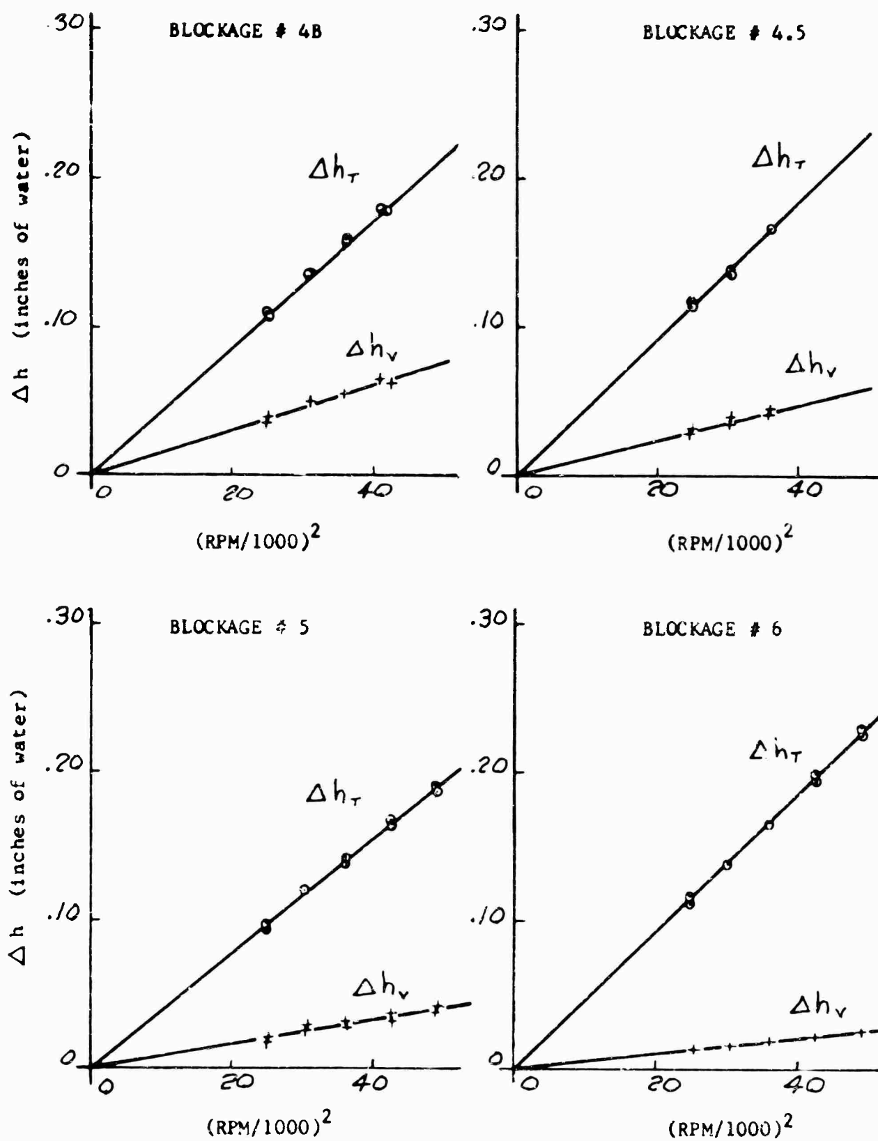
Figure 16. Duct System Calibration for Various Blockages.
