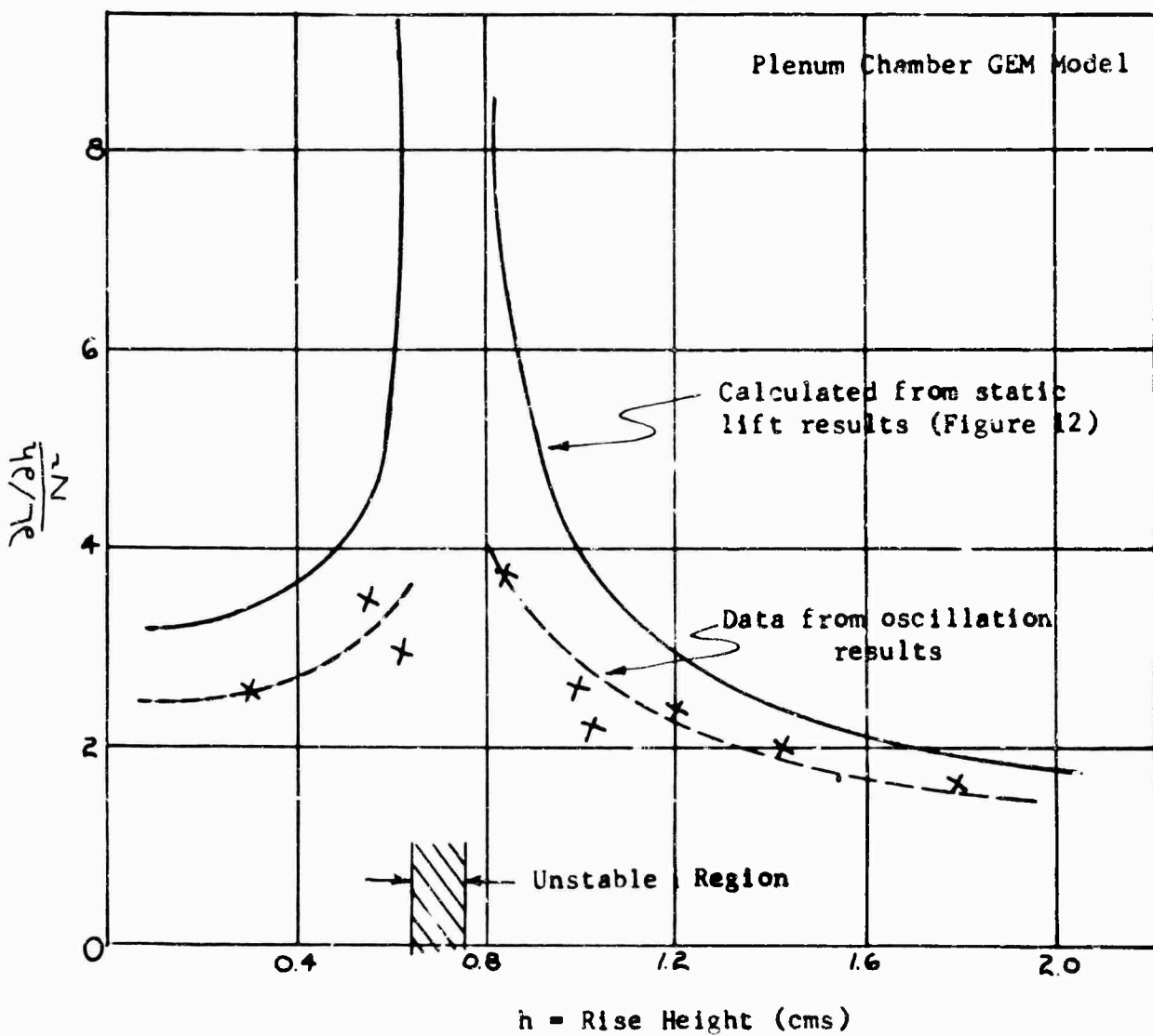
Figure 32. Comparison of Heave Stability Parameter \frac{\partial L}{\partial h} / N^2 as Determined From Oscillation Tests and Static Lift Measurements.
