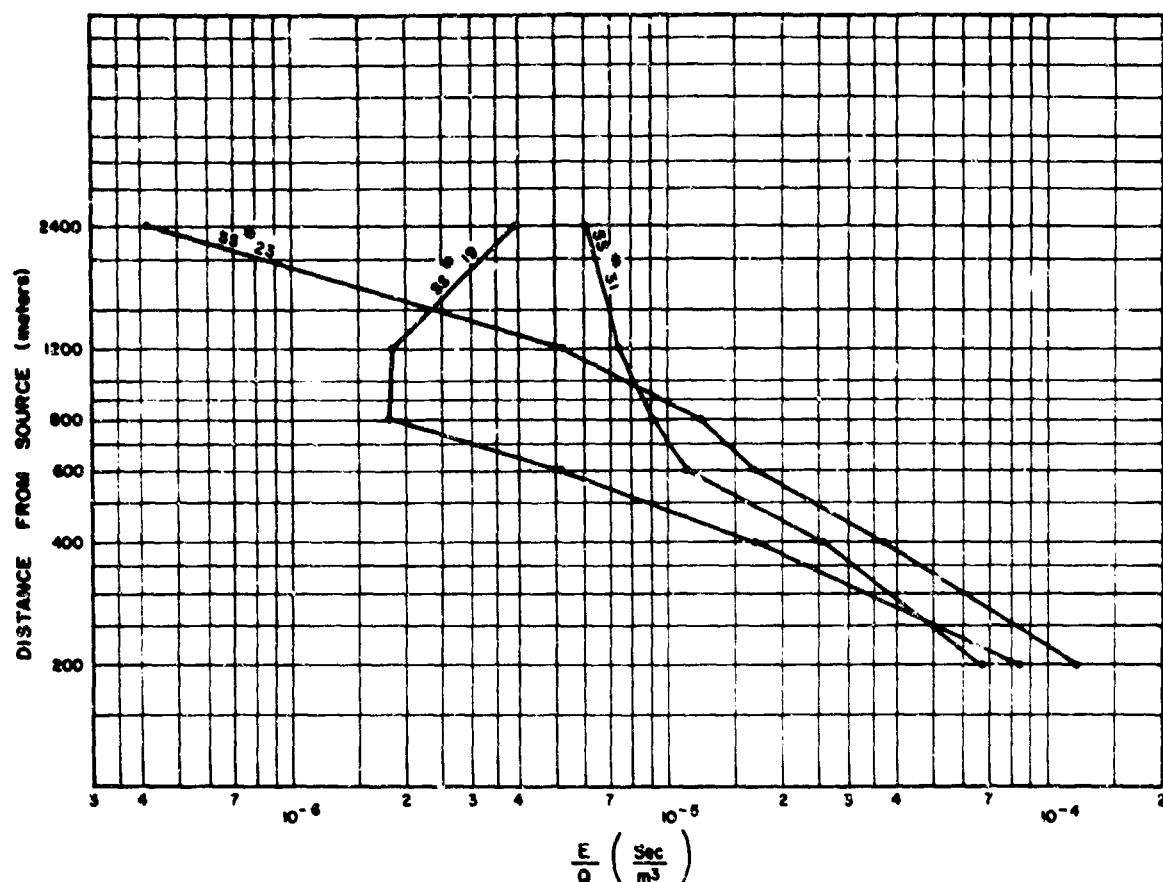
Figure 3. Downwind Distribution of Peak Dosages Normalized for Source Strength for Three Sand Storm Experiments Conducted Under Similar Meteorological Conditions
