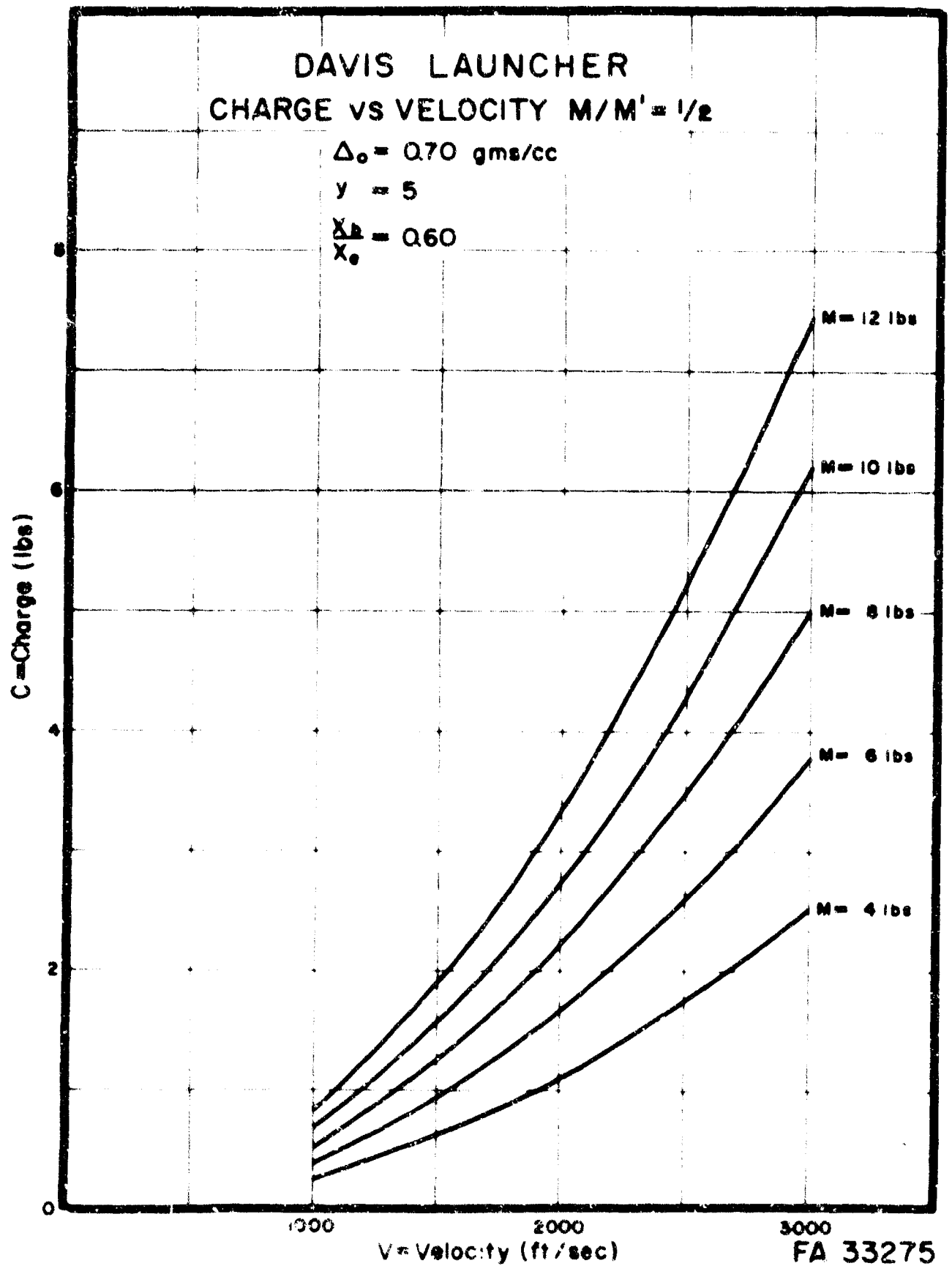
Figure 3. Charge vs Velocity M/M' = 1/2
