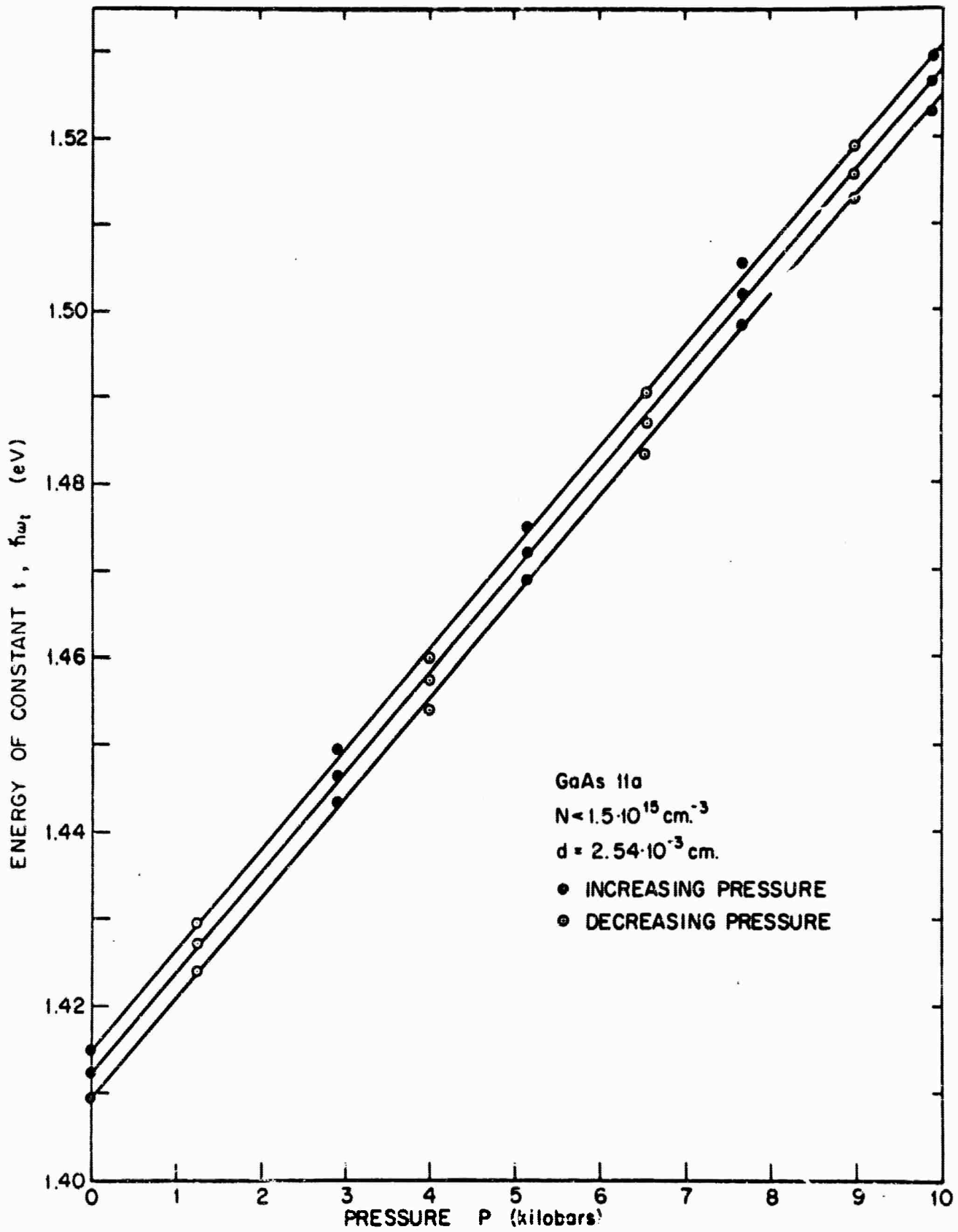
FIG. 3-4 ENERGY OF CONSTANT TRANSMISSION VERSUS PRESSURE FOR GaAs IIa
