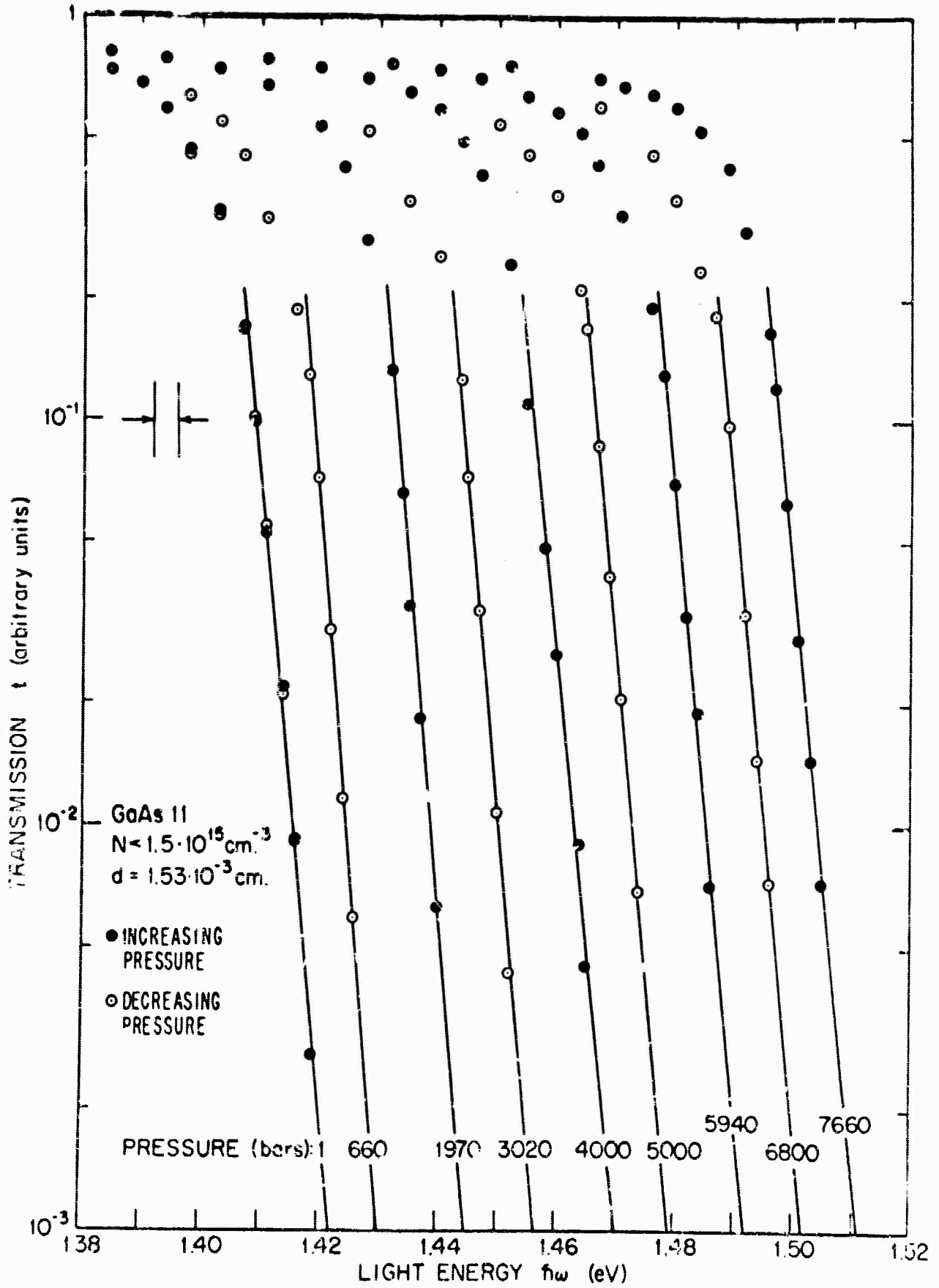
FIG. 3-1 EFFECT OF PRESSURE ON THE OPTICAL TRANSMISSION OF GaAs II
