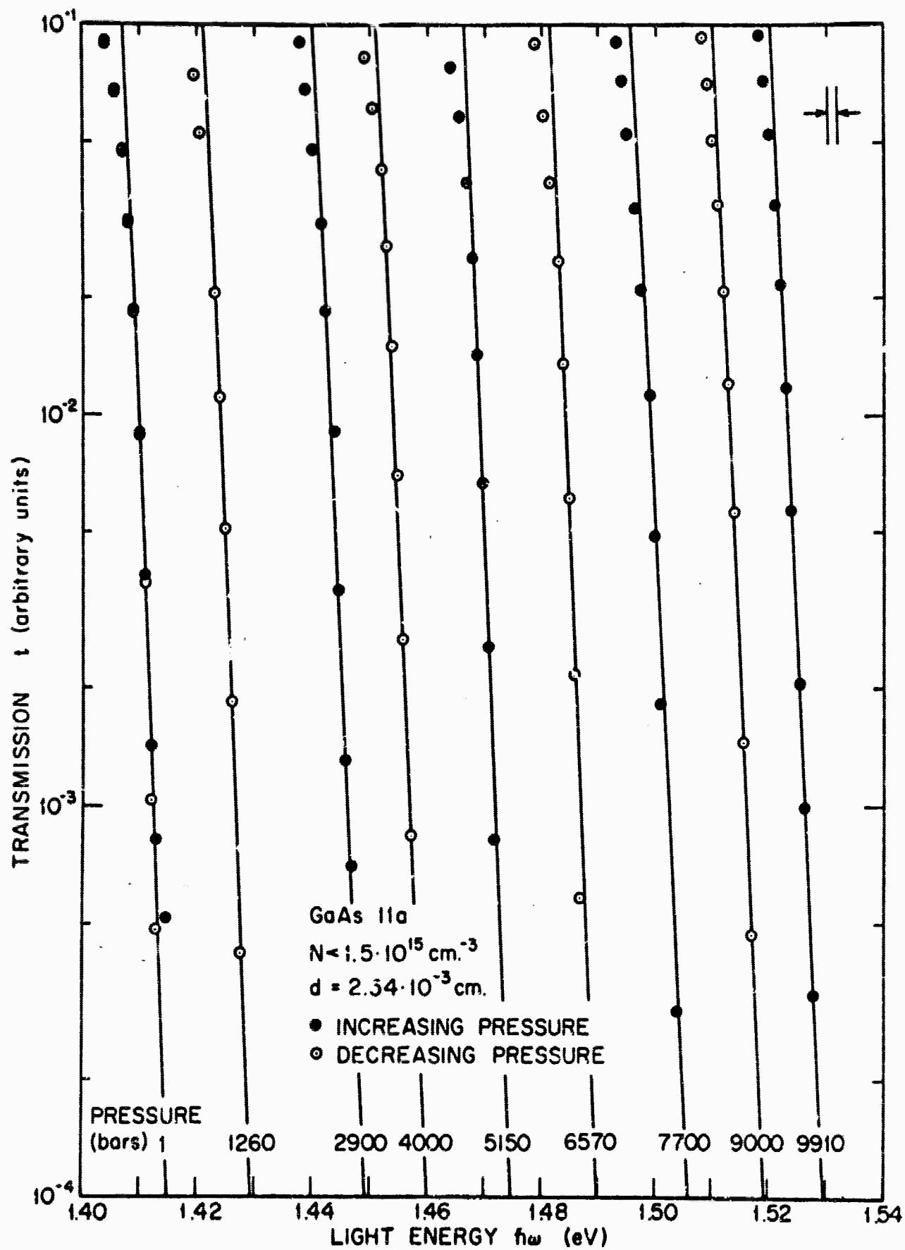
FIG. 3-3 EFFECT OF PRESSURE ON THE OPTICAL TRANSMISSION OF GaAs 11a.
