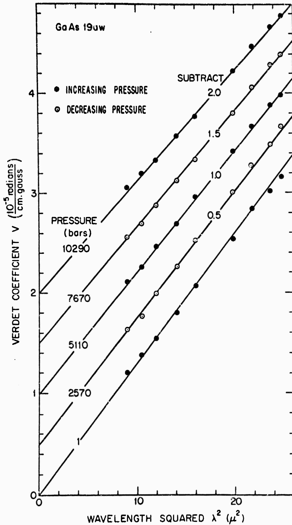
FIG. 3-21 PRESSURE DEPENDENCE OF V FOR GaAs 19 \mu w
