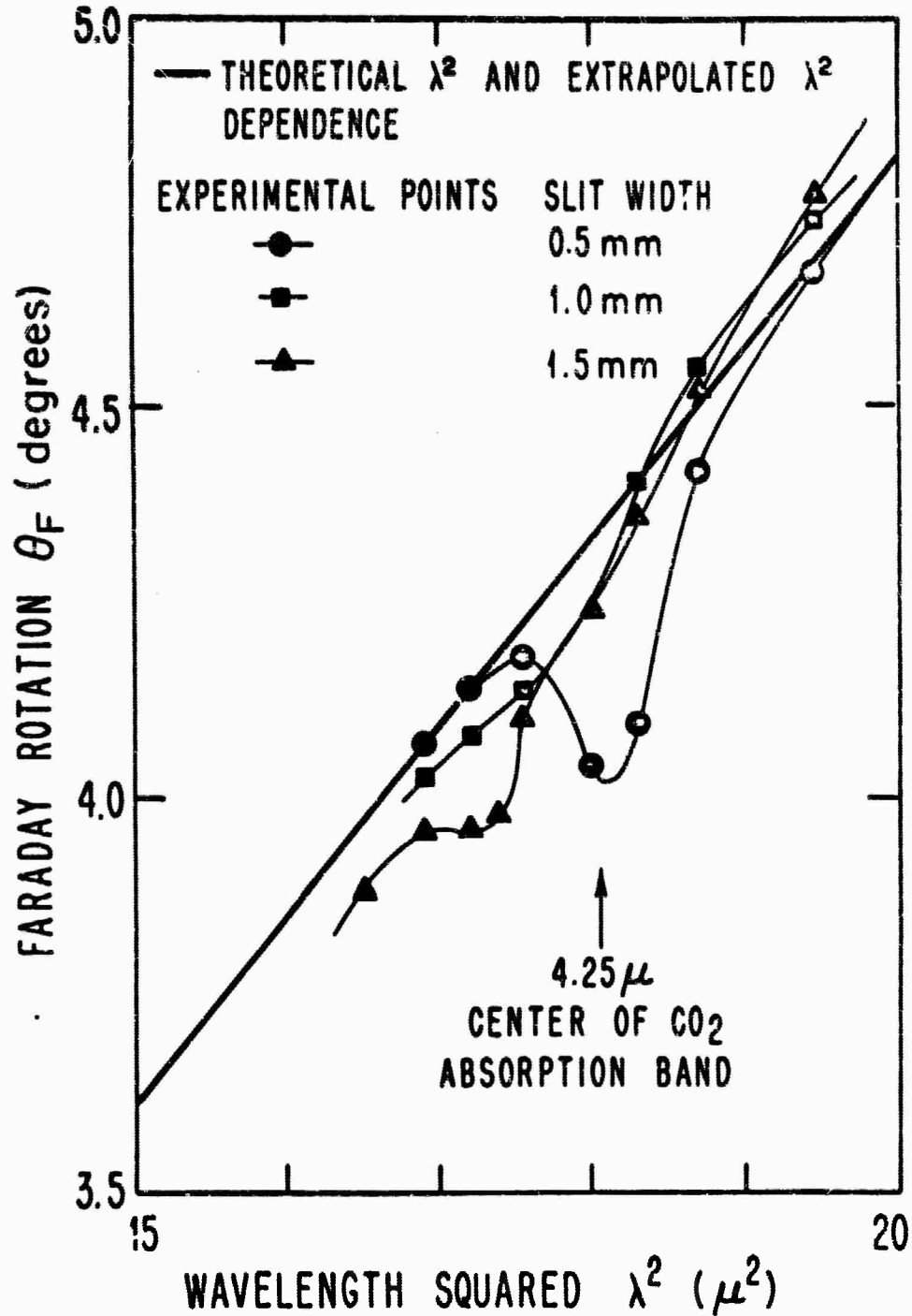
FIG. 3-11 ANOMALOUS ROTATION IN GaAs NEAR THE 4.25 \mu CO 2 ABSORPTION BAND.
