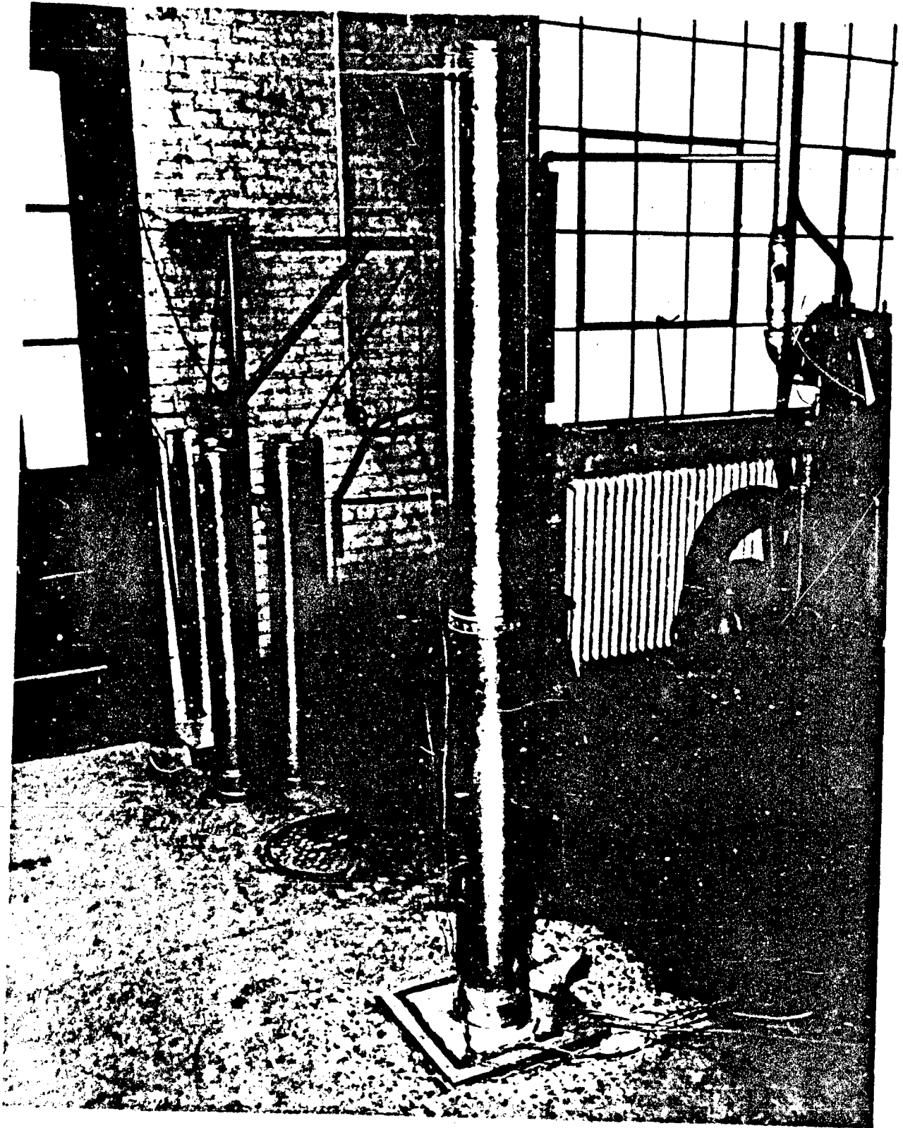
Figure 4. Stack Extending from Shelter
