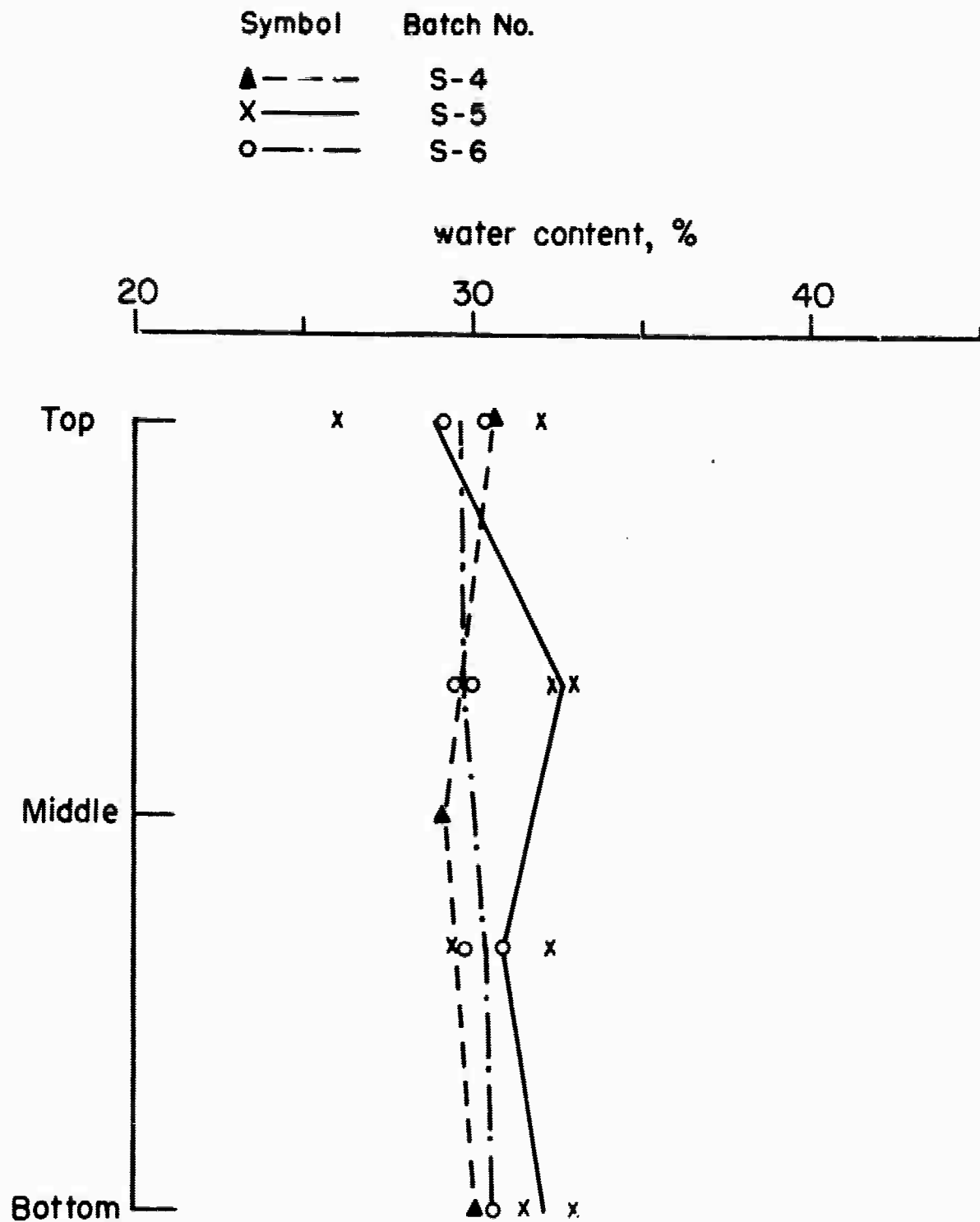
Fig. 3.1 Variation in Water Content of Batches of Boston Blue Clay
