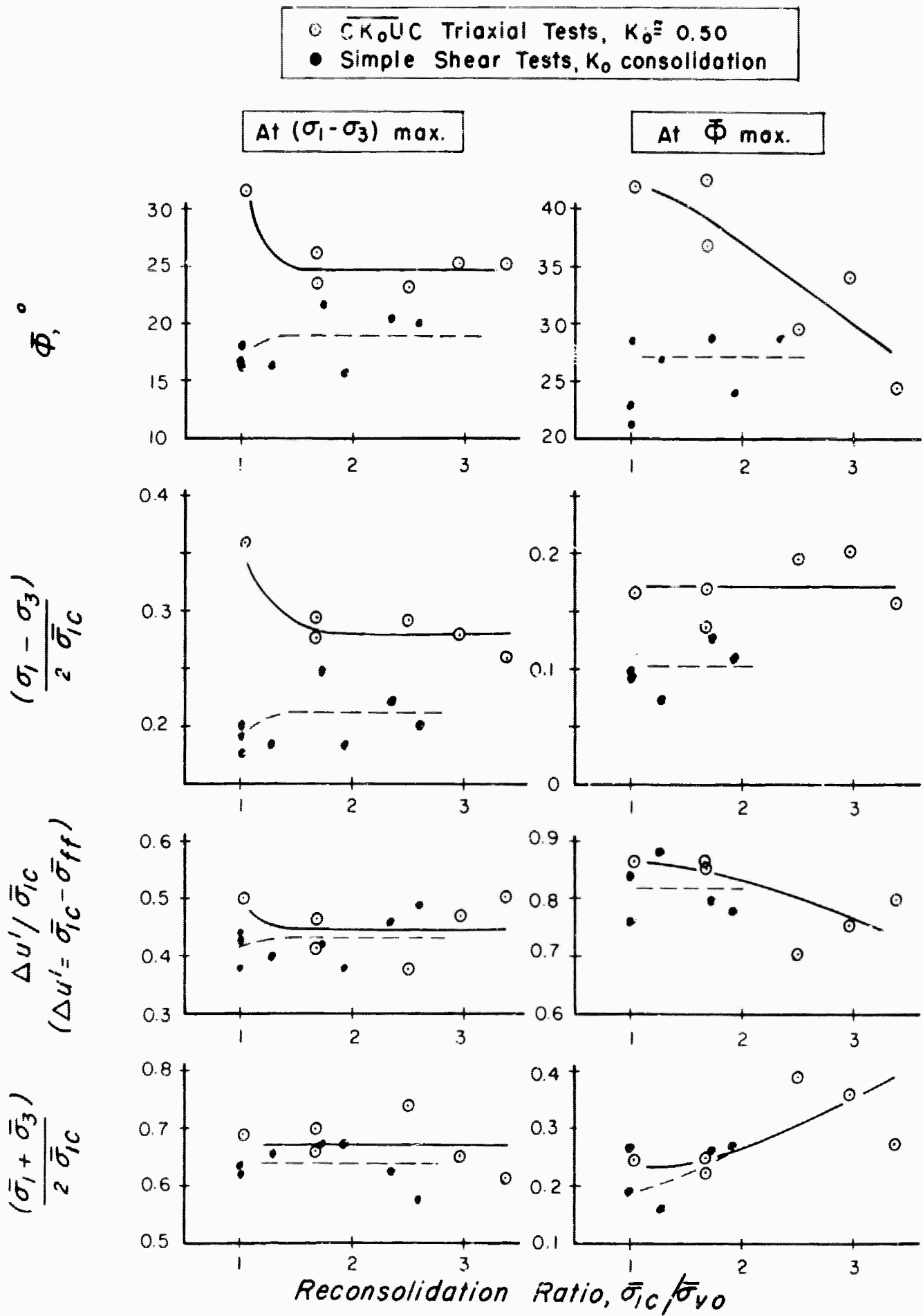
Fig. 2.29 Strength Parameters from \overline{C\bar{U}} Triaxial and Simple Shear Tests on N.C. Undisturbed Manglerud Clay (Landva, 1962)
