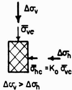
Fig.1.4 Typical Stress Systems in the Field for a Normally Consolidated Clay (footings and walls are assumed to have frictionless surfaces)
