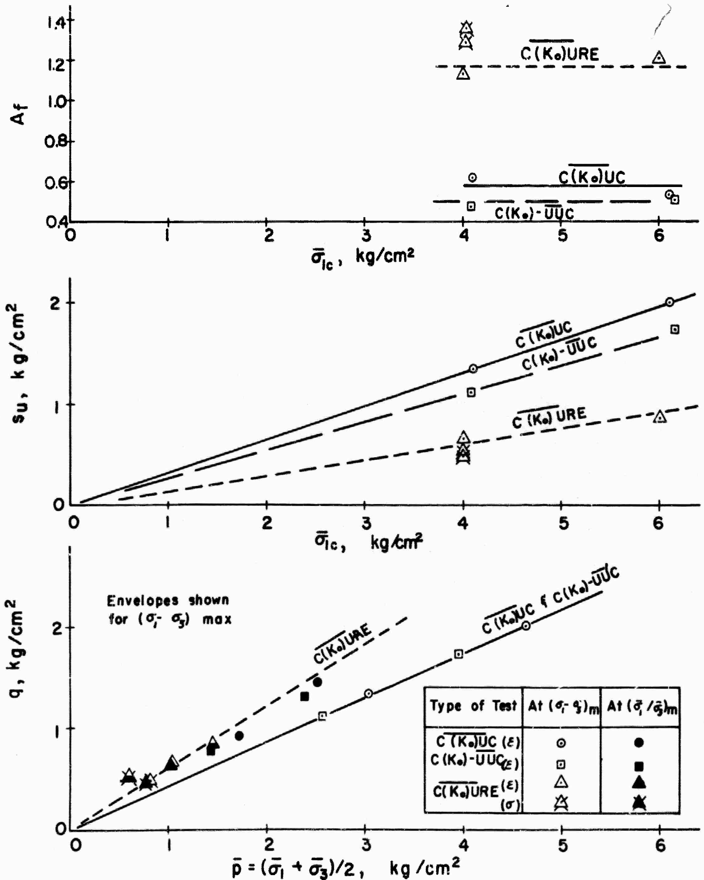
Fig.4.6 Summary of Strength Data from \overline{C}U Tests on N.C. BBC with K_0 Consolidation
