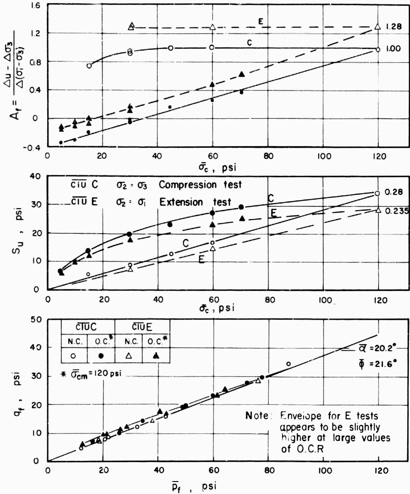
Fig. 2.16 Undrained Strength Parameters for \overline{CIU} C and \overline{CIU} E Tests on Remolded Weald Clay (Parry, 1960)
