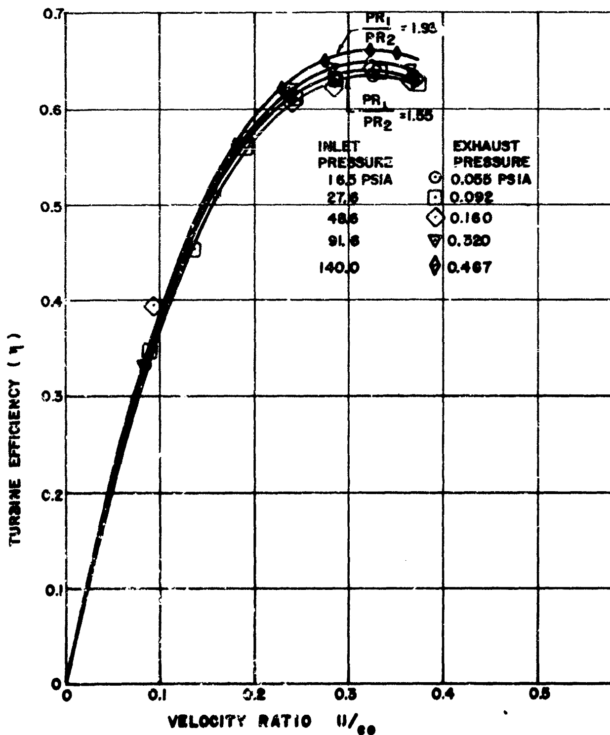
FIGURE 28. TEST DATA OF RE-ENTRY TURBINE (EFFICIENCY)
