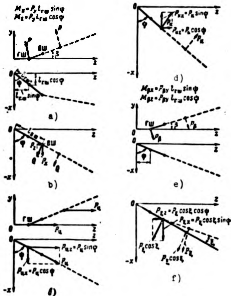
Fig. 9.8. The determination of forces and moments on a rotor hub.
