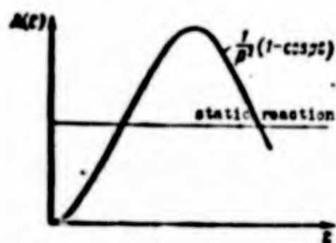
Fig. 4.15. Transition conductivity curve of a linear system with one degree of freedom.
