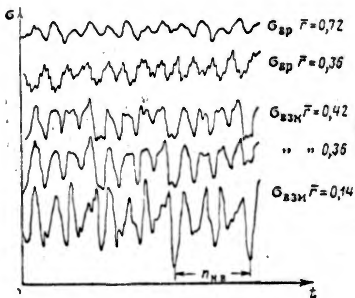
Fig. 9.7. Recording of variable stresses in a rotor blade spar in conditions of deceleration before landing.
