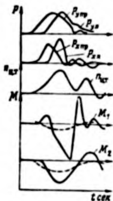
Fig. 4.27. Character of change of forces in a fuselage during landing. --- rigid aircraft, — elastic aircraft.
