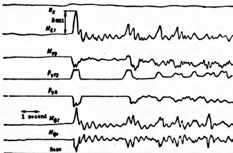
Fig. 10.44. Example of deciphering recorded parameters: n_x - overload, M_w - bending moment of wing, M_{f1} , M_{f2} , and M_{f3} - bending moments of fuselage in 1, 2, and 3 sections, P_{y \text{ left}} and P_{y \text{ right}} - vertical components of forces on left and right landing gear strut, h_{\text{max}} - magnitude of ordinate in mm, corresponding to maximum deviation of measured magnitude from reading level.
