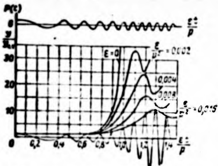
Fig. 3.7. Oscillations during passage through resonance.
