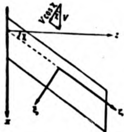
Fig. 2.15. Diagram of a sweptback wing.
