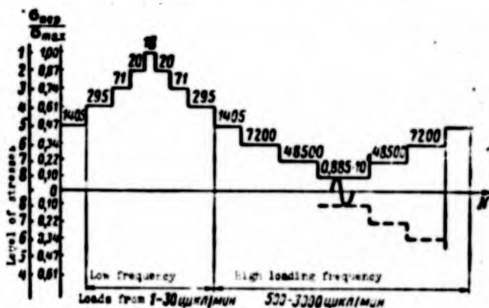
Fig. 7.40. Diagram of one loading cycle (1 cycle of the program contains 10^6 loads).
