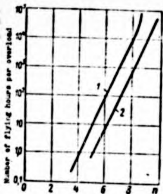
Fig. 7.27. Recurrence of maneuvering overloads.
