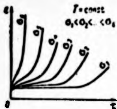
Fig. 8.19. Approximate change of the characteristics of creep with the increase of stresses.
