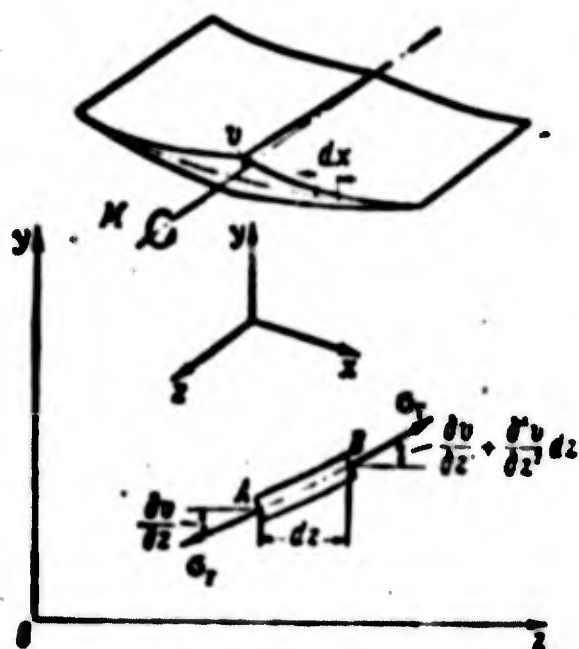
Fig. 8.27. Diagram of the action of stresses in a double-wedge wing during bending.
