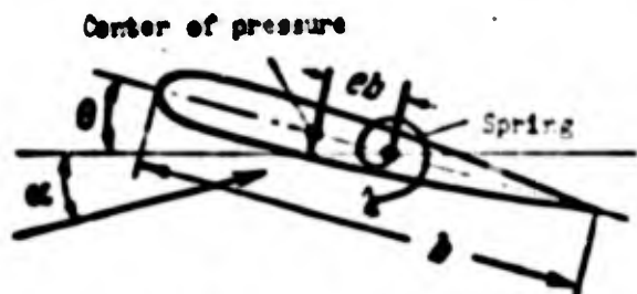
Fig. 2.14. Diagram of section of elastic wing.
