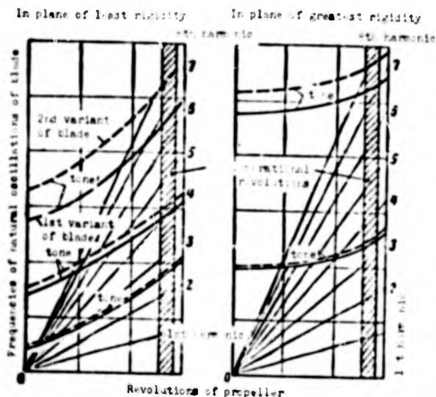
Fig. 3.24. Typical graph of change in natural frequencies of flexural oscillations of blade of helicopter rotor. 1st variant — blade with bad frequency responses, 2nd variant — blade with improved frequency responses.
