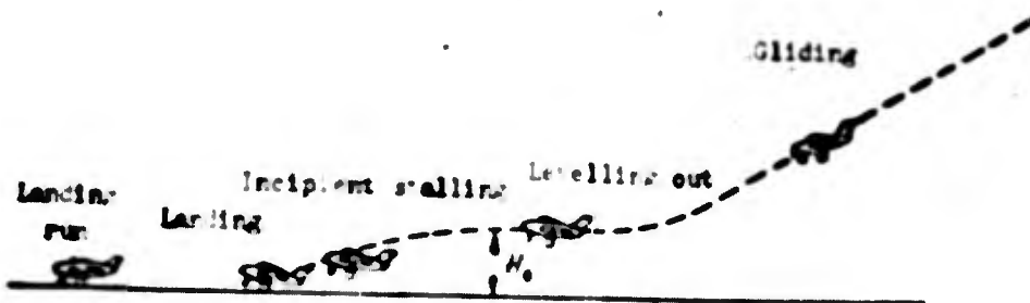
Fig. 2.30. Trajectory of landing.
