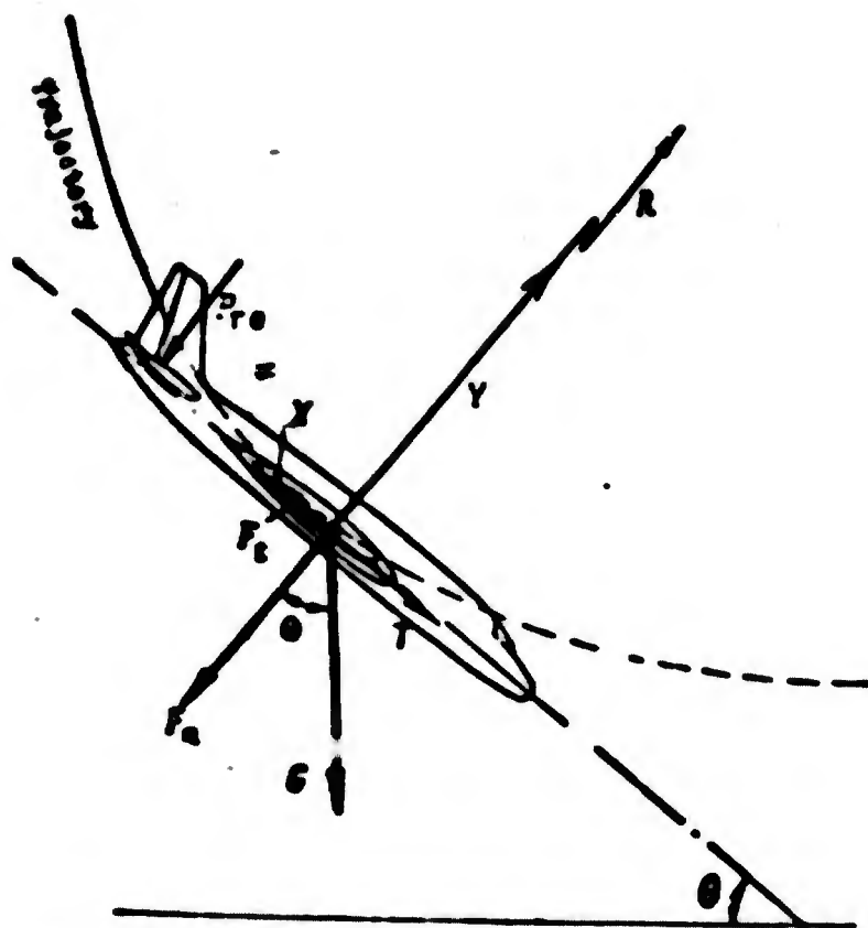
Fig. 1.7. Forces acting on an aircraft in curvilinear flight.
