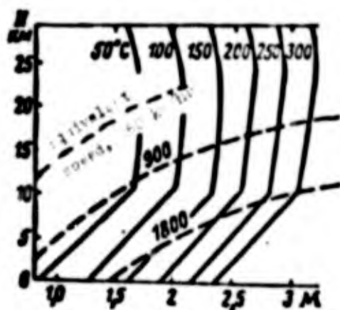
Fig. 8.8. Curves of equal steady-state skin temperatures as functions of Mach number and altitude of flight H .
