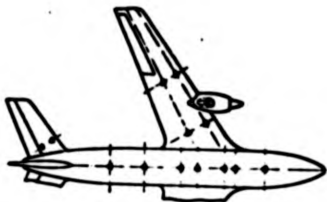
Fig. 10.36. Diagram of installation of strain gauges for the investigation of loads. \Delta - place of installation of strain gauges.
