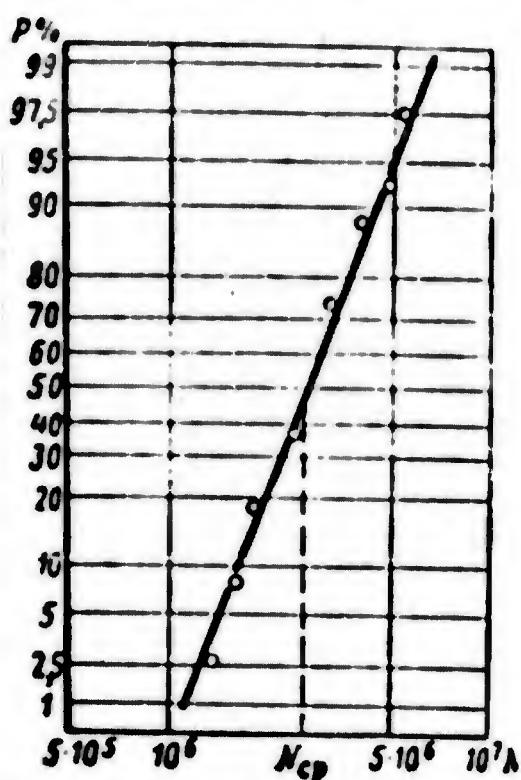
Fig. 7.6. Results of endurance tests of a group of samples.
