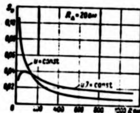
Fig. 10.29. Change of sensitivity of equipment according to diagram II, depending upon resistance of strain gauge.
