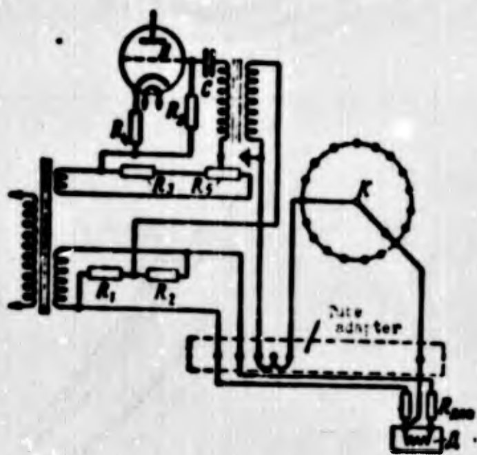
Fig. 10.14. Schematic diagram of equipment for measurement of temperatures. \Delta - transducer, R_{\text{доп}} - additional resistance, R_1, \dots, R_c - resistance, I - tube, K - commutator.
