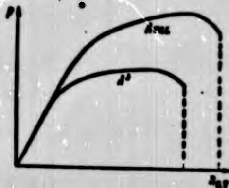
Fig. 10.20. Diagram of work of landing gear. A_{\max} - maximum work, A^{op} - operational work.
