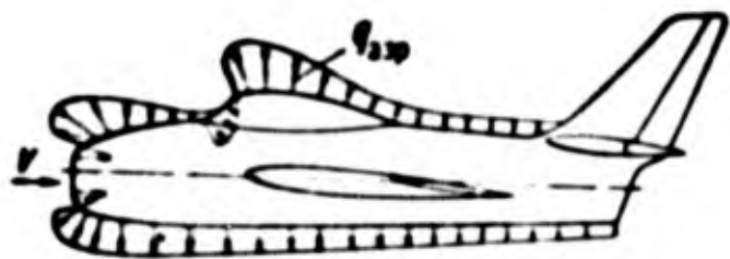
Fig. 2.44. Distribution of aerodynamic loads on surface of fuselage.
