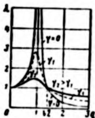
Fig. 3.13. Resonance characteristics of a damped object with different damping.
