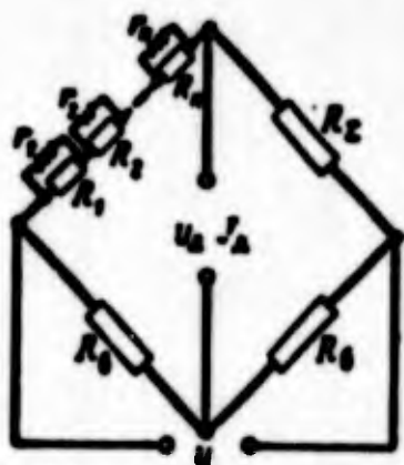
Fig. 10.32. Series connection of strain gauges with shunting resistors r_1 .
