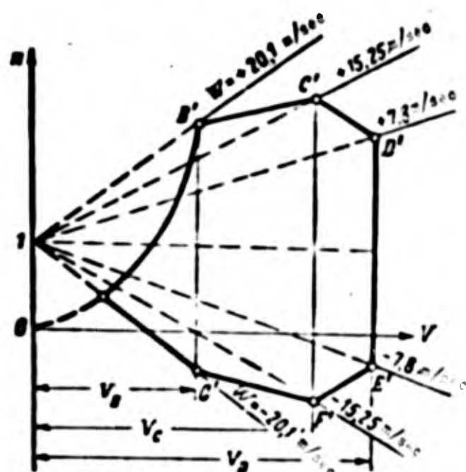
Fig. 1.28. Diagram V-n for overloads during flight in bumpy air.
