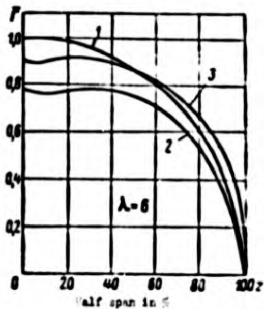
Fig. 2.12. Influence of sweepback on distribution of circulation along span. 1) for straight wing; 2) for sweptback wing during an angle of attack equal to angle of attack of straight wing; 3) for sweptback wing during lift equal to lift of a straight wing.
