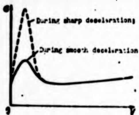
Fig. 9.21. Dependence of variable normal stresses in the reductor frame of a helicopter on the speed of flight.
