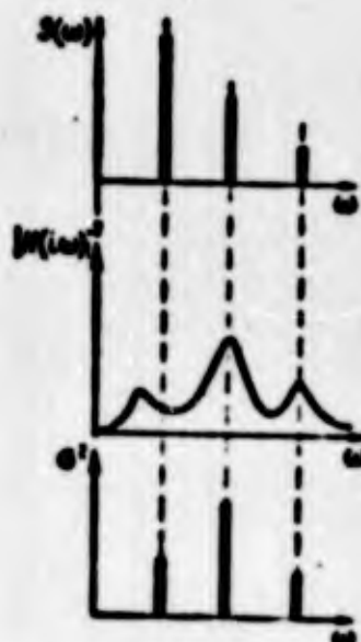
Fig. 5.21. Graphs of functions of mechanical conductivity and stresses with discrete noise spectrum.
