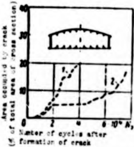
Fig. 7.41. Character of crack development in a wing structure. 1) aluminum alloy of type V95; 2) aluminum alloy of type D16.
