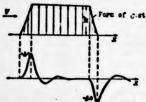
Fig. 7.24. Character of change of G-force during passage of an aircraft through a gust.
