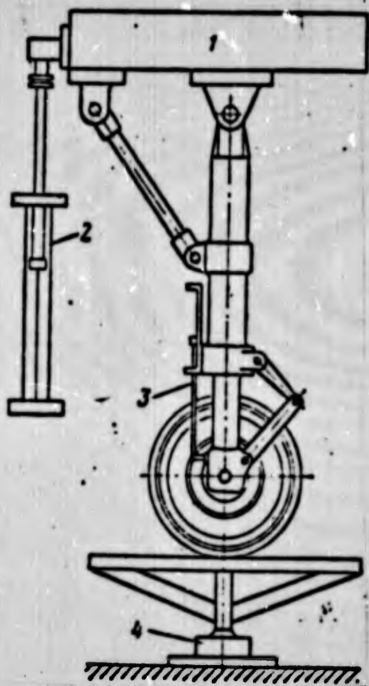
Fig. 10.18. Diagram of pile-driver installation. 1) load; 2) slide wire for recording the movements of the center of gravity of dropped load; 3) slide wire for recording the process of shock-absorption. 4) hydraulic dynamometer.
