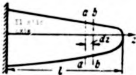
Fig. 3.19. Console diagram of a wing.
