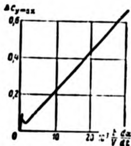
Fig. 1.23. Dependence of \Delta c_{y \max} on speed of change of angle of attack.
