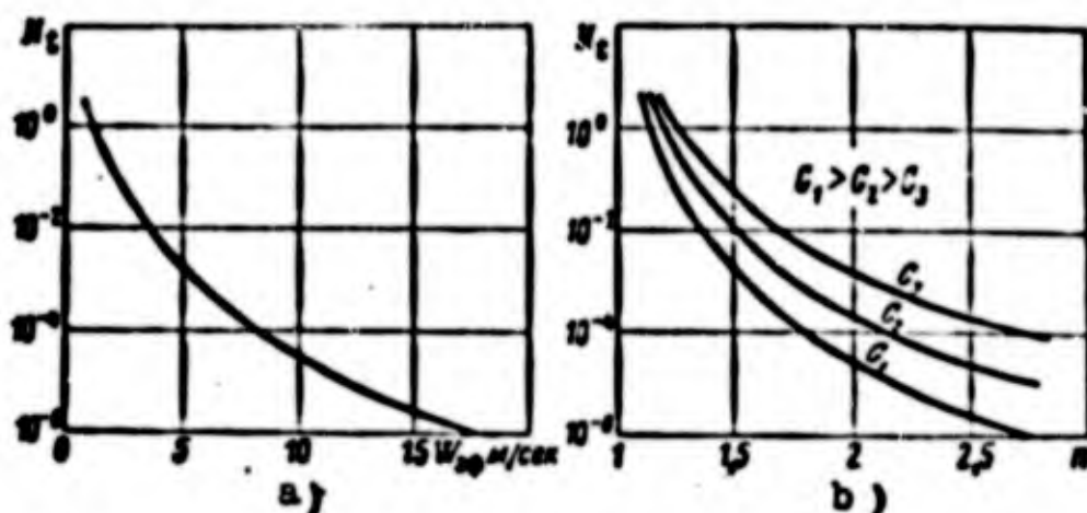
Fig. 7.34. Graphs of integral recurrence of gusts of wind (a) and overloads of an aircraft (b).
