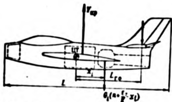
Fig. 2.45. Forces acting on fuselage in flight.
