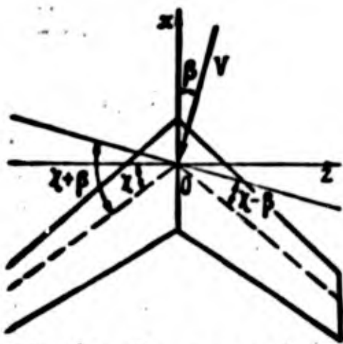
Fig. 2.28. Diagram of swept-back empennage during sideslip.
