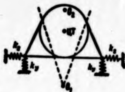
Fig. 9.15. Diagram of a helicopter for the calculation of ground resonance.
