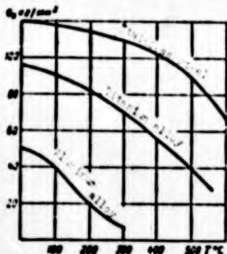
Fig. 8.16. Change of ultimate strength \sigma_b of certain alloys, depending upon temperature.
