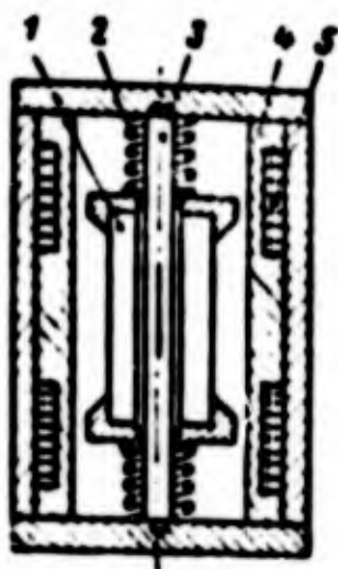
Fig. 10.9. Diagram of a magnetoelectric (inductive) vibrometric transducer.
