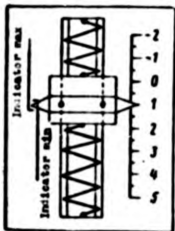
Fig. 1.1. Recorder of overloads of V. P. Vetchinkin.
