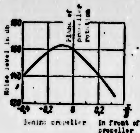
Fig. 5.18. Curve of noise level in the plane of propeller rotation. x/D - distance (along length of fuselage) in fractions of propeller diameter D .
