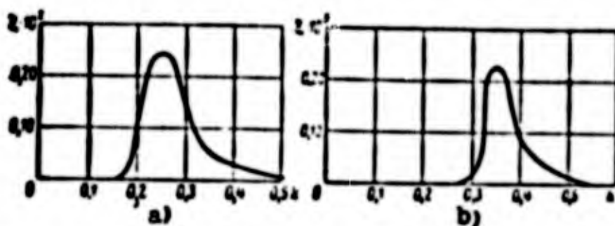
Fig. 7.32. Change of the function of damage intensity. a) maneuvering aircraft; b) non-maneuvering aircraft.
