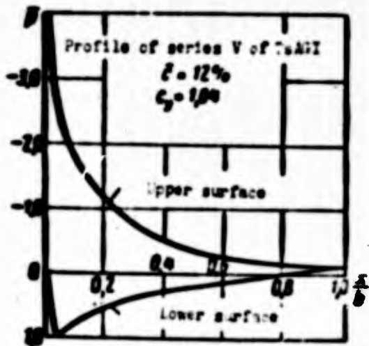
Fig. 2.3. Distribution of pressure along chord of wing at large angle of attack. \bar{p} = \frac{p_{exc}}{q} — pressure coefficient, b_{exc} — excess pressure at point, x/b — distance from nose of profile in fraction of chord b .
