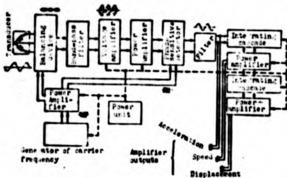
Fig. 10.11. Block diagram of vibration-measuring equipment with electromagnetic transducers.
