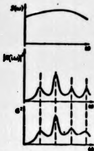
Fig. 5.20. Graphs of the function of mechanical conductivity and stresses for a panel with continuous noise spectrum.
