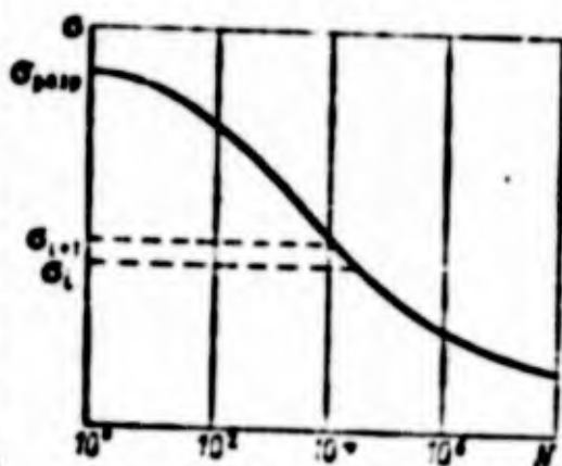
Fig. 7.31. Strength characteristics of a structural element.
