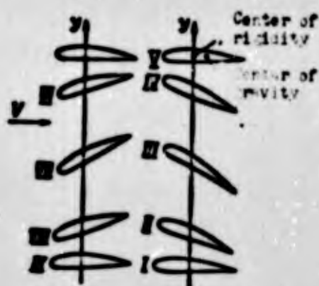
Fig. 6.3. Diagram of the appearance of flexure-torsion wing flutter. I-IX) consecutive positions of wing section during oscillations.
