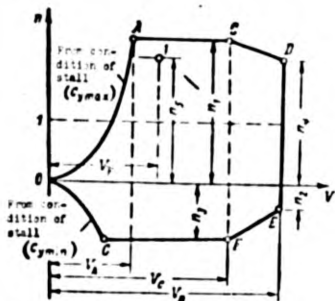
Fig. 1.27. Diagram V-n for maneuvering cases of flight.
