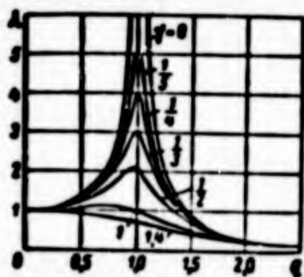
Fig. 3.5. Resonance curves.
