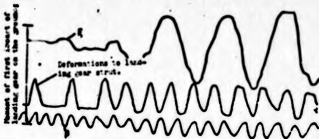
Fig. 9.16. Recording of the beginning of ground resonance on a helicopter. \xi - lag angle of blade (with respect to DH); \beta - blade-flapping angle (with respect to FH).
