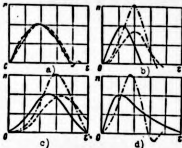
Fig. 3.10. Indications of instrument during action of overloads, determined by: a) formula (3.45) at q = 0.1 ; b) formula (3.45) at q = 0.7 ; c) formula (3.46) at q = 0.7 ; d) formula (3.47) at q = 0.7 — actual overload, — — — indications of instrument at h = 0.1 p , — — — — — indications of instrument at h = 0.7 p .
