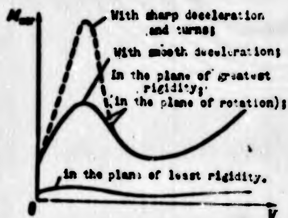
Fig. 9.18. Dependence of variable bending moments in a tail rotor blade on the speed of flight.
