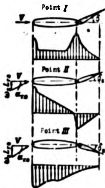
Fig. 2.23. Distribution of loads on horizontal empennage during different phases of elevator deflection (points I, II, III, correspond to Fig. 2.22).
