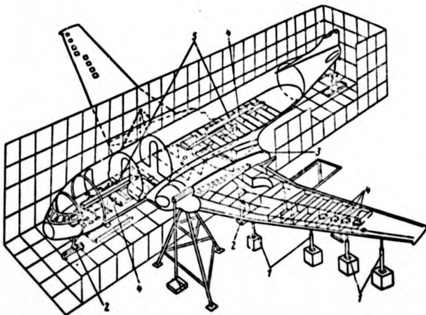
Fig. 7.38. Overall view of tests in a hydrobasin. 1) loading system of wing; 2) attachment of landing gear; 3) packing; 4) ballast; 5) lever system of fuselage loading.
