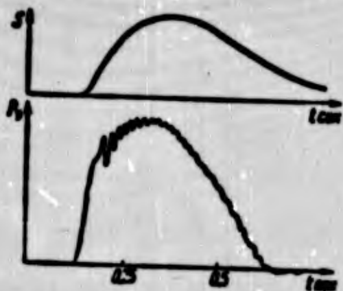
Fig. 10.19. Diagram of the change of the support reaction P_y and the movement of shock-absorption S during the drop of landing gear on a pile-driver.
