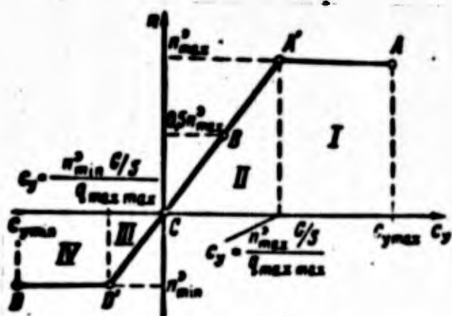
Fig. 2.1. Basic calculation cases of a wing.
