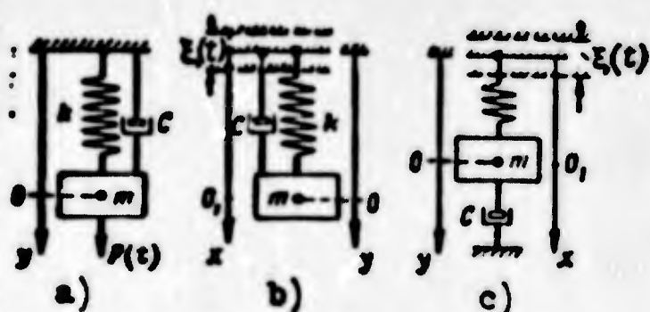
Fig. 3.3. Excitation of oscillation in linear systems with one degree of freedom. a) force is applied to mass; b and c) assigned motion of point of bracing (b-damping is proportional to relative velocity of mass; c-damping is proportional to absolute velocity of mass).
