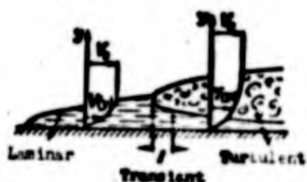
Fig. 8.4. Approximate structure of boundary layer.
