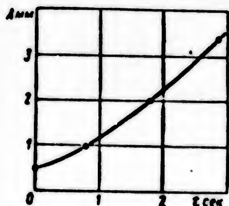
Fig. 6.8. Change of amplitudes of oscillations during antisymmetric flexure-aileron flutter of a glider.
