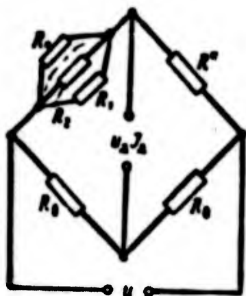
Fig. 10.30. Parallel connection of strain gauges.
