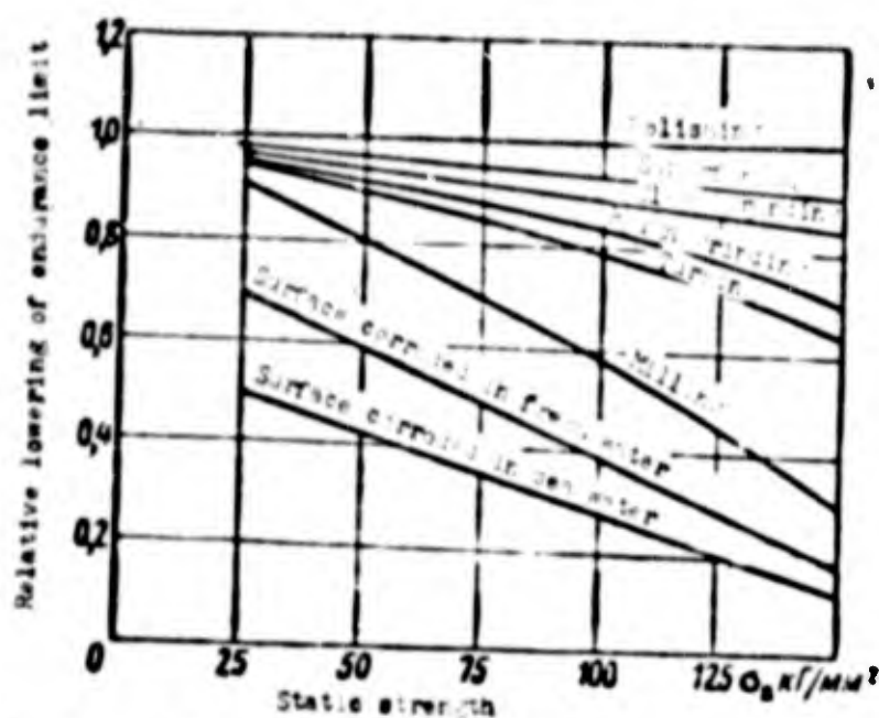
Fig. 7.8. Influence of quality of treatment on endurance limit of steel depending upon its static strength.
