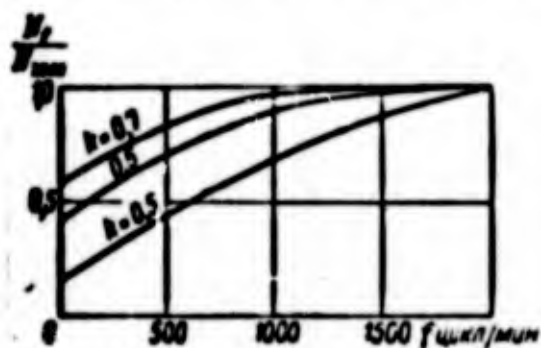
Fig. 7.13. Influence of loading frequency on fatigue strength of an aluminum alloy when k = 0.5 to 0.7 .
