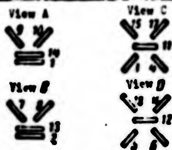
Fig. 10.26. Distribution of strain gauges on a thin-walled shell for measuring the main load components.
