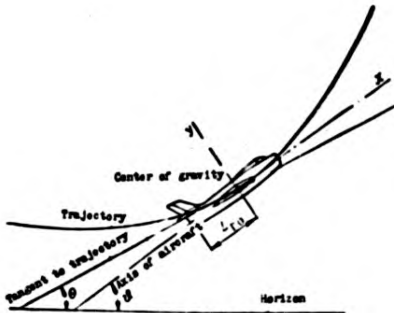
Fig. 1.11. Geometric parameters of trajectory of aircraft during maneuver.
