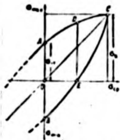
Fig. 7.5. Complete strength diagram.
