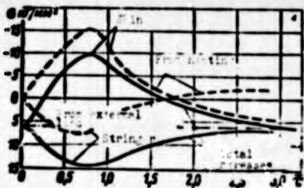
Fig. 8.15. Total stresses from an external load and temperature.
