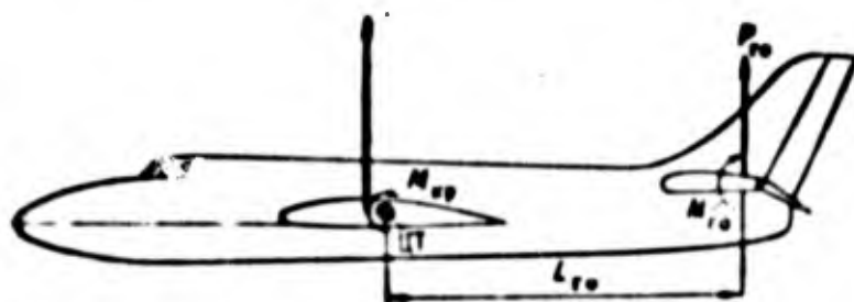
Fig.2.29. Diagram of aerodynamic forces acting on aircraft.
