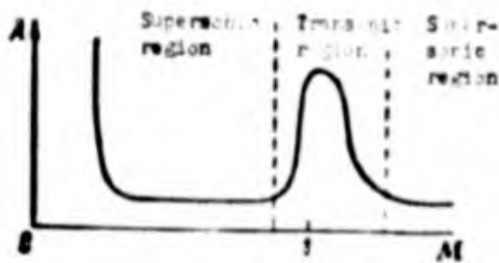
Fig. 5.4. Graph of the change of amplitudes of aerodynamic oscillations of aircraft according to flight Mach number.
