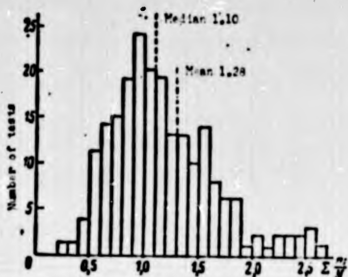
Fig. 7.15. Diagram of the results of fatigue tests with several loading stages (according to foreign data).
