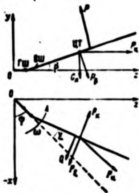
Fig. 9.4. Forces acting upon a rotor blade.
