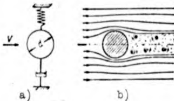
Fig. 5.6. Diagram of the appearance of oscillations of a cylinder in a flow of air. a) diagram of cylinder oscillations; b) diagram of vortices in the wake of a circular cylinder.
