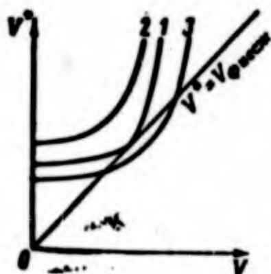
Fig. 6.14. An analysis of the roots of the flutter equation (6.17).
