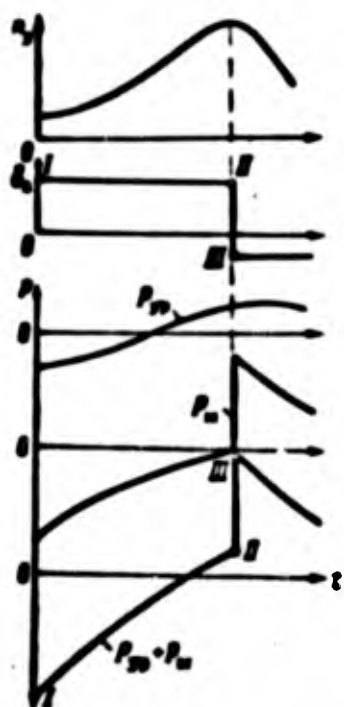
Fig. 2.22. Phases of elevator deflection.
