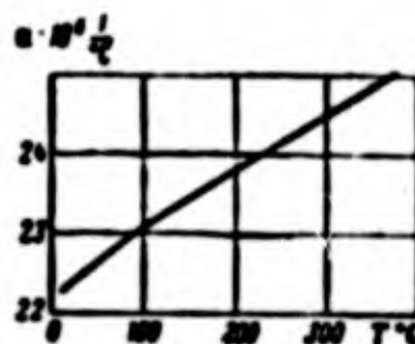
Fig. 8.22. Change of the coefficient of linear expansion of an aluminum alloy with respect to temperature.
