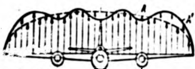
Fig. 2.10. Relative circulation of aerodynamic load during small and large angles of attack of wing.
