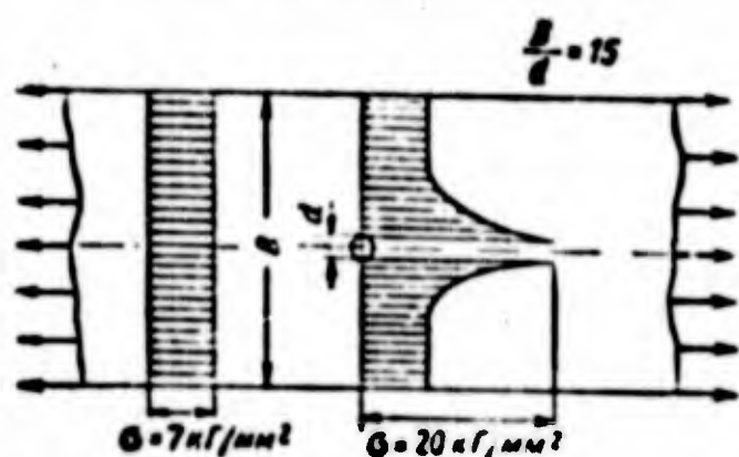
Fig. 7.7. Distribution of stresses in a plate which has a hole in it.
