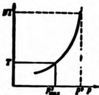
Fig. 1.29. Approximate dependence of probable maximum load on duration of flight.
