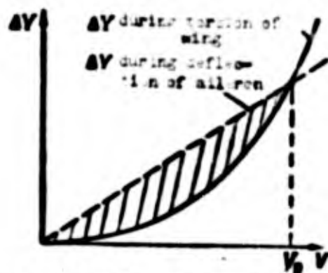
Fig. 2.18. Change in increase of lift during deflection of aileron with respect to speed of flight.
