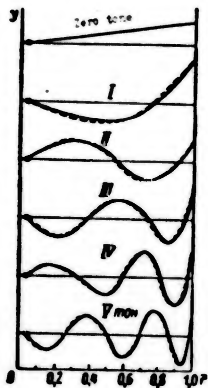
Fig. 3.25. Forms of oscillations (in plane of least rigidity) of blade of rotor of helicopter without rotation and in field of centrifugal forces. — revolutions are equal to zero, ---- operational revolutions \bar{r} = \frac{r}{R} relative radius of section of blade.
