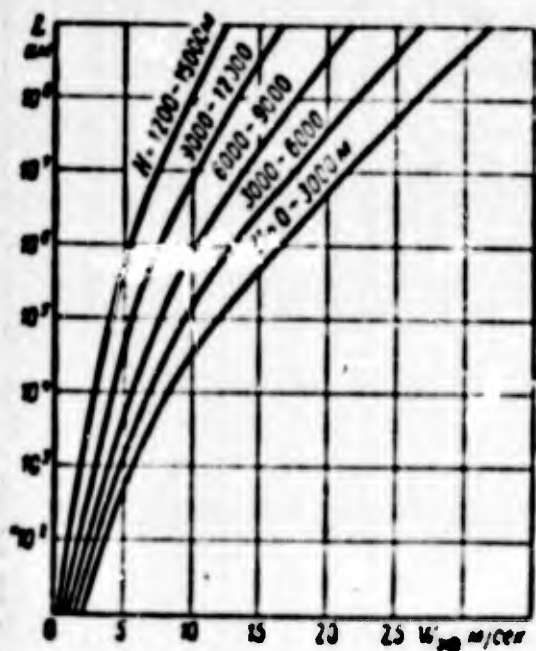
Fig. 7.26. Recurrence of gusts at different altitudes.
