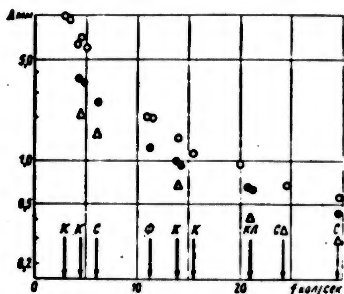
Fig. 5.9. Combined graph of aerodynamic oscillations of an aircraft. ○ — wing, ● — stabilizer, Δ — fin. ↓ — frequencies of natural oscillations: K — wing, Φ — fuselage, C — stabilizer, KΠ — fin.
