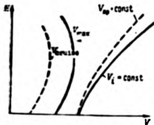
Fig. 1.3. Approximate character of limitation of flight speed of a piston-engined aircraft.
