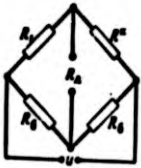
Fig. 10.3. Diagram of a measuring bridge.
