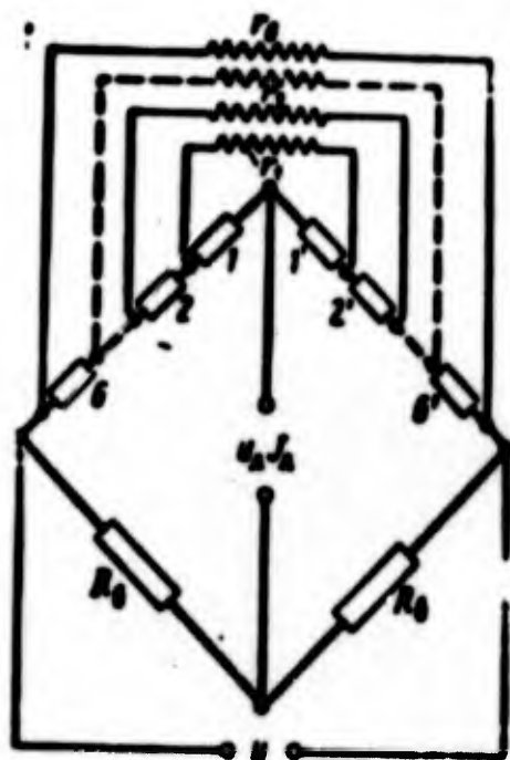
Fig. 10.34. Simplified diagram of series connection of strain gauges.
