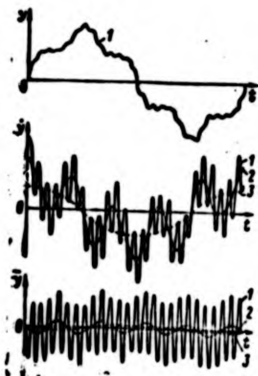
Fig. 10.8. Graphs of displacements y , speeds \dot{y} , and accelerations \ddot{y} of the same oscillatory motion (illustration to Table 10.1). 1) composite graph of oscillations with frequencies of 2, 10, and 50 oscillations per second; 2) composite graph of oscillations with frequencies of 2 and 10 oscillations per second; 3) graph of oscillations with frequency of 2 oscillations per second.
