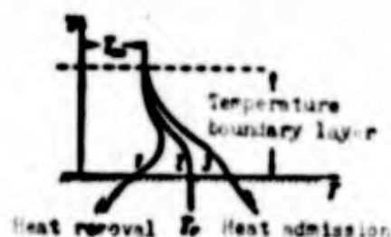
Fig. 8.5. Profile of air temperatures on the boundary layer. 1) wall temperature less than T_r ("cold" wall); 2) wall temperature equal to T_r (heat-insulated wall); 3) wall temperature greater than T_r (hot wall). T_\infty — temperature of undisturbed flow.
