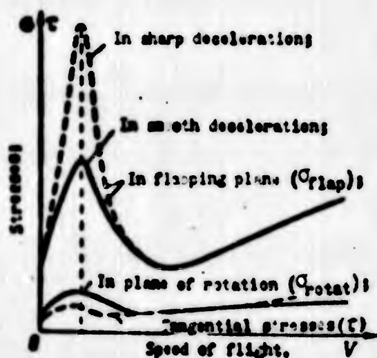
Fig. 9.17. Dependence of variable stresses in the spar of a rotor blade on the speed of flight.
