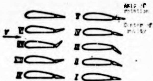
Fig. 6.6. Diagram of the appearance of flexure-aileron wing flutter. I-IX) consecutive positions of aileron during oscillations.
