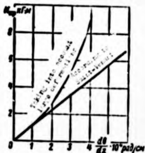
Fig. 8.26. Change of \frac{d\theta}{dz} during torsion of a double-wedge wing.
