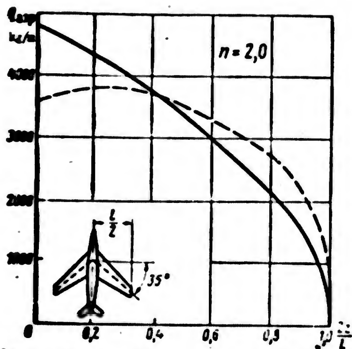
Fig. 2.16. Influence of deformations of sweptback wing on distribution of linear load along wing. — elastic wing, - - - rigid wing.
