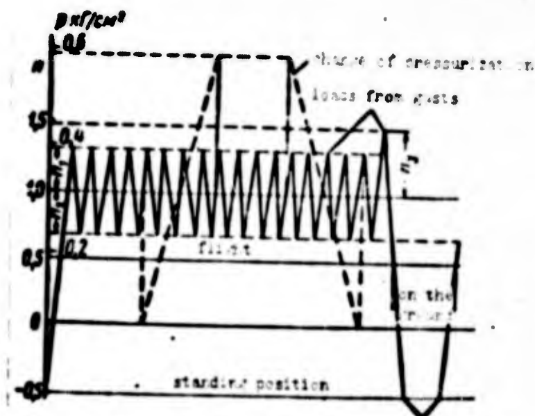
Fig. 7.37. Diagram of the loading program of the aircraft "Caravel" in one cycle, corresponding to a typical flight. n_1 - overload corresponding to an ascending gust of w_{ef} = 3 m/sec, n_2 - overload, corresponding to a descending gust of w_{ef} = 3 m/sec, n_3 - overload corresponding to an ascending gust of w_{ef} = 5 m/sec.
