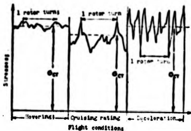
Fig. 9.22. Stresses appearing in the main rotor blade of a helicopter in different flight conditions ( \sigma_{st} - stresses from static load).
