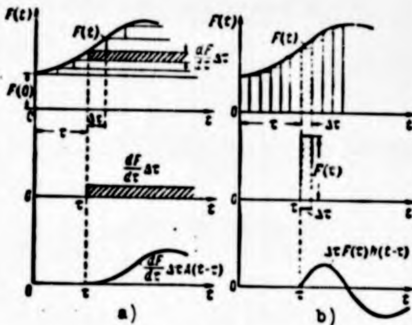
Fig. 4.17. Geometric representation of the Duhamel integral by the step function a) and \delta -function b).
