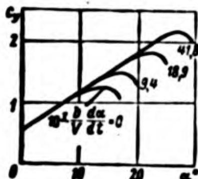
Fig. 1.21. Influence of speed of change of angle of attack on c_{y \max} ( \lambda = 5 , Re = 3.6 \cdot 10^5 , profile GÖ 398, wing is motionless, direction of flow changes).
