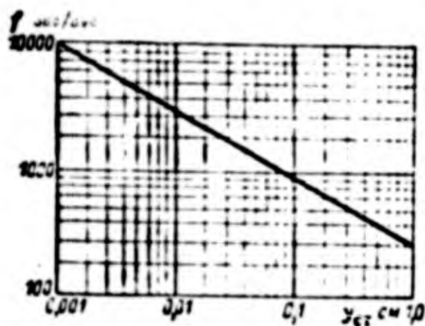
Fig. 3.14. Dependence of natural frequency of a damped object on static sag of shock absorber.
