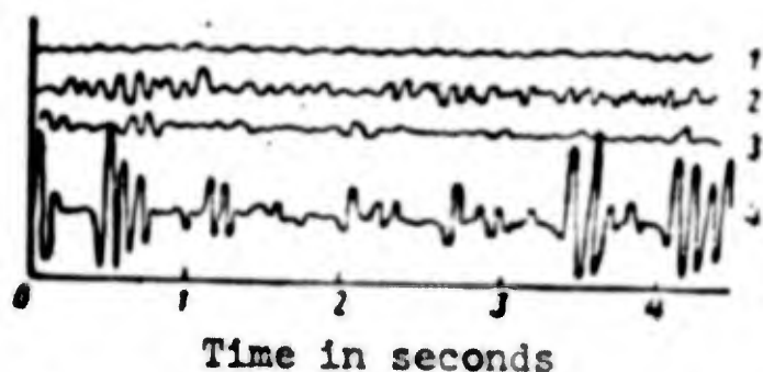
Fig. 5.11. Recording of oscillations during buffeting of the empennage on a glider. 1 and 2) fuselage correspondingly on axes z and y , 3) wing; 4) elevator.
