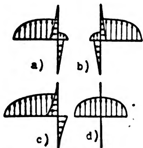
Fig. 2.26. Influence, on asymmetric loads, of the location of the horizontal empennage on the fin. a and b) low location of stabilizer; c) middle location of stabilizer; d) stabilizer is located in upper part of fin.
