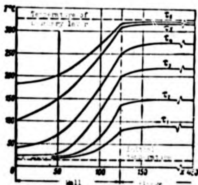
Fig. 8.10. Temperature field of the wall of a spar and skin for different durations of heating. x — distance from center of wall
