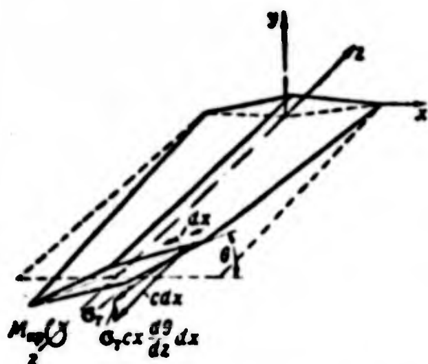
Fig. 8.24. Diagram of the action of torque and stresses in a double-wedge wing.
