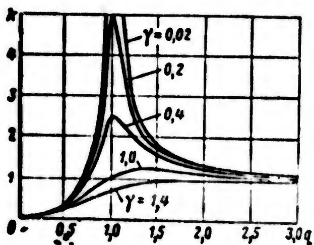
Fig. 10.6. Frequency-response curves of a vibrometric transducer.
