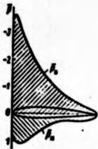
Fig. 10.25. Diagram of pressure distribution along a wing profile. \bar{p} is the pressure coefficient, \bar{p}_{up} and \bar{p}_{low} correspondingly are the pressure coefficients on the upper and lower surfaces of the wing.
