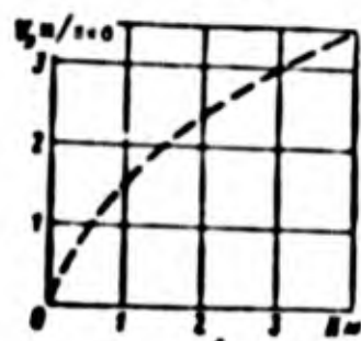
Fig. 2.31. Dependence of V_y on altitude of holding.
