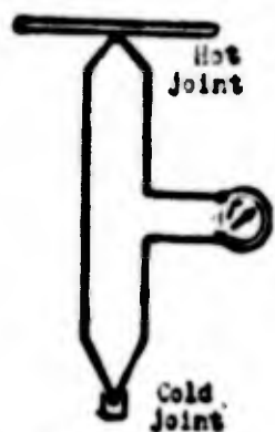
Fig. 10.12. Measuring circuit of temperatures with the help of a thermocouple and galvanometer.
