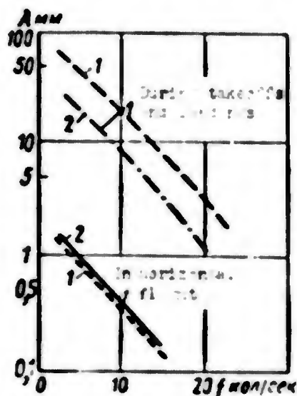
Fig. 5.16. Comparison of aerodynamic oscillations and oscillations appearing during takeoffs and landings. 1) stabilizer; 2) wing.
