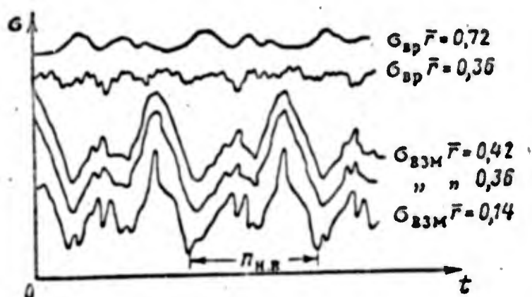
Fig. 9.6. Recording (oscillogram) variable stresses in a rotor blade spar in horizontal flight. \sigma_{\text{flap}} — in flapping plane, \sigma_{\text{rotat}} — in plane of rotation of blade, \bar{r} — relative radius of blade section, n_{\text{m.r.}} — period of oscillation, corresponding to one turn of main rotor.
