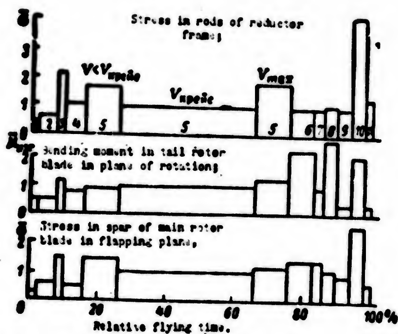
Fig. 9.23. Relative load capacity of assemblies of a single-rotor helicopter in different flight conditions (variable bending moment M_{bend} and stresses \bar{\sigma} in every structural assembly refer to the moment and stress which appear in horizontal flight at cruising speed).
