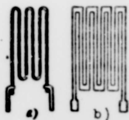
Fig. 10.1. Diagrams of strain gauges. a) wire strain gauge; b) strain gauge made from foil.
