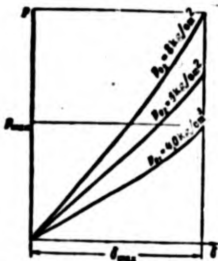
Fig. 2.35. Diagram of work of a pneumatic tire.
