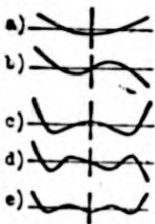
Fig. 320. Forms of natural flexural oscillations of a straight wing of a transport aircraft. a, c, e — symmetric bend, respectively, of I, II, and III tones; b, d — antisymmetric bends, respectively of I and II tones.
