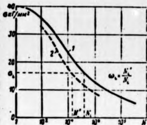
Fig. 7.16. Change of strength characteristics during tests with several levels of stresses. 1) curve, each point of which is determined at one level of repeated stresses; 2) strength curve determined by taking into account the action of stresses of several levels.
