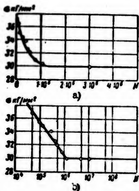
Fig. 7.3. Strength curves in different coordinates. a) linear coordinates; b) semilogarithmic coordinates.
