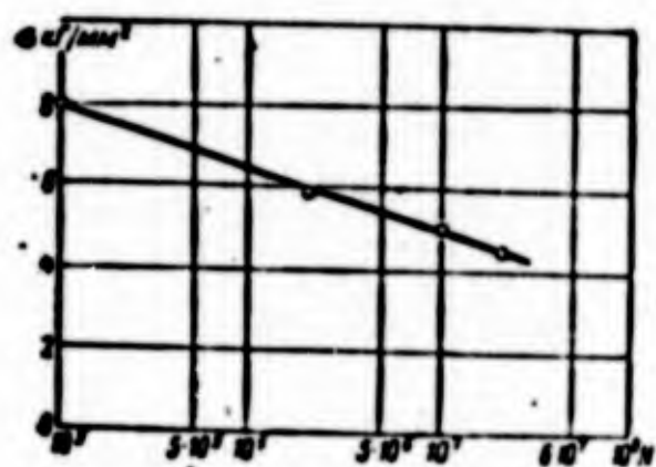
Fig. 7.4. Strength curve of an aluminum alloy.
