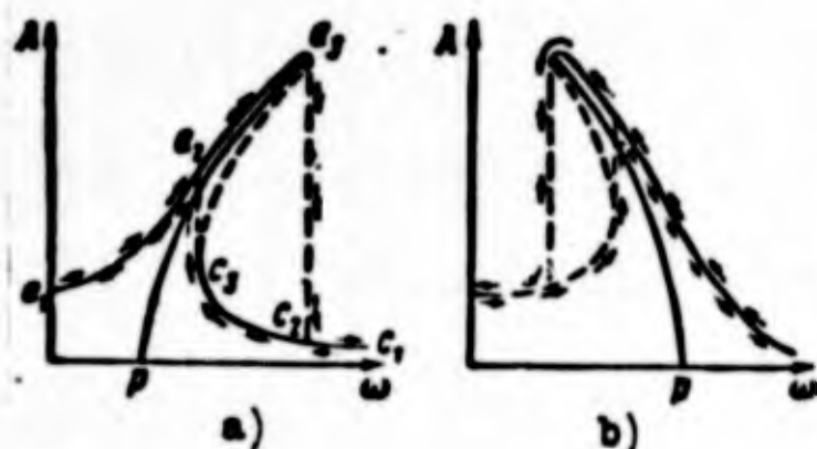
Fig. 3.12. Resonance curves of nonlinear systems. a) for system with gradually increasing rigidity (Fig. 3.11d — "rigid" system); b) for system with gradually decreasing rigidity (Fig. 3.11e — "soft" system).
