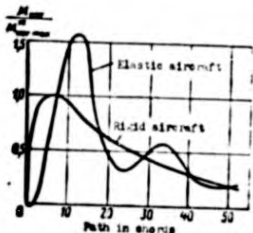
Fig. 4.18. Graph of bend-wind ( M_{\text{bend.max}}^r is the maximum magnitude of bending moment of the wing of a rigid aircraft).
