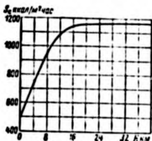
Fig. 8.7. Change of solar heat flow according to altitude H .
