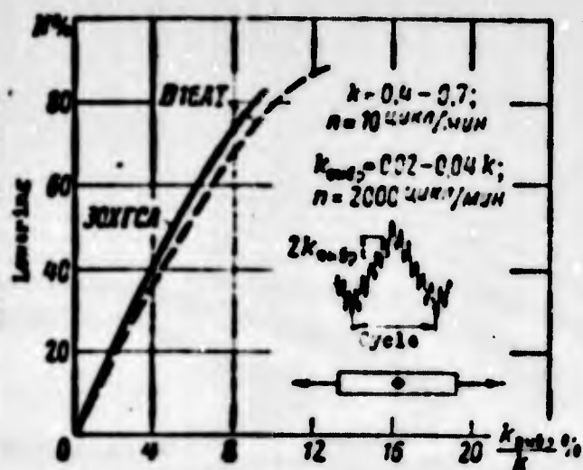
Fig. 7.19. Influence of vibrations on strength during repeated loads.
