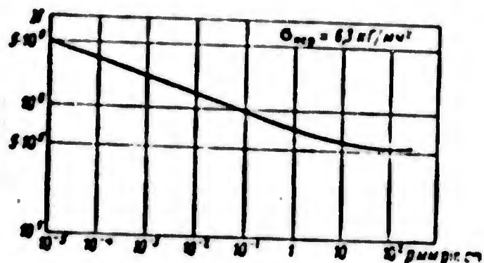
Fig. 7.9. Influence of an air medium on the endurance of an aluminum alloy.
