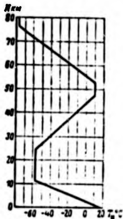
Fig. 8.3. Change of air temperature with altitude.
