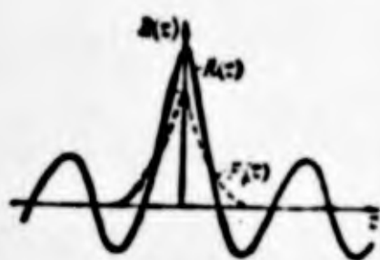
Fig. 4.12. Form of correlation function of a process having a periodic component. R_1(\tau) -correlation function corresponding to the random component of function x(t) .
