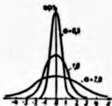
Fig. 4.6. Curves of normal distribution with different values of \sigma .
