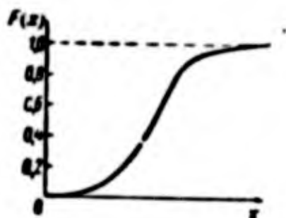
Fig. 4.2. Curve of integral probability distribution.
