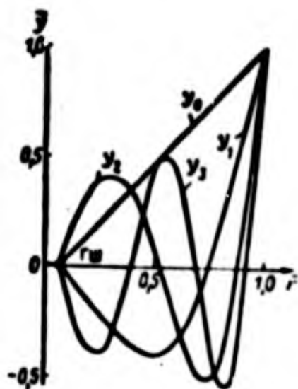
Fig. 9.3. Forms of oscillations for an absolutely rigid blade ( y_0 ) and for the first three tones of a real elastic blade ( y_1 , y_2 , y_3 ).
