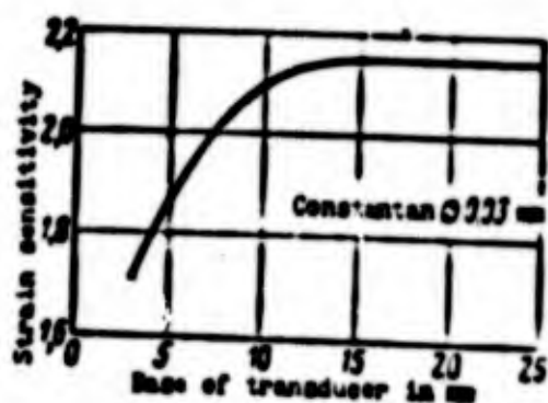
Fig. 10.2. Graph of the dependence of strain sensitivity of a wire gauge on its base.
