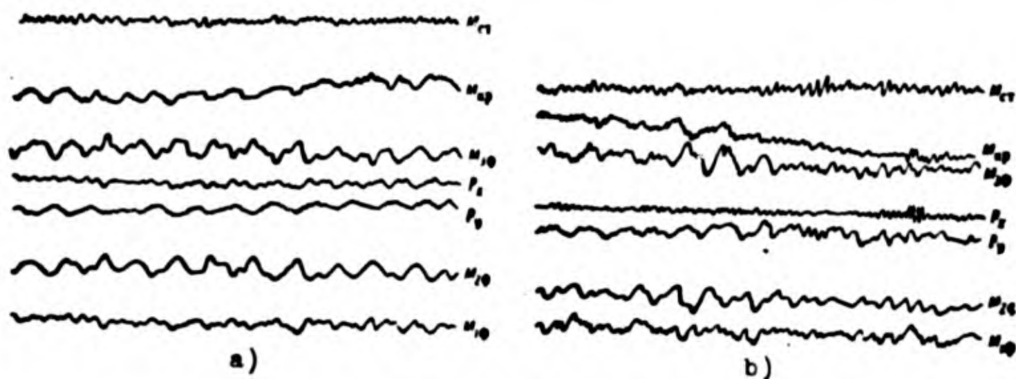
Fig. 2.42. Character of loads during takeoff run a) and landing run b) of an aircraft. M_{sta} , M_{wl} and M_{fus} — bending moments of stabilizer, wing, and fuselage, respectively; 1, 2, 3 — numbers of sections, P_x and P_y are loadson main strut of landing gear.
