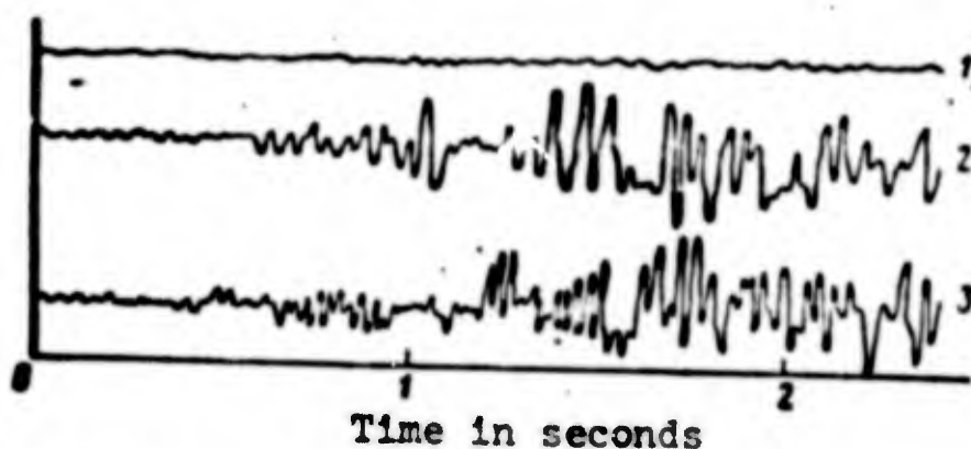
Fig. 5.12. Recording of oscillations during buffeting of the empennage on an aircraft. 1) wing; 2) afterbody; 3) elevator.
