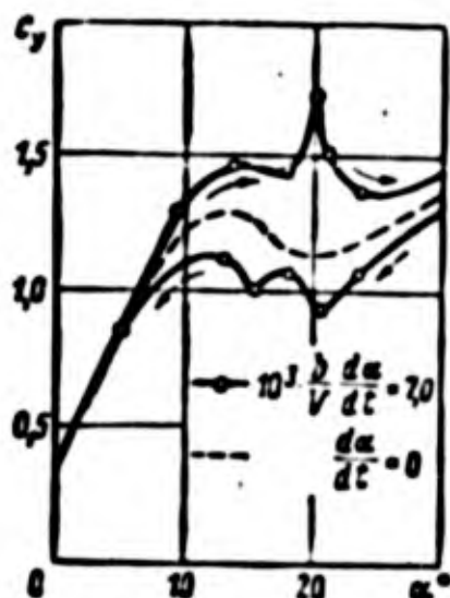
Fig. 1.22. Influence of speed of change of angle of attack on coefficient of maximum lift (profile of Klark UN, \lambda_{cr} = \infty , Re = 1.2 \cdot 10^5 ); direction of flow is constant, angle of attack of profile changes.
