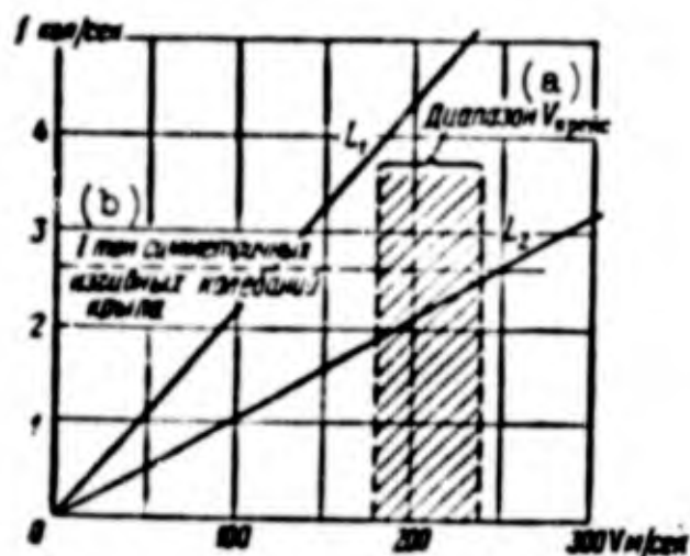
Fig. 4.19. Dependence of the frequency of influence of gust on the speed of flight. L_1 and L_2 — limiting values of length of gusts. KEY: (a) Range V_{cr} ; (b) 1st tone of symmetric bending oscillations of wing.
