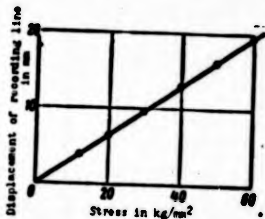
Fig. 10.5. Typical calibration graph of tensometric equipment.
