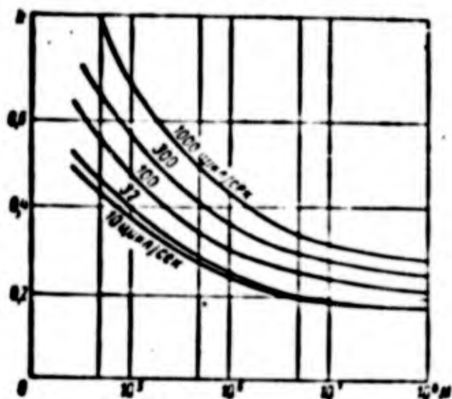
Fig. 7.12. Influence of loading frequency on fatigue strength of an aluminum alloy in an air medium.
