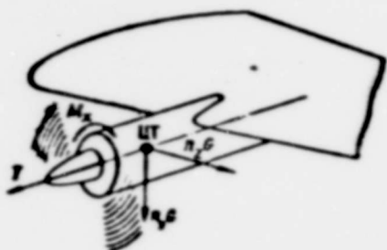
Fig. 2.43. Diagram of forces acting on turboprop motor.
