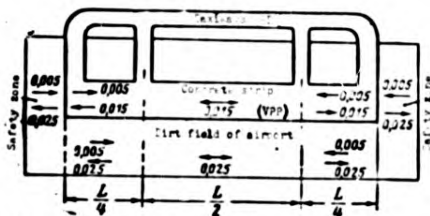
Fig. 2.33. Diagram of runway and taxiways of an airport, with indication of permissible slopes.
