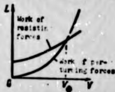
Fig. 6.4. Diagram of change of work L of excitation forces and resisting forces according to flow rate.
