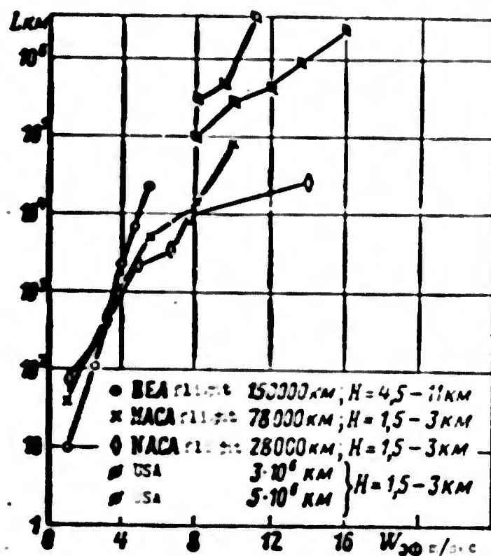
Fig. 1.26. Recurrence of W_{ef} on different altitudes ( L — path which aircraft must fly in order to encounter, on the average, one gust of assigned intensity).
