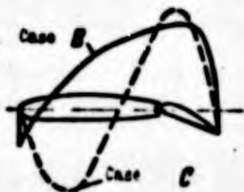
Fig. 2.6. Change of distribution of loads during deflection of aileron.
