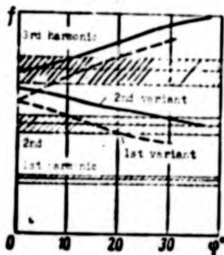
Fig. 3.26. Dependence of frequencies of natural oscillations of blade of steering propeller of helicopter on angle of installation. 1st variant — blade with bad frequency responses, 2nd variant — blade with improved frequency responses.
