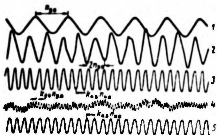
Fig. 9.10. Typical recording of vibrations and stresses in helicopter assemblies during horizontal flight. 1) flapping angle \beta of tail rotor blade; 2) bending moment of tail rotor blade in plane of rotation; 3) normal stresses in mounting rods of rotor reduction gear; 4) normal stresses in stringer of end beam; 5) vibrations in cockpit.
