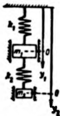
Fig. 3.15. System with two degrees of freedom.
