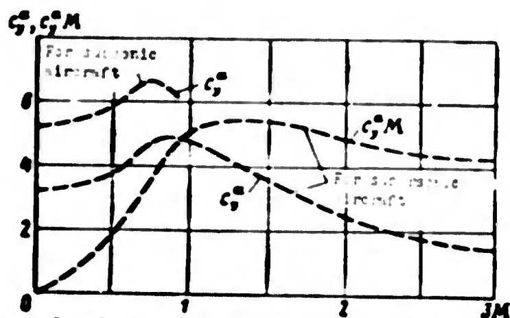
Fig. 1.20. Dependence of c_y and c_y M on Mach number.
