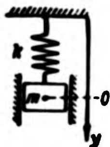
Fig. 3.1. Oscillatory system with one degree of freedom without damping.
