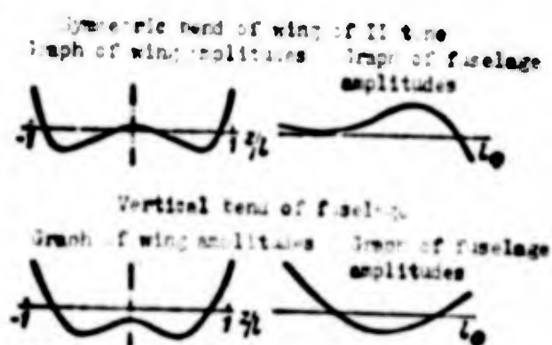
Fig. 3.21. Forms of oscillations of transport aircraft.
