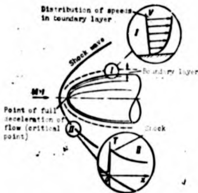
Fig. 8.2. Diagram of supersonic flow around a body and the character of change of temperature T in a shock.
