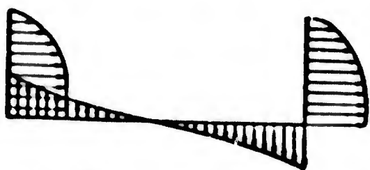
Fig. 2.27. Asymmetric loads on horizontal empennage with two-fin vertical empennage.
