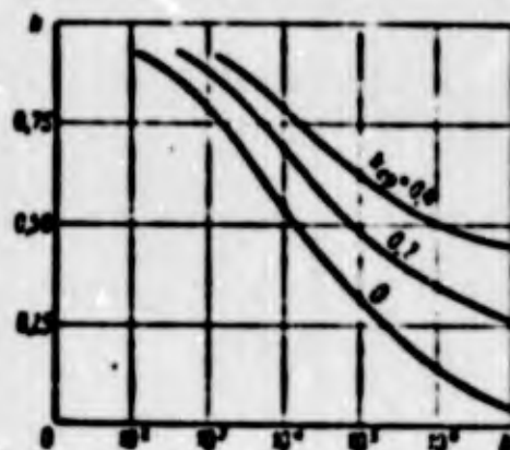
Fig. 7.23. Complete strength graph in coordinates k = f(N) when k_{av} = \text{const.}
