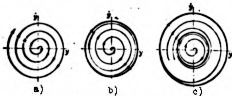
Fig. 6.11. Phase diagrams of oscillations. a) increasing oscillations; b) oscillations with a limit cycle; c) case of oscillations with several limit cycles.
