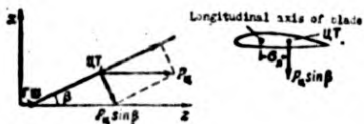
Fig. 9.12. Diagram of appearance of moment M_{fe.h.} with inaccurate transverse weight balancing of a blade.
