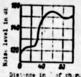
Fig. 5.19. Curve of noise level on a wing during stall.
