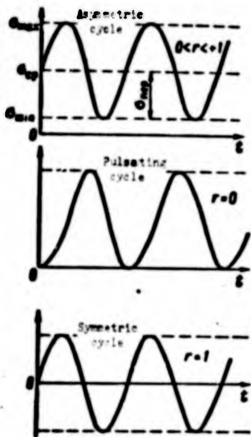
Fig. 7.2. Types of cycles of variable stresses.
