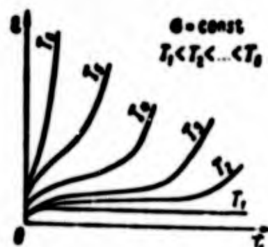
Fig. 8.20. Approximate change of the characteristics of creep with the increase of temperature.
