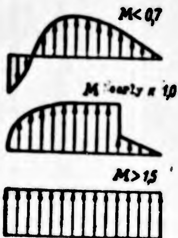
Fig. 2.5. Distribution of load along the chord at small angle of attack.
