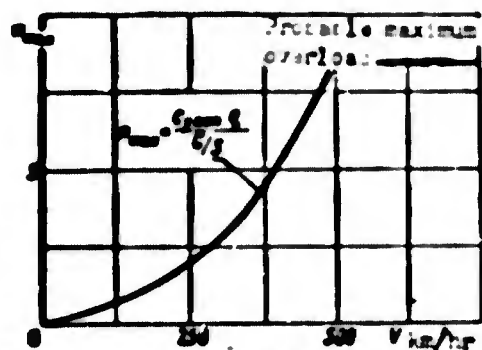
Fig. 1.12. Dependence of maximum overload on speed of flight for maneuvering aircraft.
