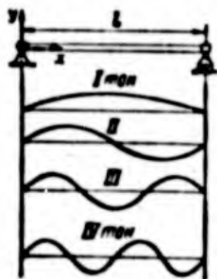
Fig. 3.23. Forms of oscillations of a homogeneous beam with hinged supported ends.
