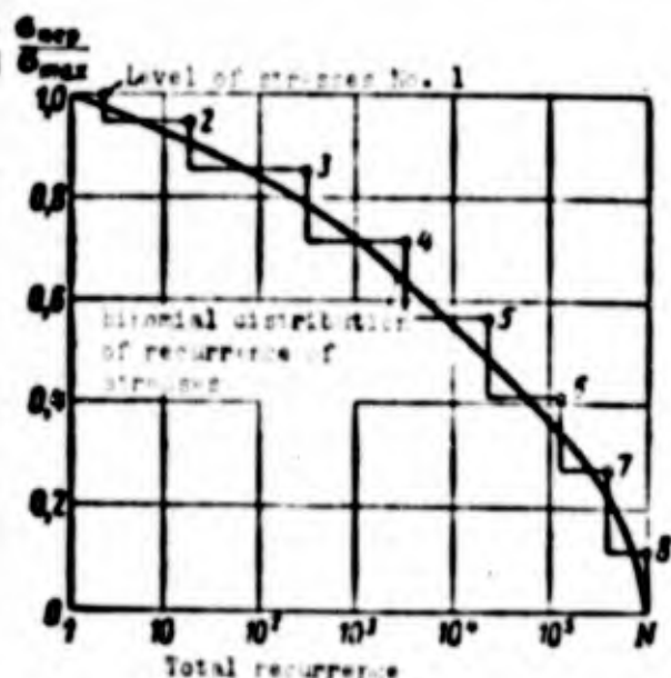
Fig. 7.39. Continuous and gradual spectrum of recurrence of stresses.
