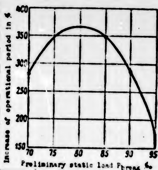
Fig. 7.21. Influence of preliminary load on the strength of a structure.
