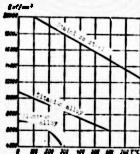
Fig. 8.17. Change of the first elastic modulus E of structural alloys, depending upon temperature.
