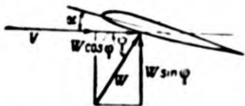
Fig. 1.18. Diagram of vectors of velocities during action of gust at angle \varphi .
