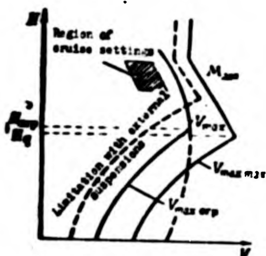
Fig. 1.4. Approximate character of limitation of speed of flight of aircraft with jet engine during subsonic speeds of flight.
