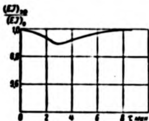
Fig. 8.28. Change of effective flexural rigidity of a double-wedge wing during heating.
