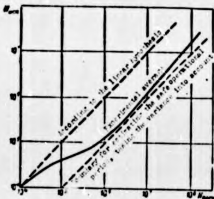
Fig. 7.17. Strength of samples made from aluminum alloy 2024 at a variable loading level.
