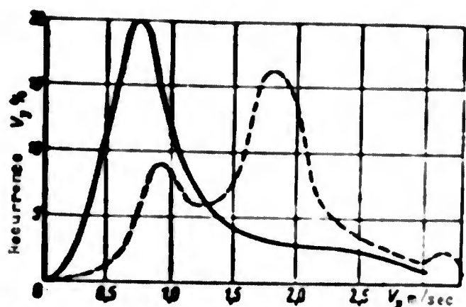
Fig. 2.32. Recurrence of V_y during landing in simple and adverse weather conditions. — landing in simple weather conditions, - - - landing in adverse weather conditions.
