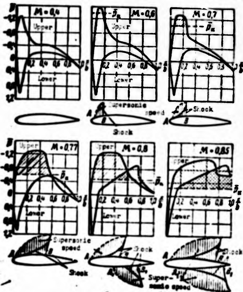
Fig. 2.4. Distribution of pressure on lower and upper surfaces of wing at different Mach numbers.
