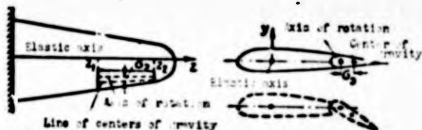
Fig. 6.5. Diagram of wing with aileron.
