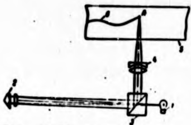
Fig. 10.23. Diagram of measurement of general deformations by the optical method.
