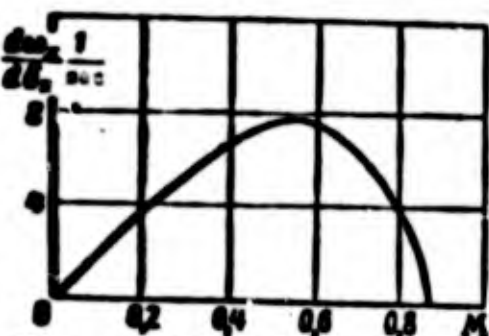
Fig. 2.21. Change in effectiveness of ailerons with respect to Mach number.
