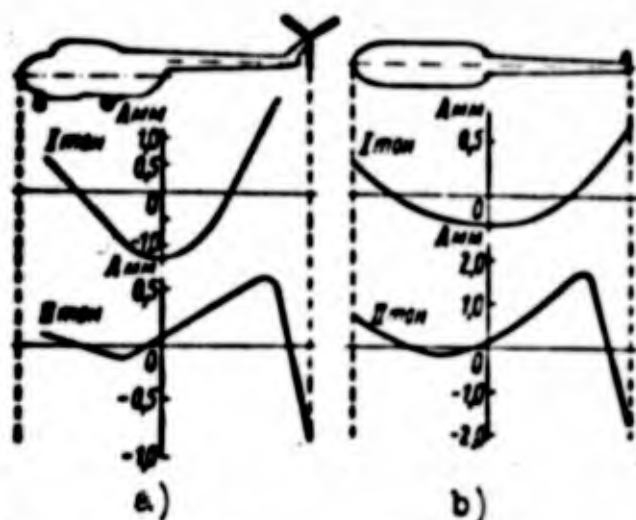
Fig. 3.22. Forms of oscillations of a single-propeller helicopter. a) vertical bend of fuselage and tail beam; b) horizontal bend of fuselage and tail beam.
