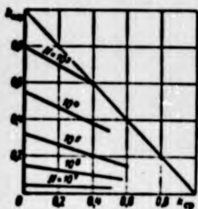
Fig. 7.22. Complete strength graph in coordinates k_{var} = f(k_{av}) when N = \text{const.}
