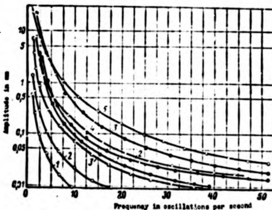
Fig. 10.39. Graphs for estimating oscillations from conditions of physiologic sensations. 0 — 0 — based on the results of generalization of test data of helicopters and aircraft: 0-1 — not noticeable, 1-2 — hardly noticeable, 2-3 — noticeable, 3-4 — slightly unpleasant, 4-5 — unpleasant to a limit, 5 — very unpleasant, ●-● — based on the results of laboratory and flying tests: 1) recommended limit; 2) uncomfortable; 3) very uncomfortable.
