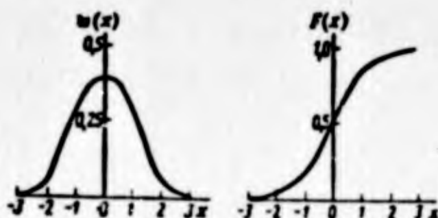
Fig. 4.5. Graphs of functions w(x) and F(x) for normal distribution.
