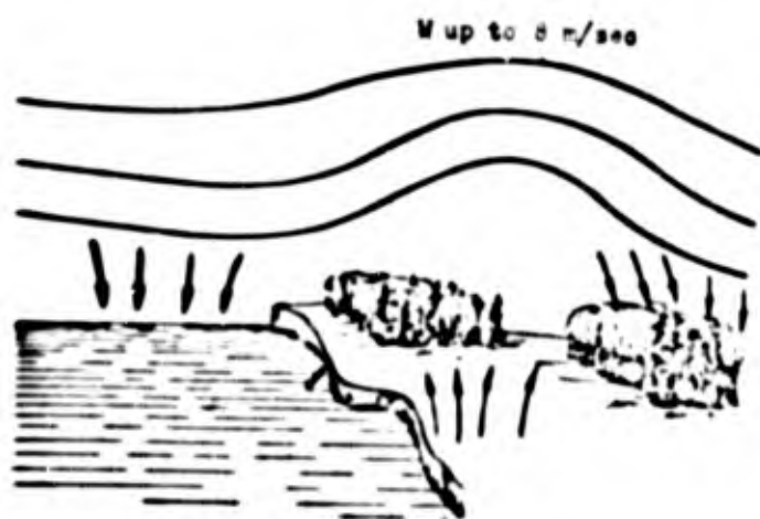
Fig. 1.13. Diagram of formation of thermal flows.
