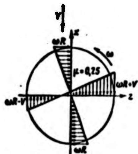
Fig. 9.2. Field of speeds of airflow on the blades of a moving rotor during flight at horizontal speed.
