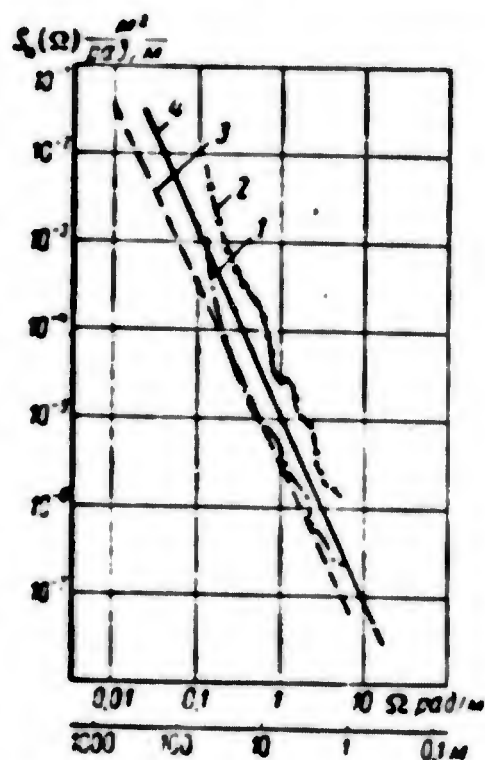
Fig. 4.29. Graphs of the spectral density of runway roughness. 1) runway; 2) taxiway; 3) permissible roughness of new runway; 4) permissible roughness after prolonged use.
