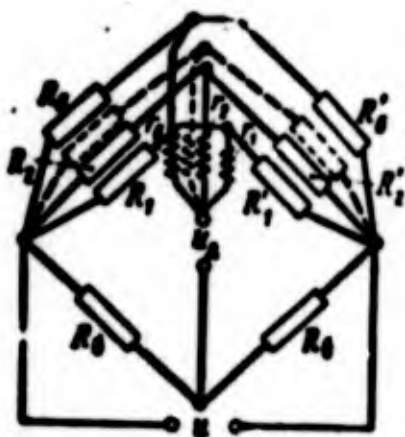
Fig. 10.33. Simplified diagram of parallel connection of strain gauges.
