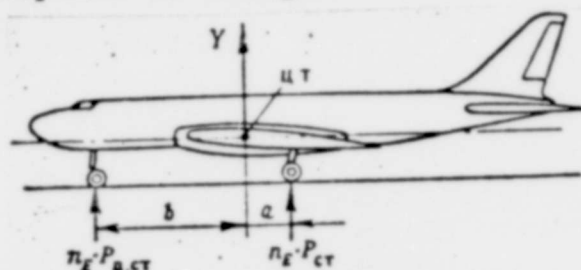
Fig. 2.39. Diagram of forces acting on aircraft during three-point landing.
