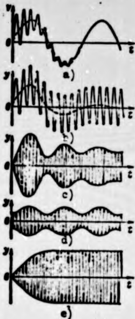
Fig. 3.4. Process of establishment of forced oscillations under the action of a disturbing force. a) \omega \ll p , b) \omega \gg p , c) \omega \sim p , d) \omega_1 \sim \omega_2 , e) \omega = p .
