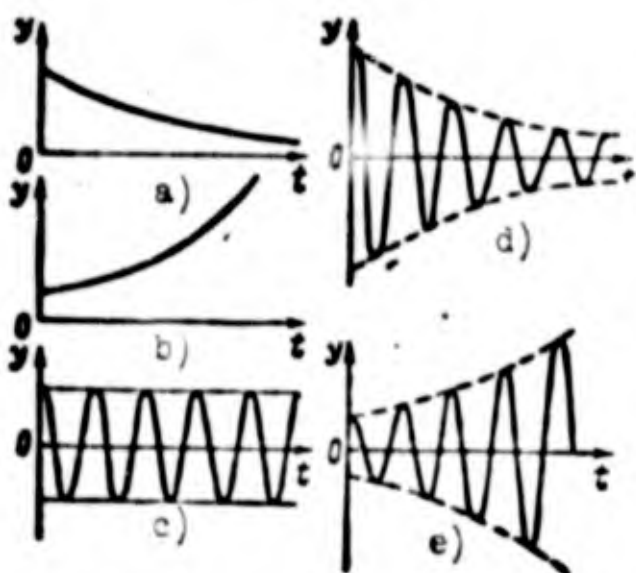
Fig. 6.13. Motion of a system at different values of damping decrement \delta and frequency p .
