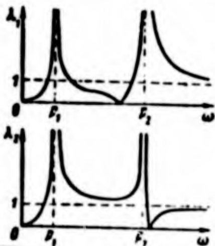
Fig. 3.18. Change of coefficients of dynamics \lambda_1 and \lambda_2 depending upon frequency during assigned motion of point of bracing.
