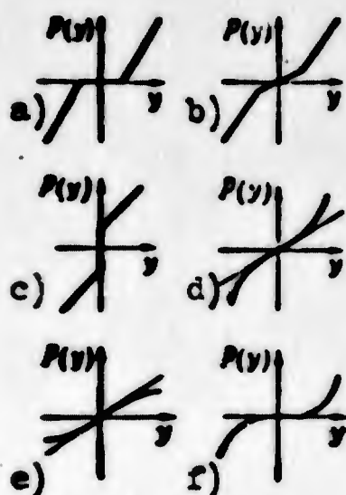
Fig. 3.11. Examples of nonlinear elastic characteristics.
