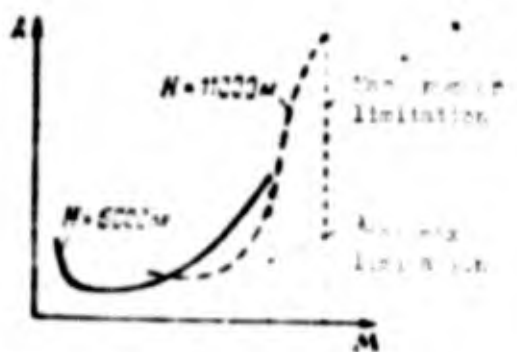
Fig. 5.10. Dependence of aerodynamic oscillations on Mach number for two altitudes of flight.
