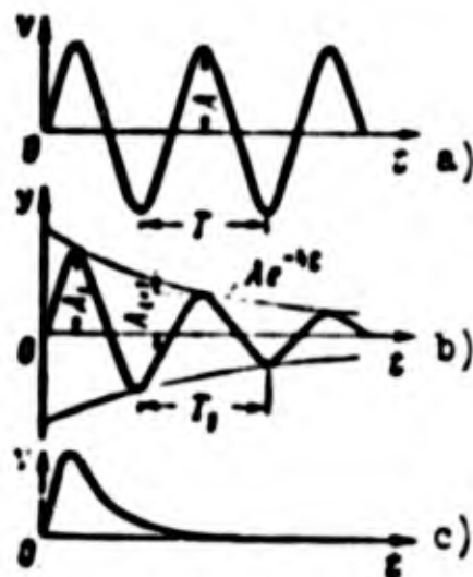
Fig. 3.2. Free oscillations in a system with different damping. a) h = 0 ; b) h < p ; c) h > p .
