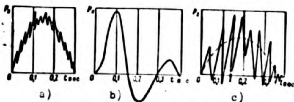
Fig. 2.34. Character of change of components of load on strut of landing gear during landing (first impact). a, b, c — vertical, frontal, and lateral components, respectively.
