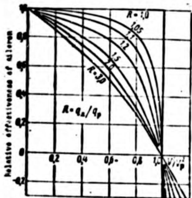
Fig. 2.20. Influence of critical speed of divergence on effectiveness of aileron.
