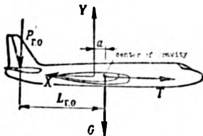
Fig. 1.6. Forces acting on an aircraft in horizontal flight.
