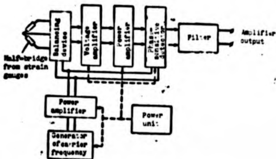
Fig. 10.4. Block diagram of tensometric equipment with amplifier.
