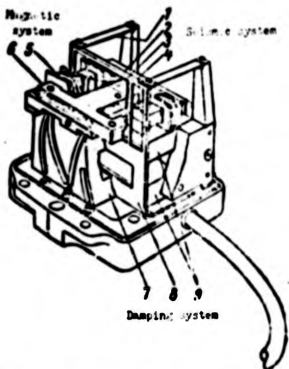
Fig. 10.10. Electromagnetic accelerometric transducer.
