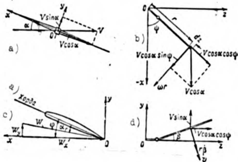
Fig. 9.5. Components of flow rate on blade. a) breakdown of flow rate V into components along rotor axes; b) flow rate on blade element in plane of rotation; c) component of resultant speed W on blade element during forward flight ( \alpha_r is the angle of attack of blade element); d) flow rate on blade element in flapping plane.
