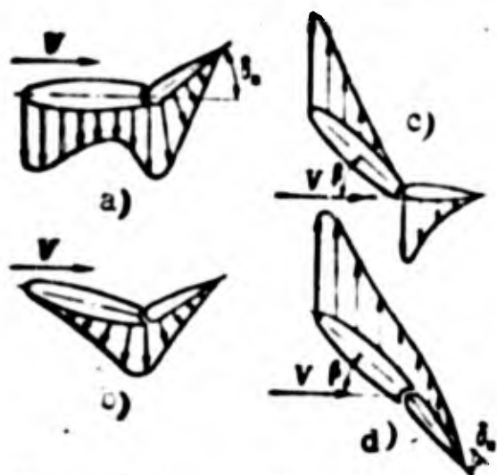
Fig. 2.25. Loads on vertical empennage in different phases of maneuver. a) beginning of maneuver, sharp rudder deflection, b) flight with small angle of sideslip; c) flight with large angle of sideslip; d) termination of maneuver, deflection of control surface for return to conditions of zero sideslip.
