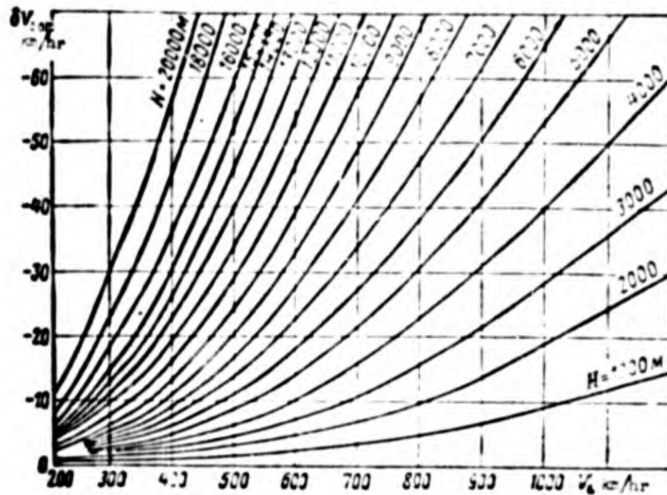
Fig. 1.2. Graph for determinating correction for compressibility.
