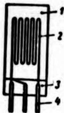
Fig. 10.13. Diagram of a film resistance transducer for measurement of temperatures. 1) base of transducer; 2) copper wire; 3) base for attaching connecting wires; 4) connecting wire.
