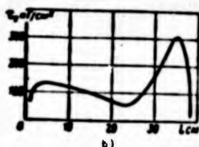
Fig. 8.14. Normal (a) and tangential (b) thermal stresses in the wall of a spar during non-stationary heating.
