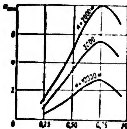
Fig. 1.10. Dependence of n_{\text{per}} on Mach number.
