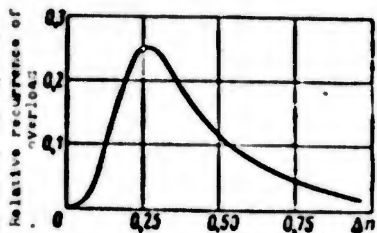
Fig. 7.28. Recurrence of overloads during the first landing shocks.
