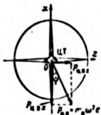
Fig. 9.13. Diagram of formation of components of unbalanced centrifugal force P_{\text{cen. rot}} with unbalance of mass forces on a rotor.
