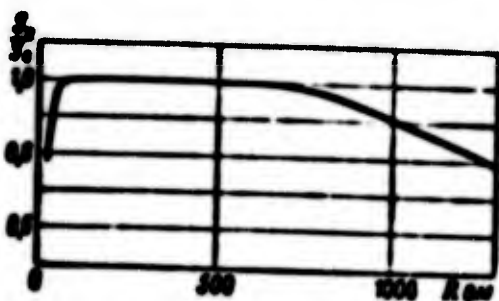
Fig. 10.28. Change of sensitivity of equipment with amplifier (diagram I) depending upon resistance of transducer R . S_0 is sensitivity at nominal resistance of transducers (120 ohms).
