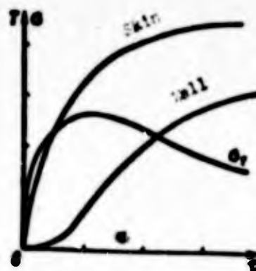
Fig. 8.13. Character of thermal stresses appearing in a wall during heating.
