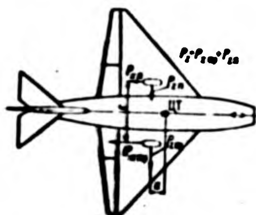
Fig. 2.47. Lateral loads on fuselage during landing.
