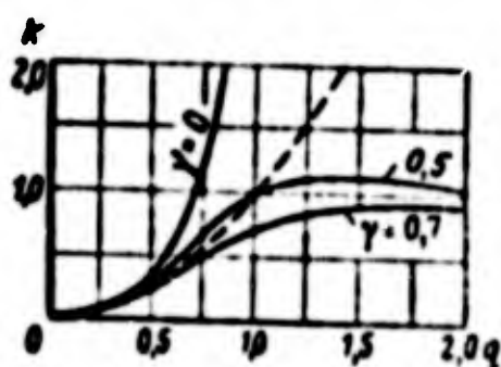
Fig. 10.7. Frequency-response curves of an accelerometer with various damping (dotted curve is a parabola).
