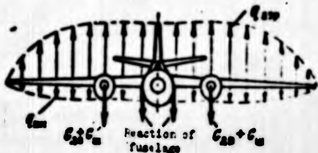
Fig. 2.8. Diagram of loads on wing ( Q_{mot} - weight of motor, Q_{l.g} - weight of landing gear). Q_{aero} Q_{in} - linear aerodynamic and inertial loads.
