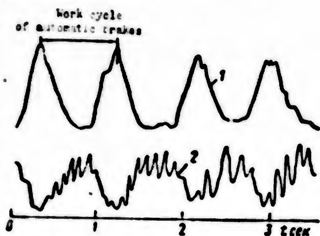
Fig. 7.29. Character of loads during braking in a landing run. 1) force in brake rod of bogie; 2) force in landing gear strut.
