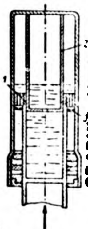
Fig. 2.36. Diagram of shock absorber of landing gear. 1) piston; 2) plunger; 3) check valve.
