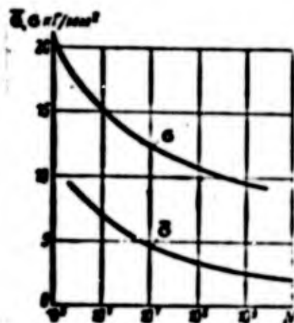
Fig. 7.36. Strength of an aluminum alloy during random alternation of stresses.
