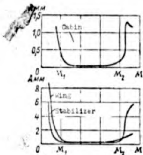
Fig. 5.5. Graphs of aerodynamic oscillations of a passenger aircraft.
