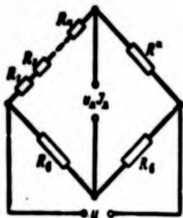
Fig. 10.31. Series connection of strain gauges.
