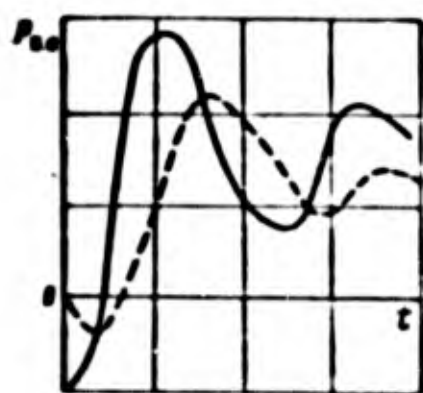
Fig. 2.24. Character of change of loads on vertical empennage during rudder deflection. — sharp application of force to pedals ( P_0 = \text{const} ), - - - smooth application of force to pedals P = P_0 (1 - e^{-2t}) .
