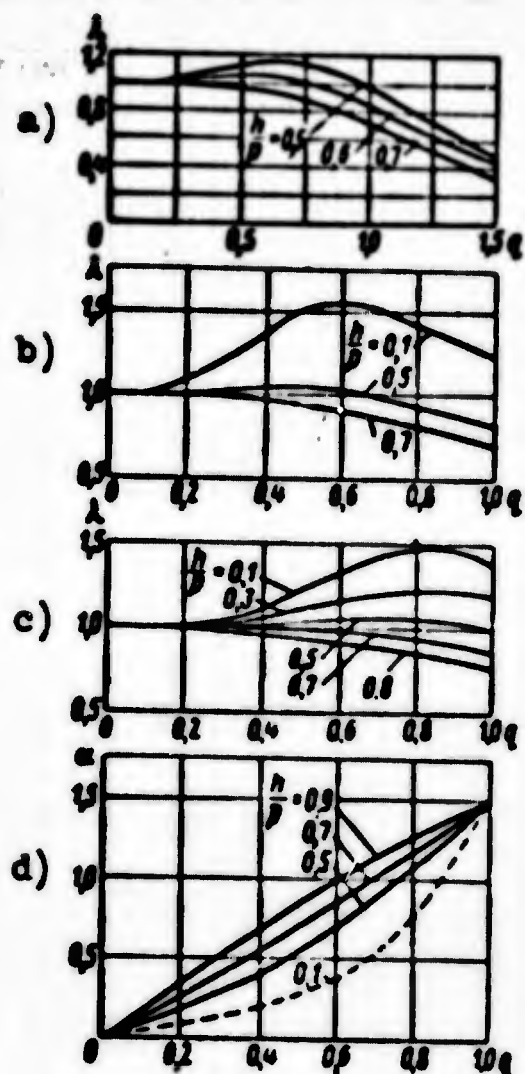
Fig. 3.9. Graphs of dynamics coefficient for forces of small duration. a) P(t) = P_0 \sin \omega t — repeated force, b) P(t) = P_0 \sin \omega t — single force, c) P(t) = \frac{P_0}{2} (1 - \cos \omega t) — single force, d) phase response for force P(t) = \frac{P_0}{2} (1 - \cos \omega t) .
