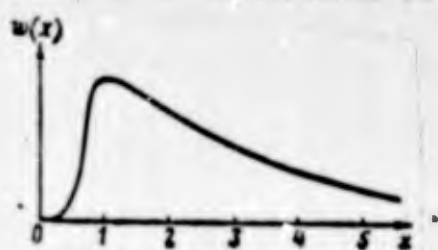
Fig. 4.7. Curve of logarithmically normal distribution.
