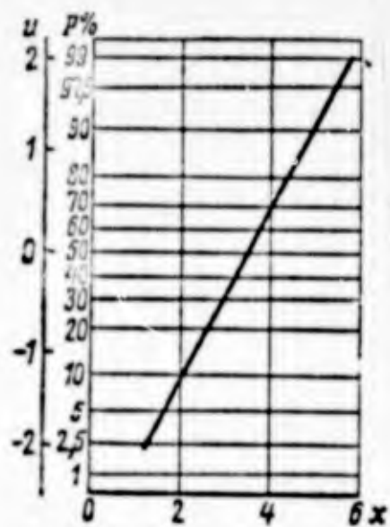
Fig. 4.8. Curve of normal distribution in probability scale.
