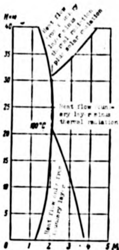
Fig. 8.9. Regions of conditions of flight and heat flow which are predominant in the common heat balance.
