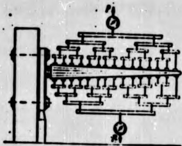
Fig. 10.16. Diagram of column tests.
