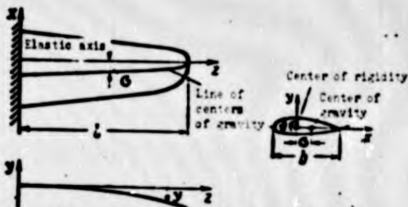
Fig. 6.1. Diagram of a wing for the calculation of flexure-torsion flutter ("cantilever diagram").
