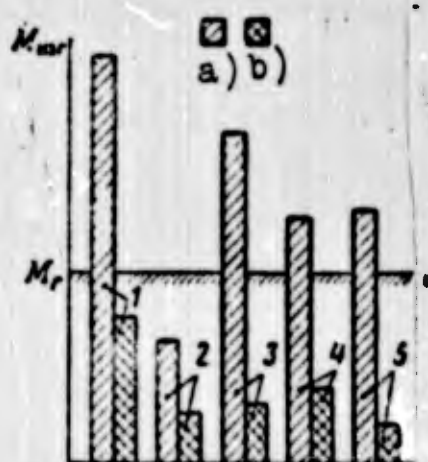
Fig. 9.20. Loading diagram of blades of two tail rotors. a) with unsatisfactory dynamic response characteristic (see Fig. 3.26, 1st variant); b) with improved dynamic response characteristic (see Fig. 3.26, 2nd variant).
