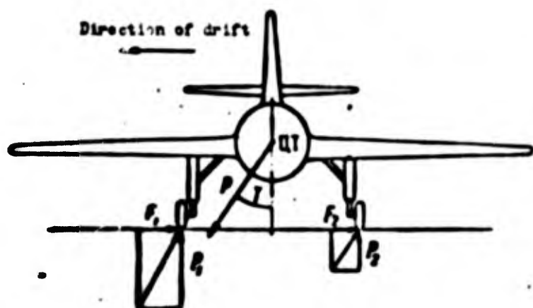
Fig. 2.40. Diagram of forces effective during landing with drift.
