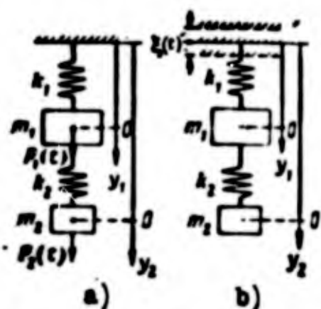
Fig. 3.16. Excitation of oscillations in a system with two degrees of freedom. a) assigned power disturbance; b) assigned motion of point of bracing.
