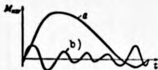
Fig. 10.43. Example of a recording of wing bending moment of an aircraft. a) when executing a zoom; b) during landing run.
