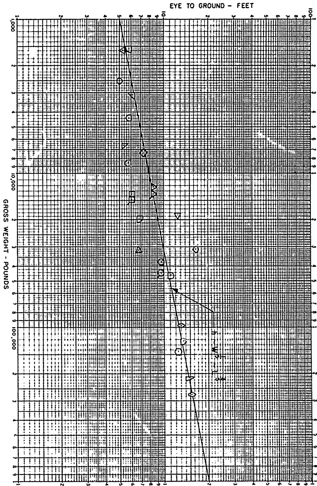
Figure 20 - Distance from Pilot's Eye to Ground (Vehicle on Ground)
