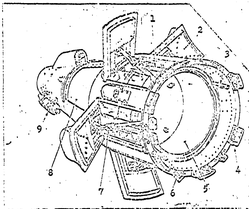
Fig. 13. Recoverable Nose Cone of Soviet Research Rocket
