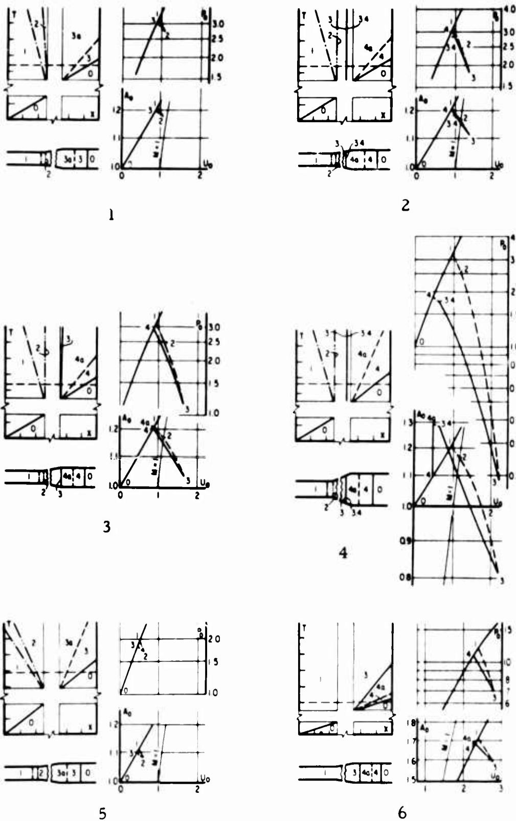
Fig. 21. Shock Interactions with Area Divergences
