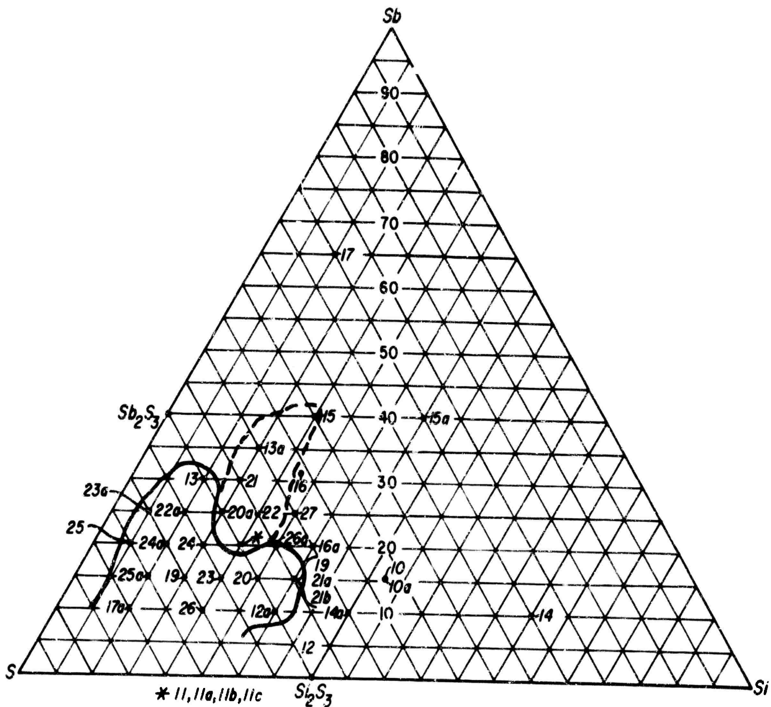
Figure 3 Si-Sb-S Glass Composition Diagram
