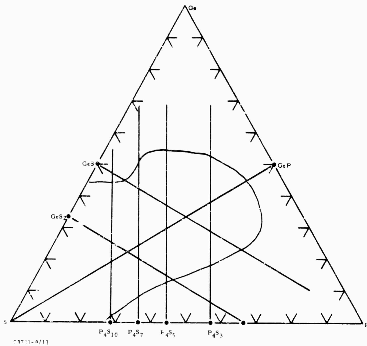
Figure 39 The Ge-P-S System
