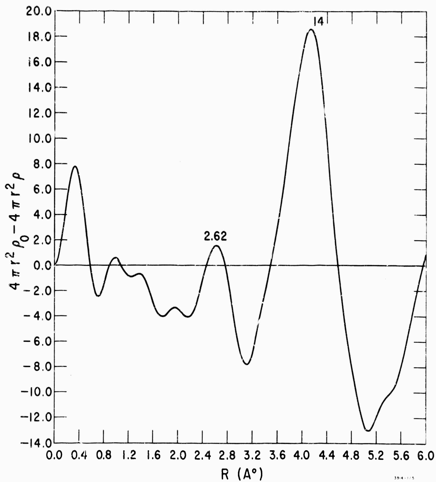
Figure 51 Radial Distribution Function of SiTe 4 Glass
