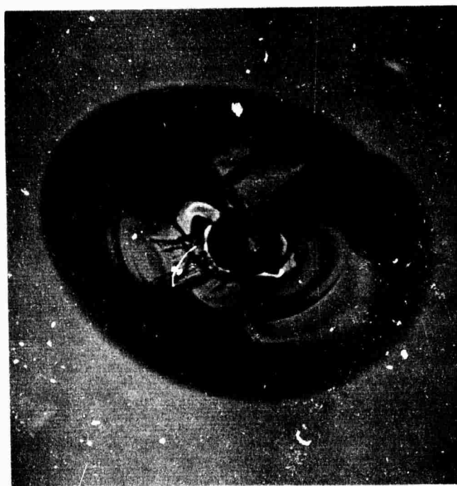
Fig. 2.2 10 to 12 micron inclusion 1,800 J/cm 2 28X
