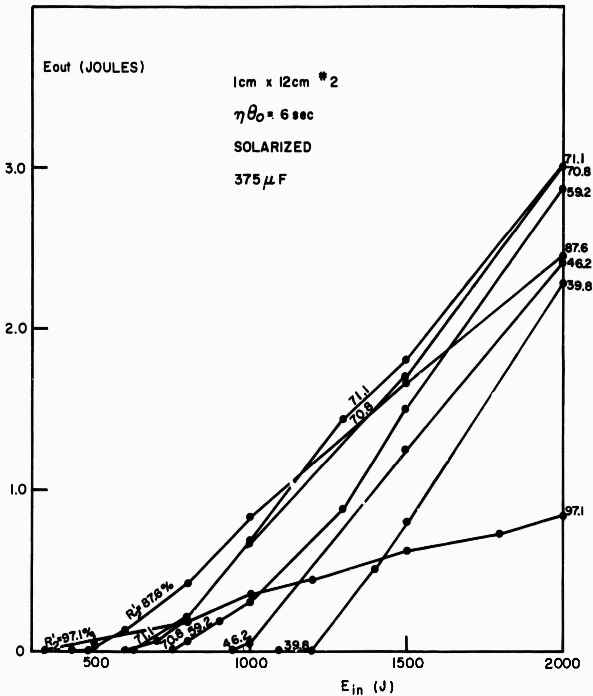
Fig.3.11 Output energy versus input electrical energy for given values of output mirror effective reflectance. Capacitance 375 \mu\text{F} . Laser sample 1 cm x 12 cm #2. R_1 = 98.7\% .
