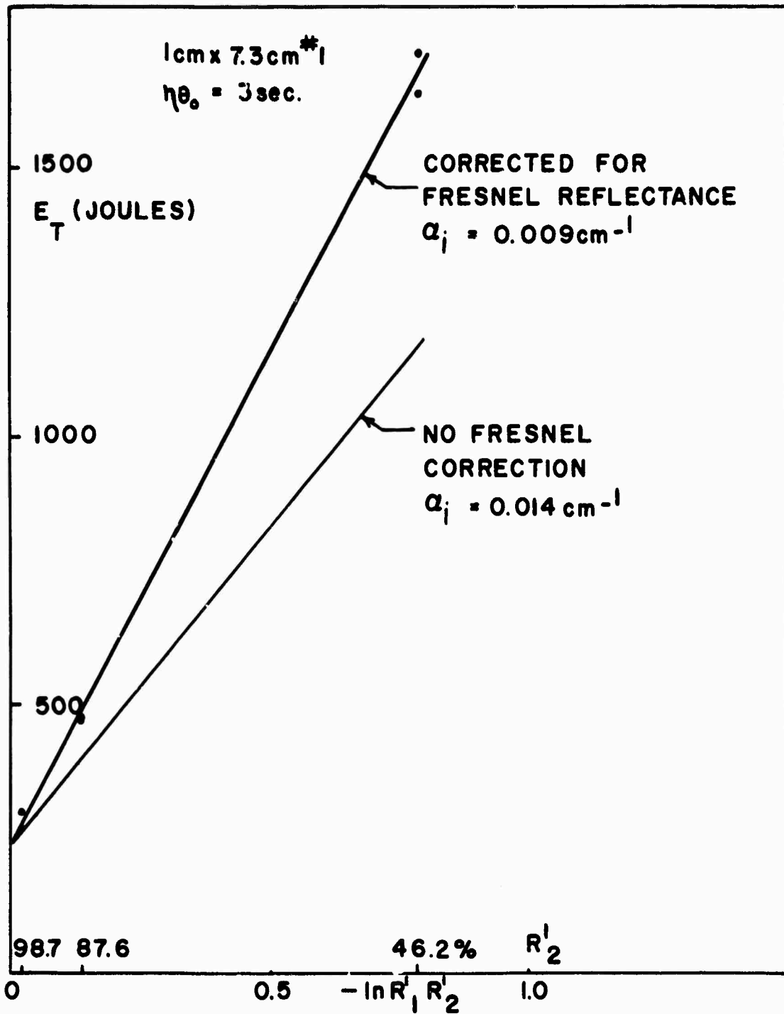
Fig. 3.9 Threshold versus -\ln R_1^i R_2^i for 1 cm x 7.2 cm #1 Code 0580 laser rod.
