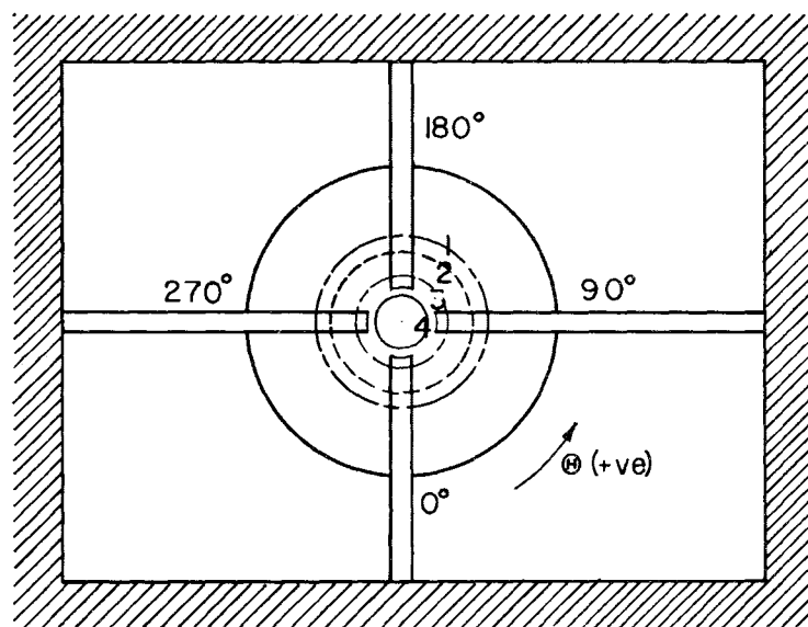
Fig. 15 Radial- and Circumferential-Probe Locations and Coordinate System
