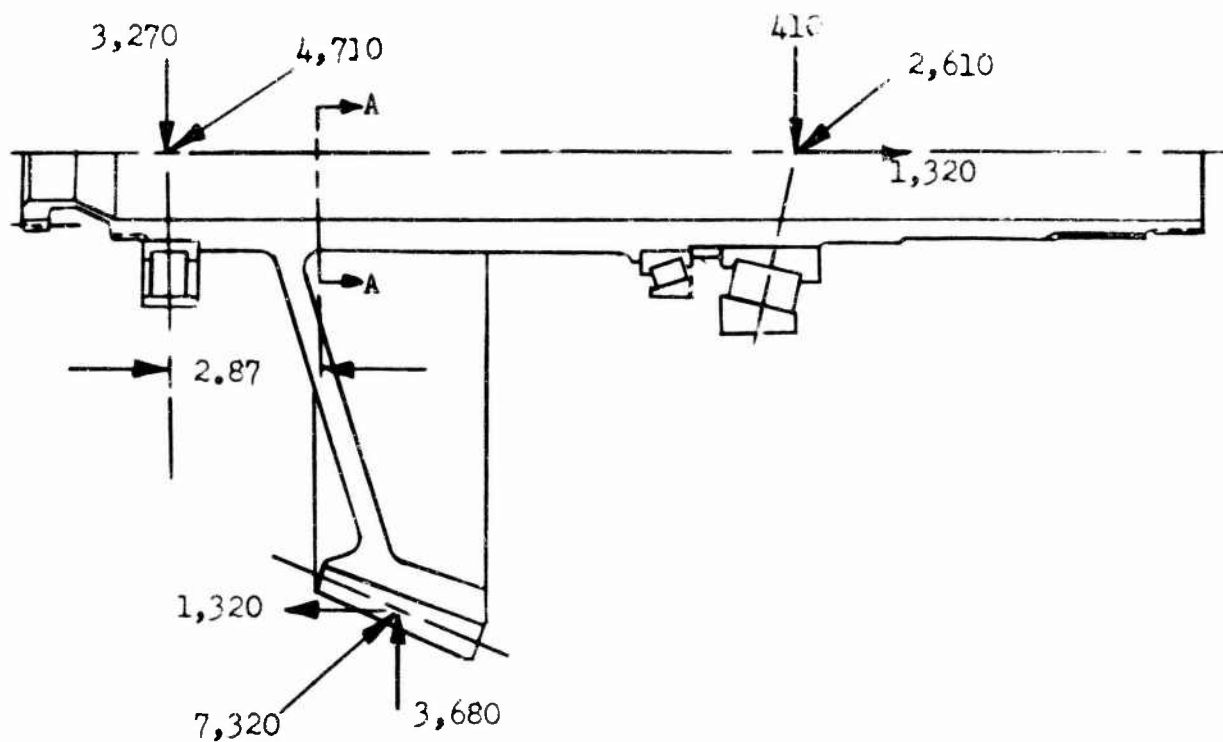
Figure 18. Output Gear Shaft, Engine Reduction Gearbox.
