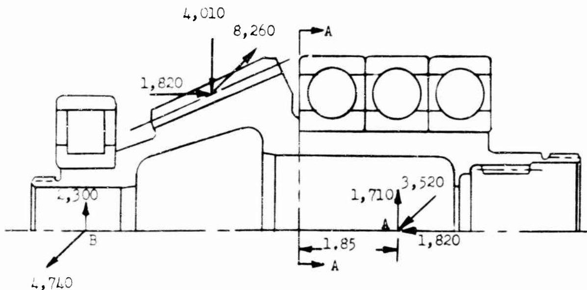
Figure 3. High-Speed-Input Bevel.
