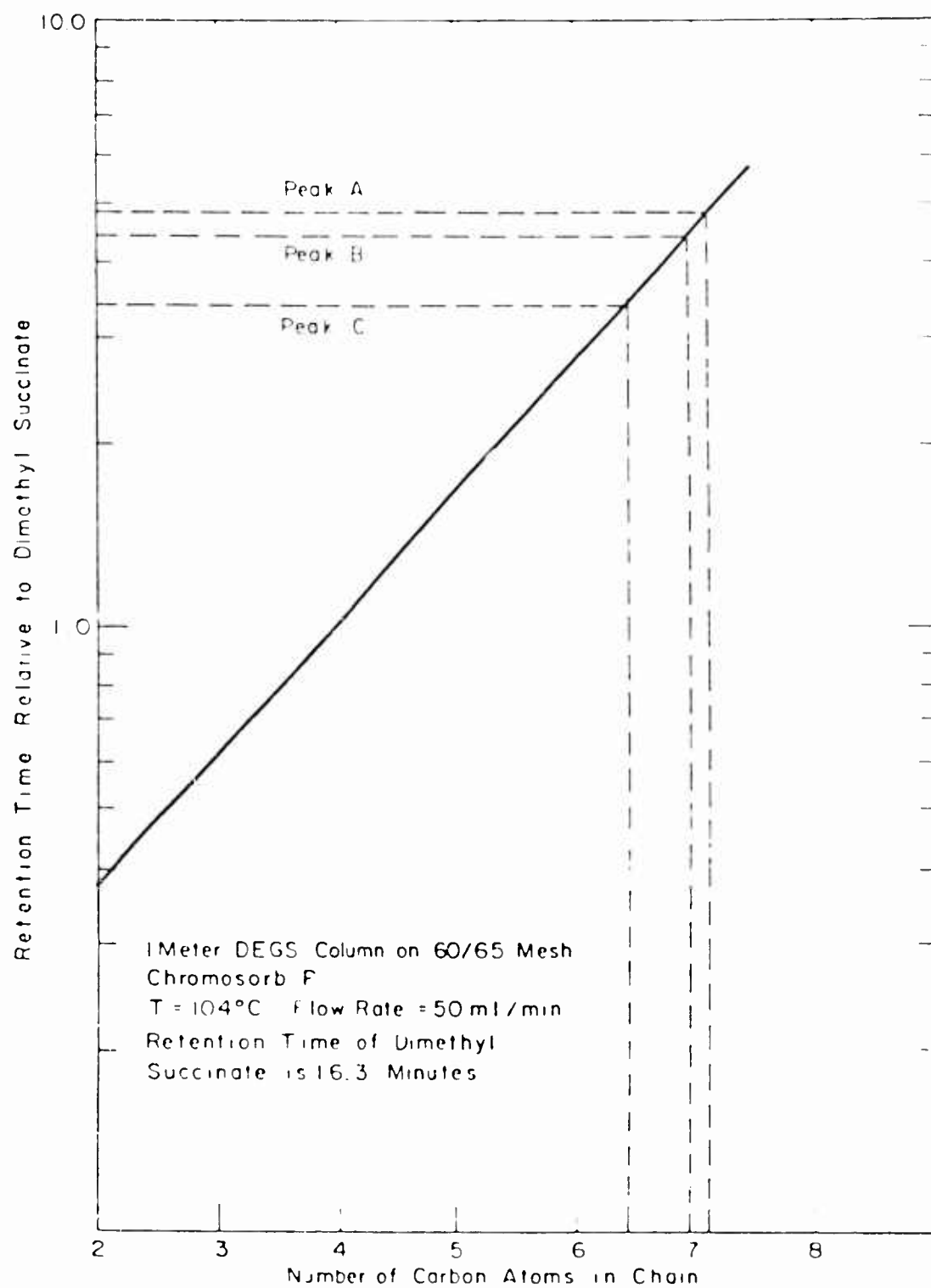
FIG. 6. Comparison of Retention Times of Certain Urinary Components with Known Dicarboxylic Esters
