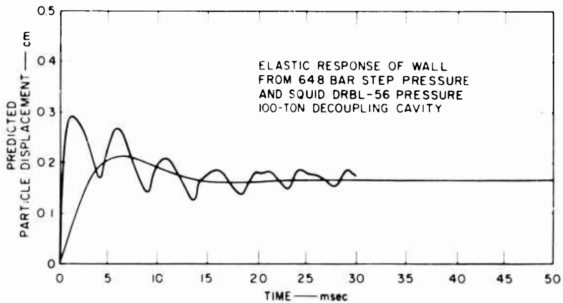
FIG. 3 DISPLACEMENT VERSUS TIME, SQUID RUN DRBL-56
