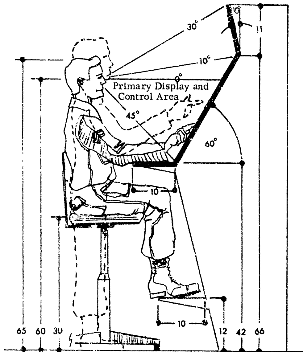
Fig. 33. Console Dimensions for Sit-Stand Operators
