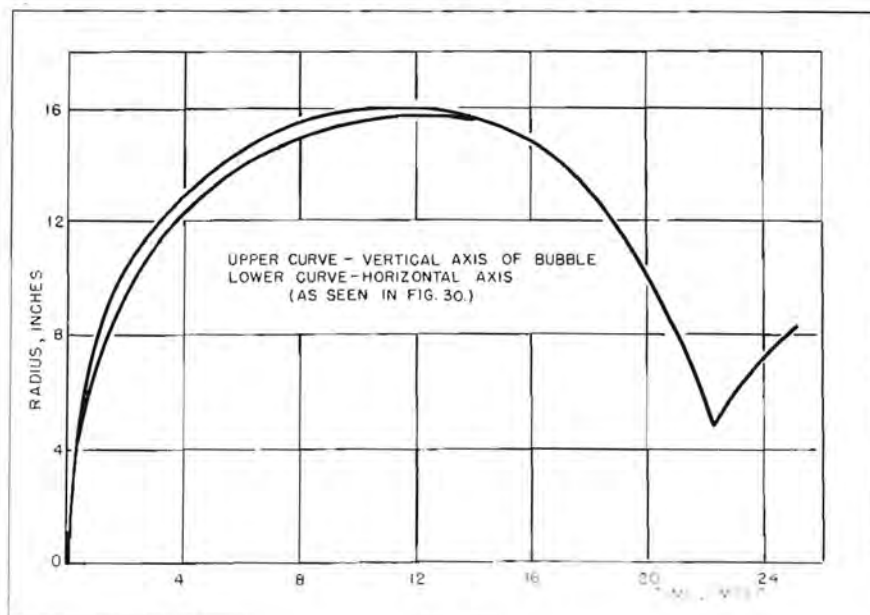
Fig. 31. Bubble radius vs. time.
