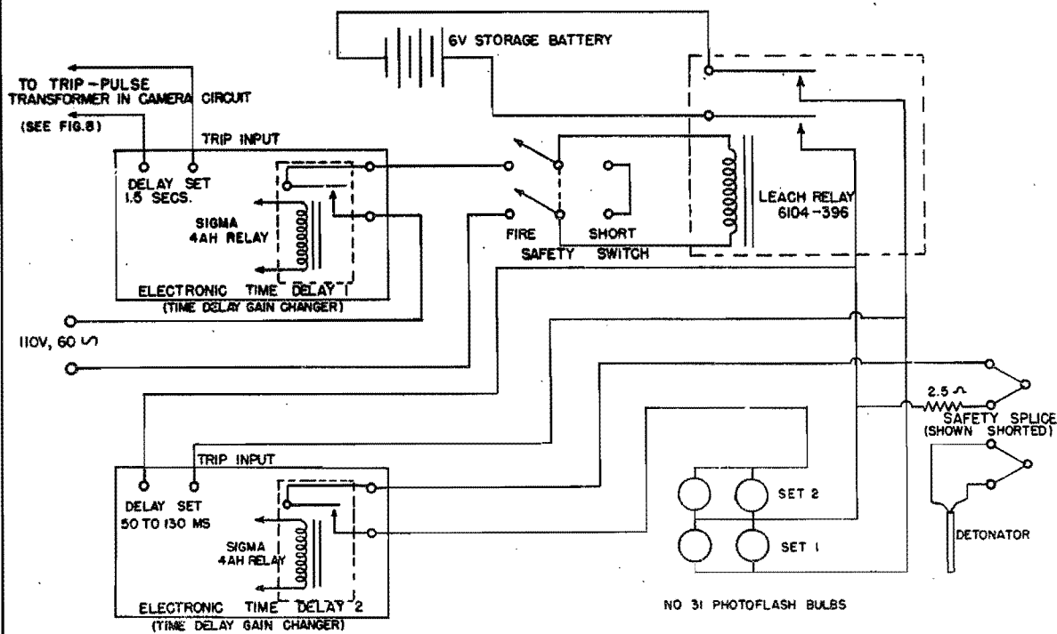
FIG. 9 AUTOMATIC FIRING SEQUENCE FOR FASTAX CAMERA UERL WOODS HOLE, MASS.
