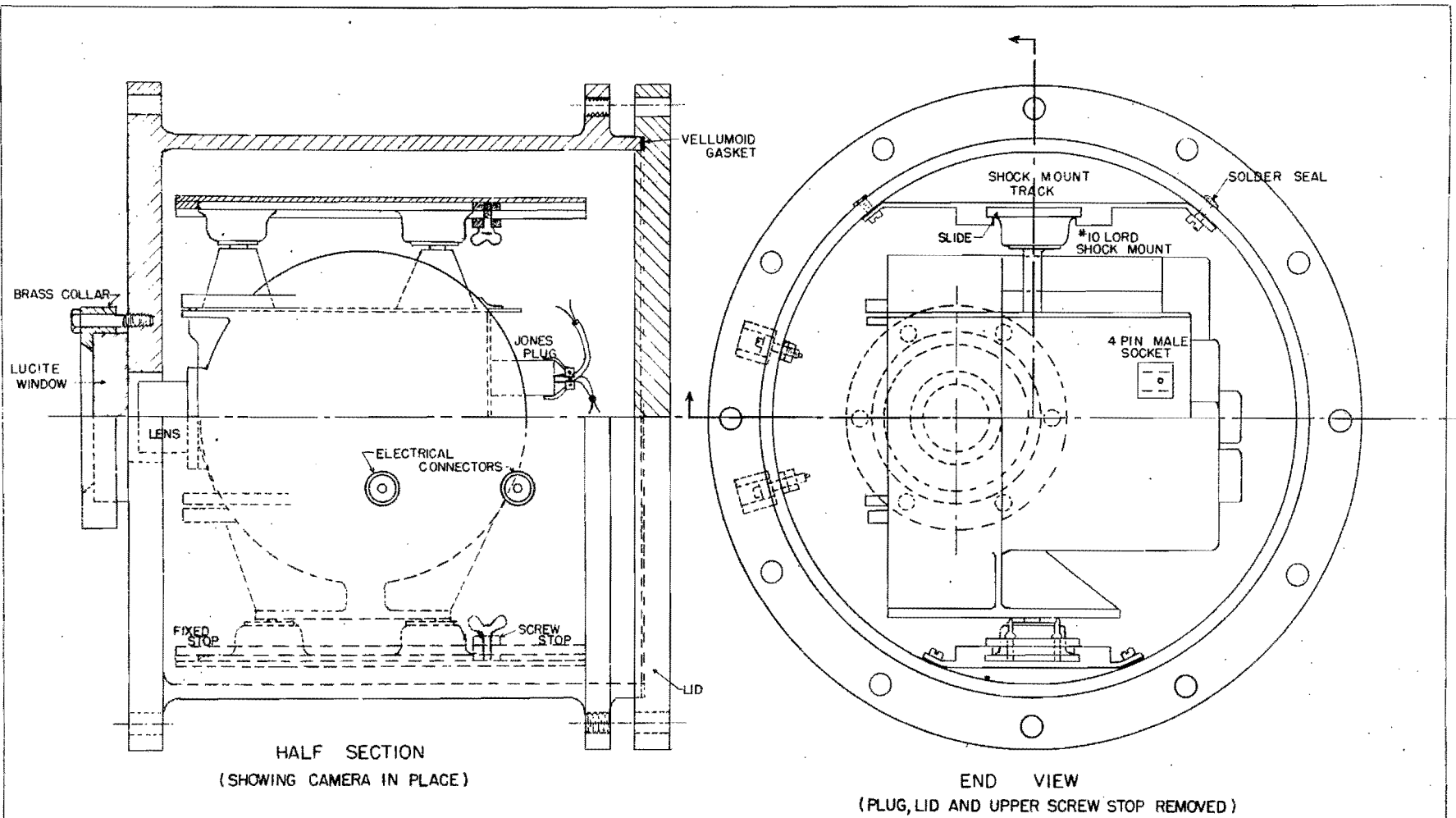
FIG. 5 EXPLOSION PROOF CASE FOR FASTAX CAMERA UERL WOODS HOLE, MASS.
